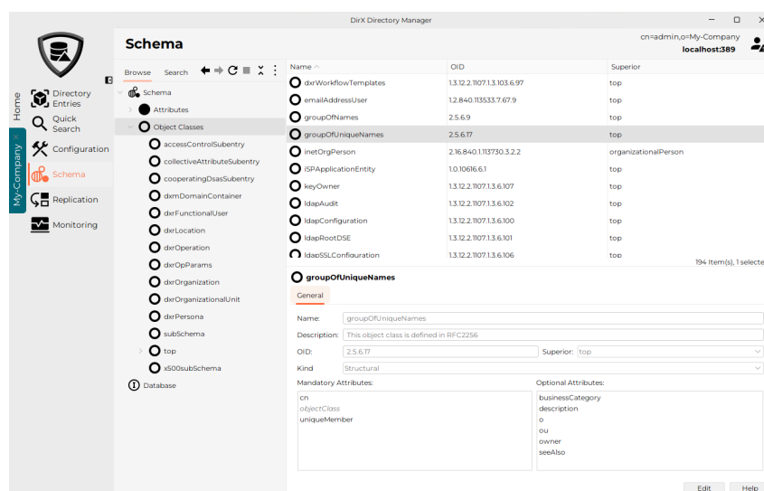
Figure 5 - DirX Manager - Schema Management
