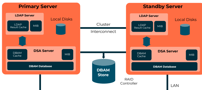
Figure 3 - DirX Directory - High Availability Cluster
