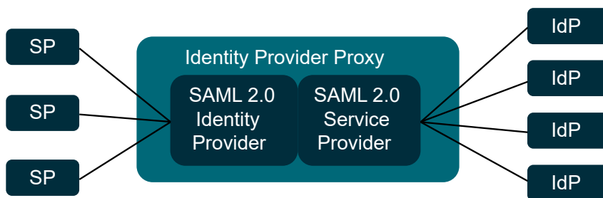
Figure 2 - DirX Access - SAML Proxying IdP in a Hub/Spoke Scenario
