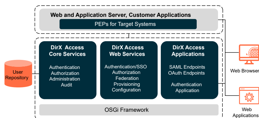
Figure 6 - DirX Access - Architecture and Integration into Applications
