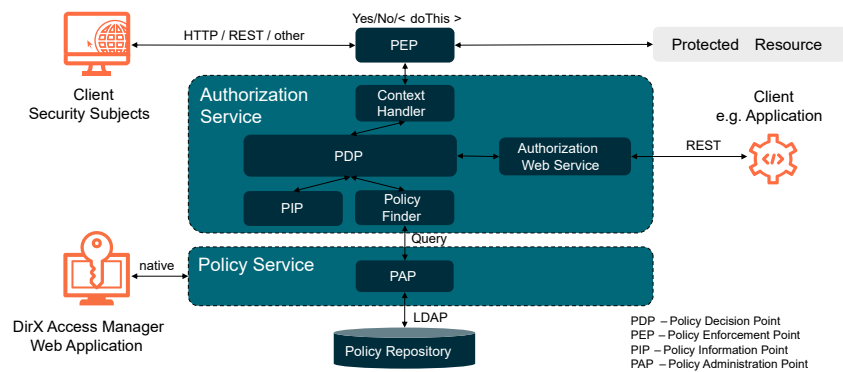
Figure 4 - DirX Access – XACML based authorization
