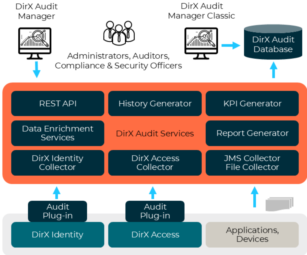
Figure 5. Key Components of DirX Audit
