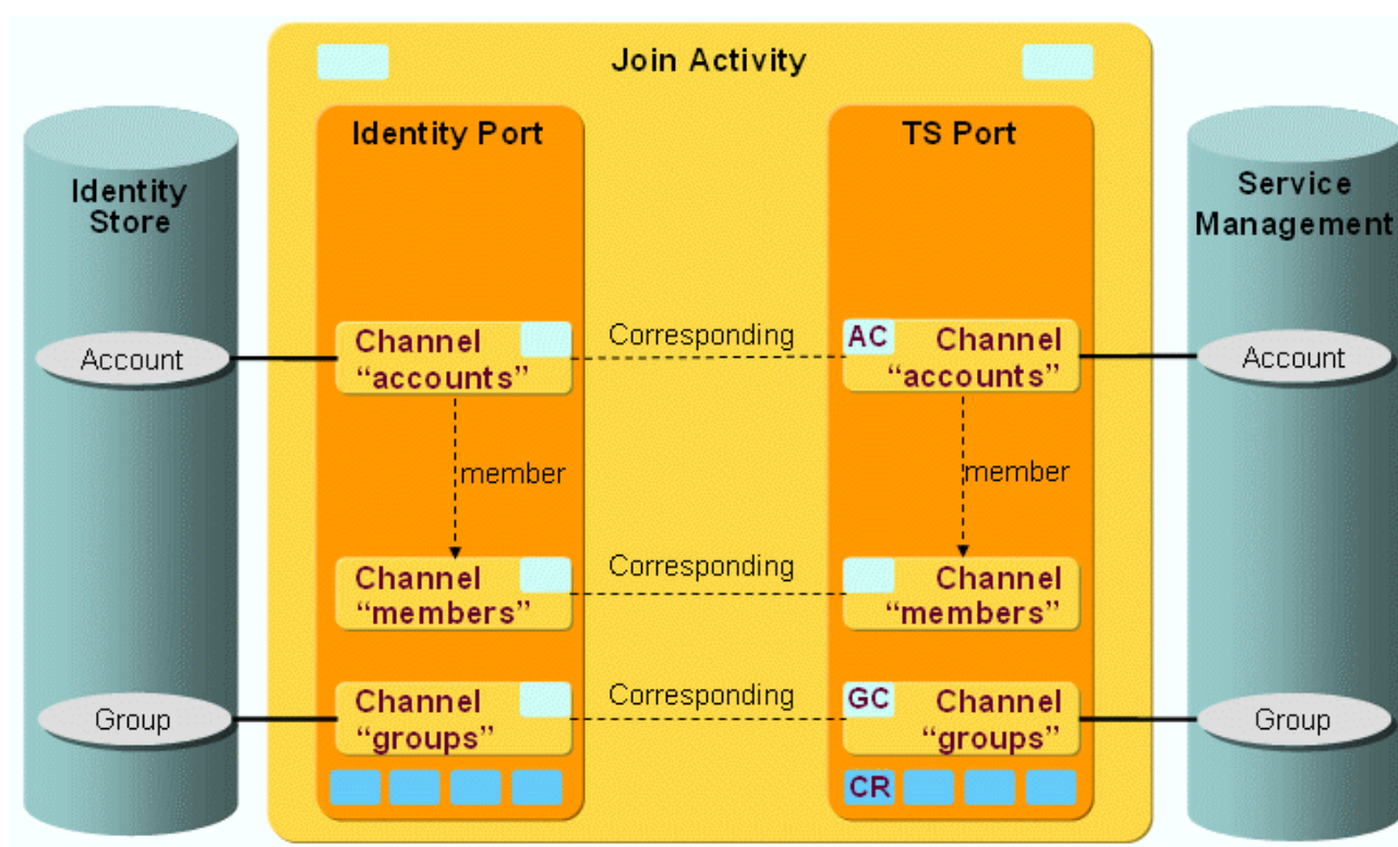
Figure 108. Service Management Channels and Object Types
