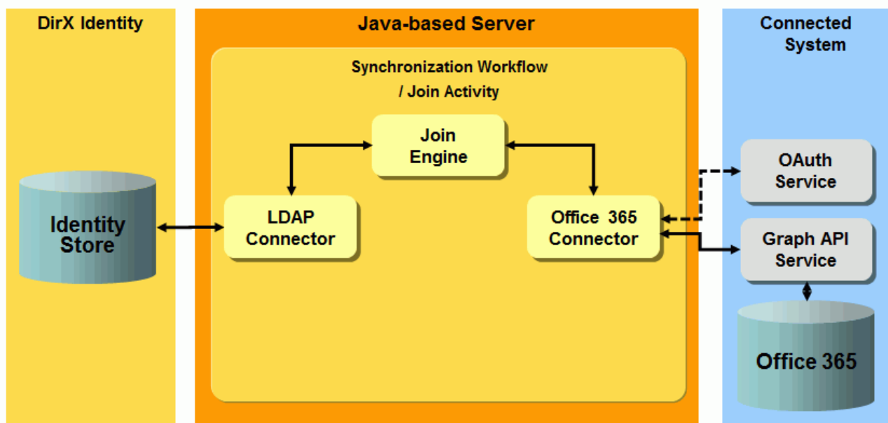
Figure 98. Microsoft 365 Provisioning Workflow Architecture
