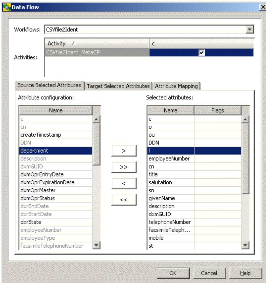
Figure 31. Data Flow Editor
