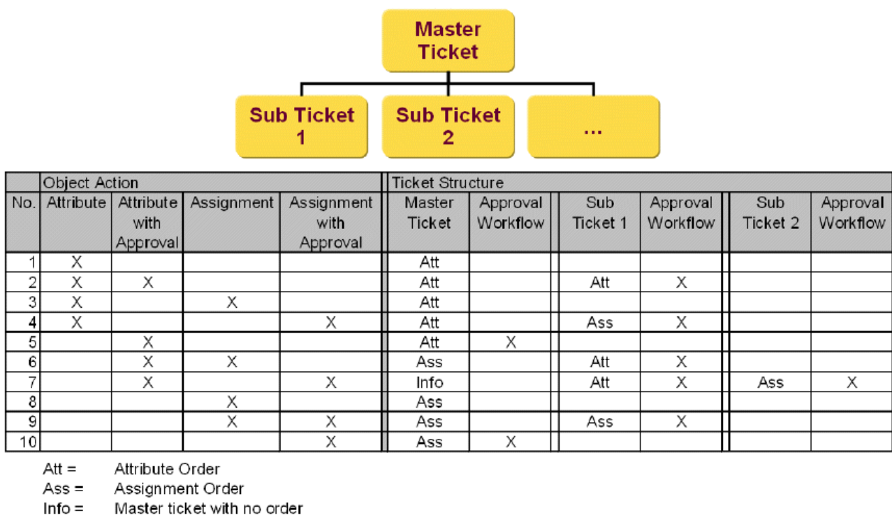
Figure 20. Ticket Structure
