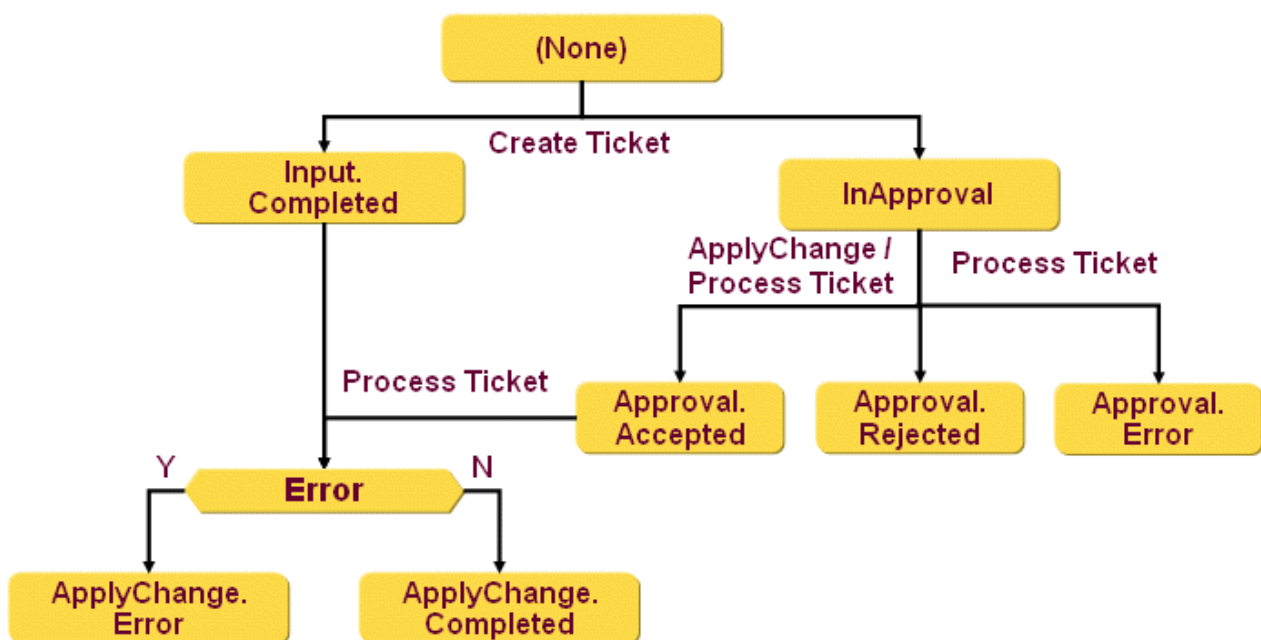
Figure 23. Ticket States
