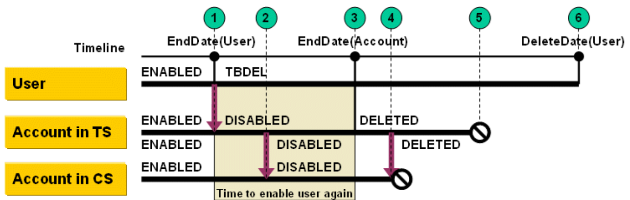
Figure 14. Relationship between User and Account Lifecycles
