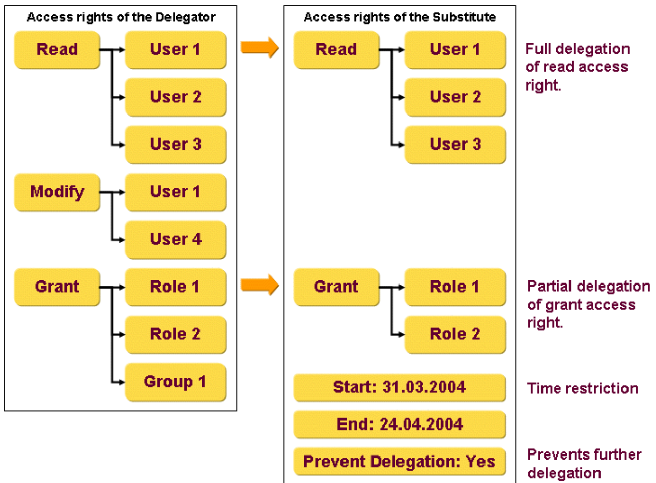
Figure 40. DirX Identity Provisioning Delegation Example
