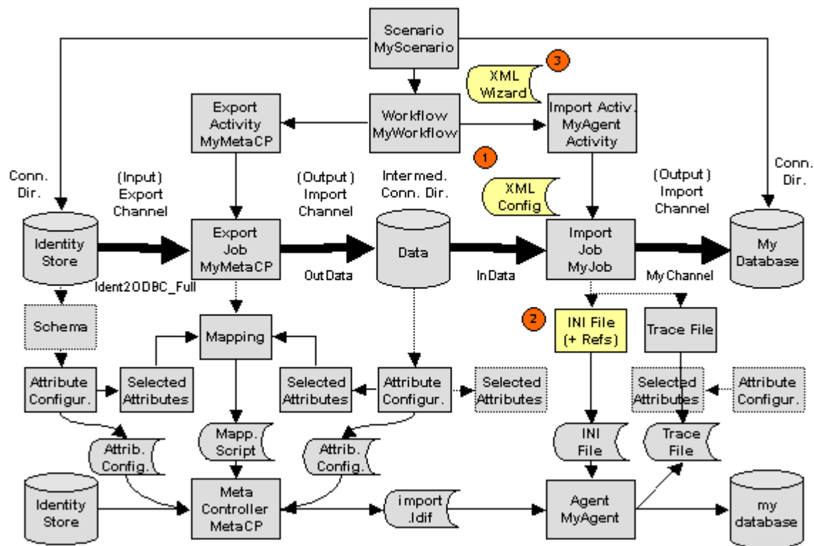
Figure 8. Level 3 Integration
