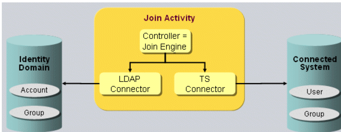
Figure 5. Provisioning Activity Structure
