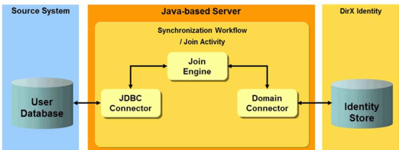
Figure 48. Relational Database User Import Workflow
