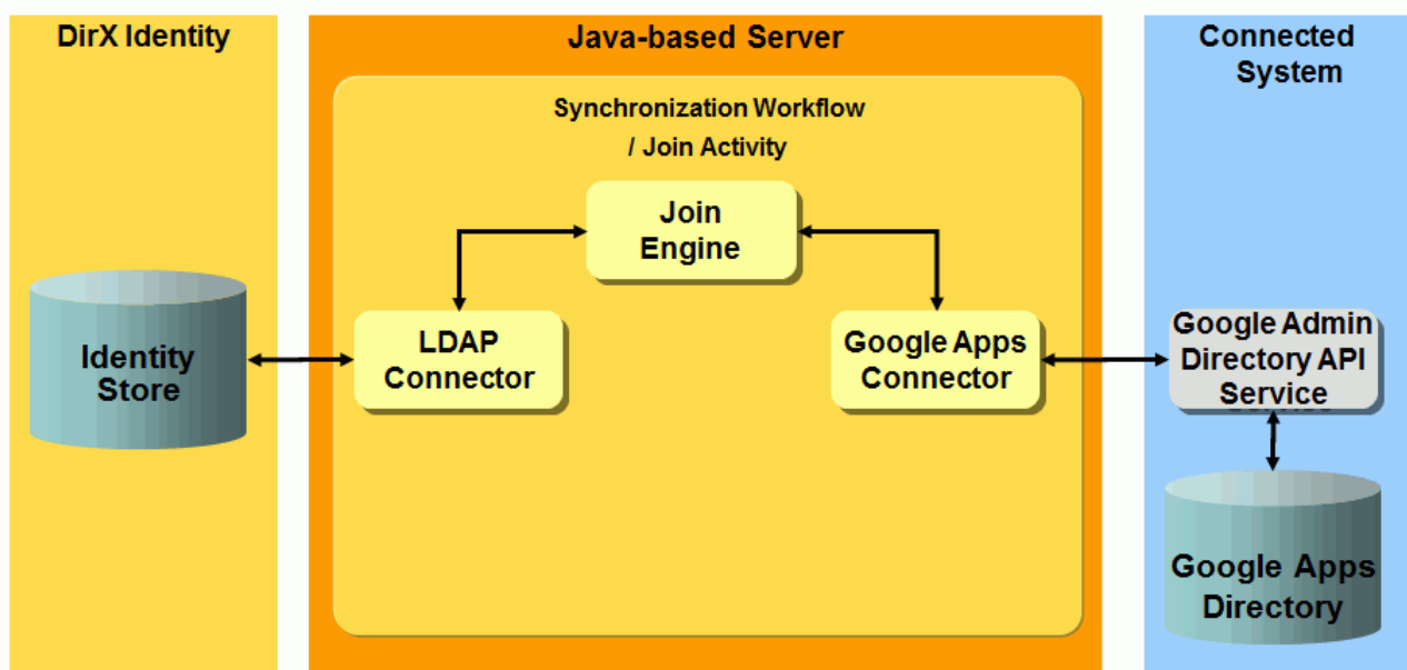
Figure 82. Google Apps Workflow Architecture
