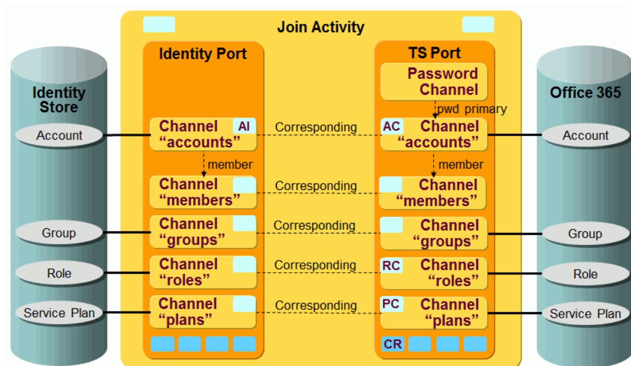
Figure 99. Microsoft 365 Provisioning Workflow Channels and Objects
