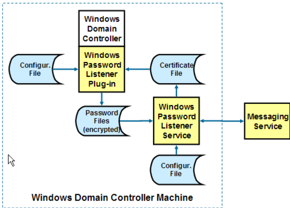
Figure 31. Windows Password Listener Architecture
