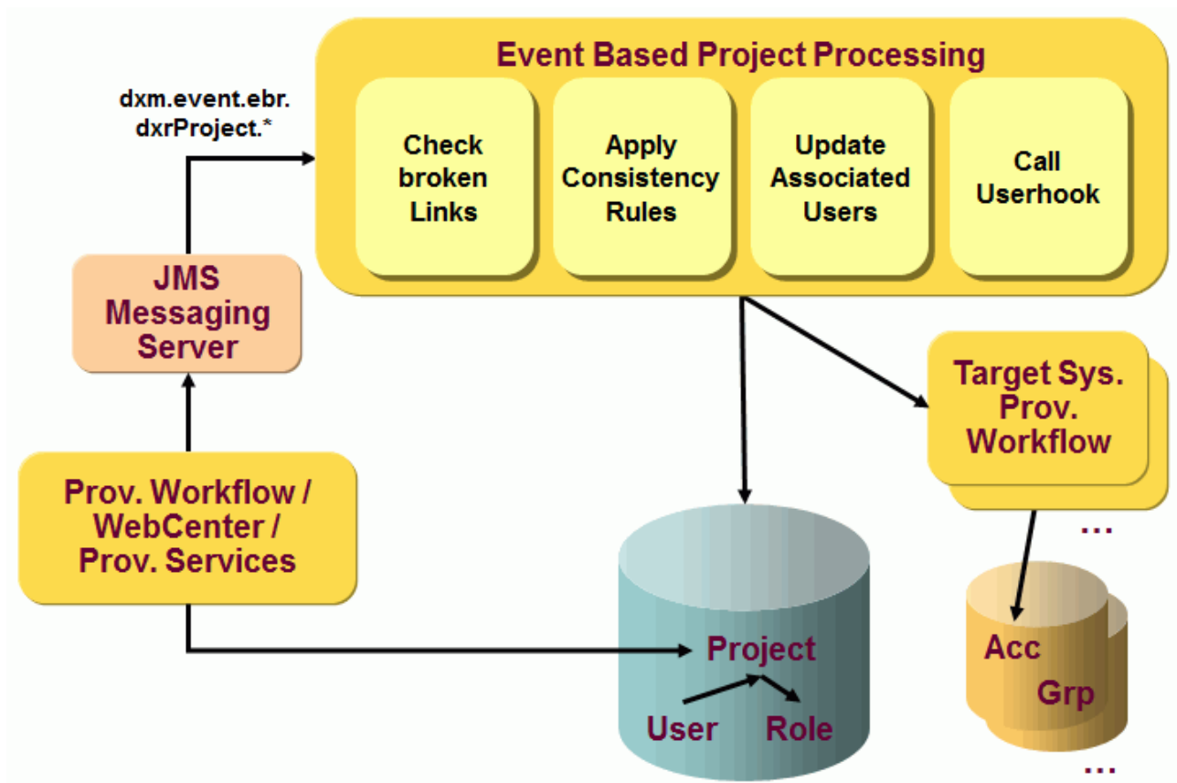
Figure 69. Event-based Maintenance Workflow Operation: Projects
