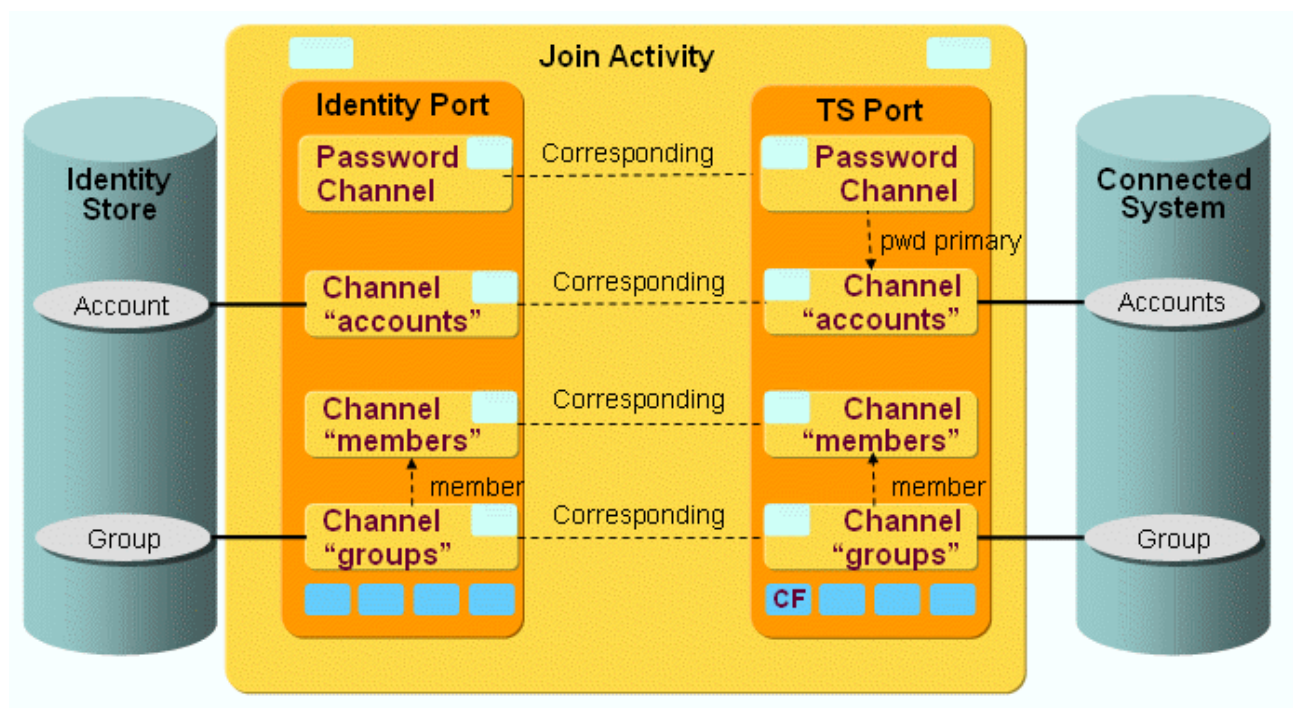
Figure 77. ADS Workflow Channels and Objects
