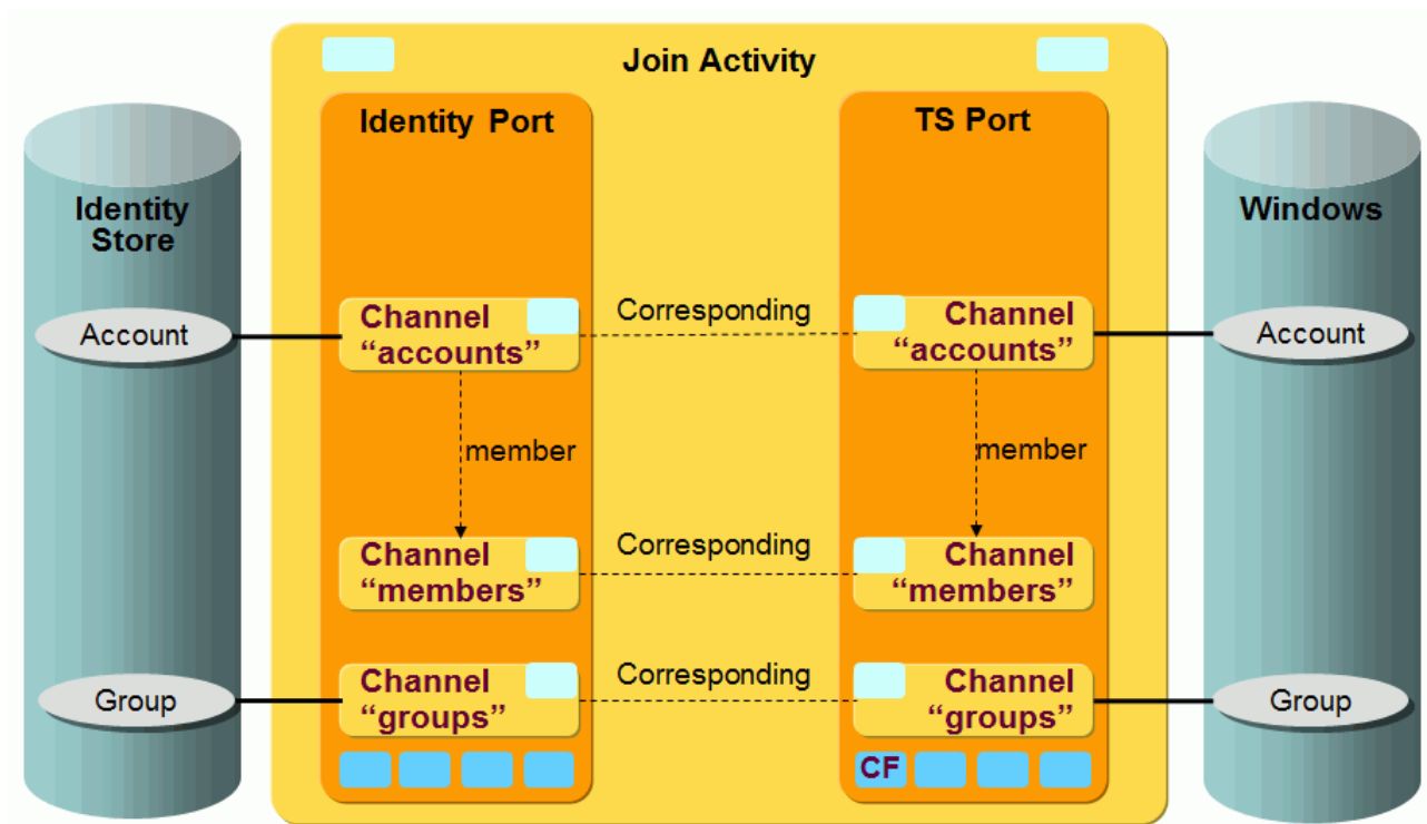
Figure 102. OpenICF Windows Local Accounts Provisioning Workflow Channels
