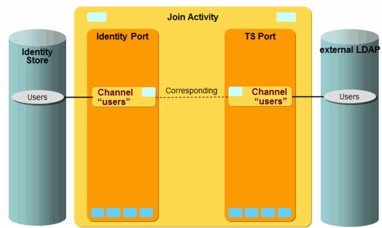
Figure 60. External LDAP Users Full Import Workflow Ports and Channels
