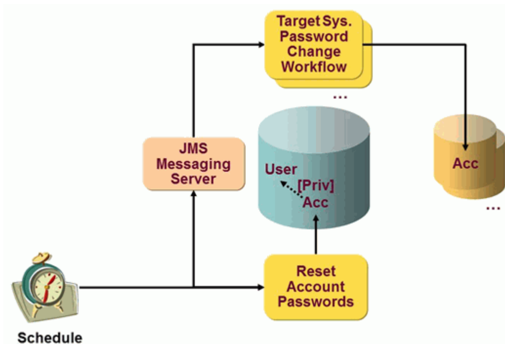
Figure 74. Account Password Management: Reset Account Passwords Workflow
