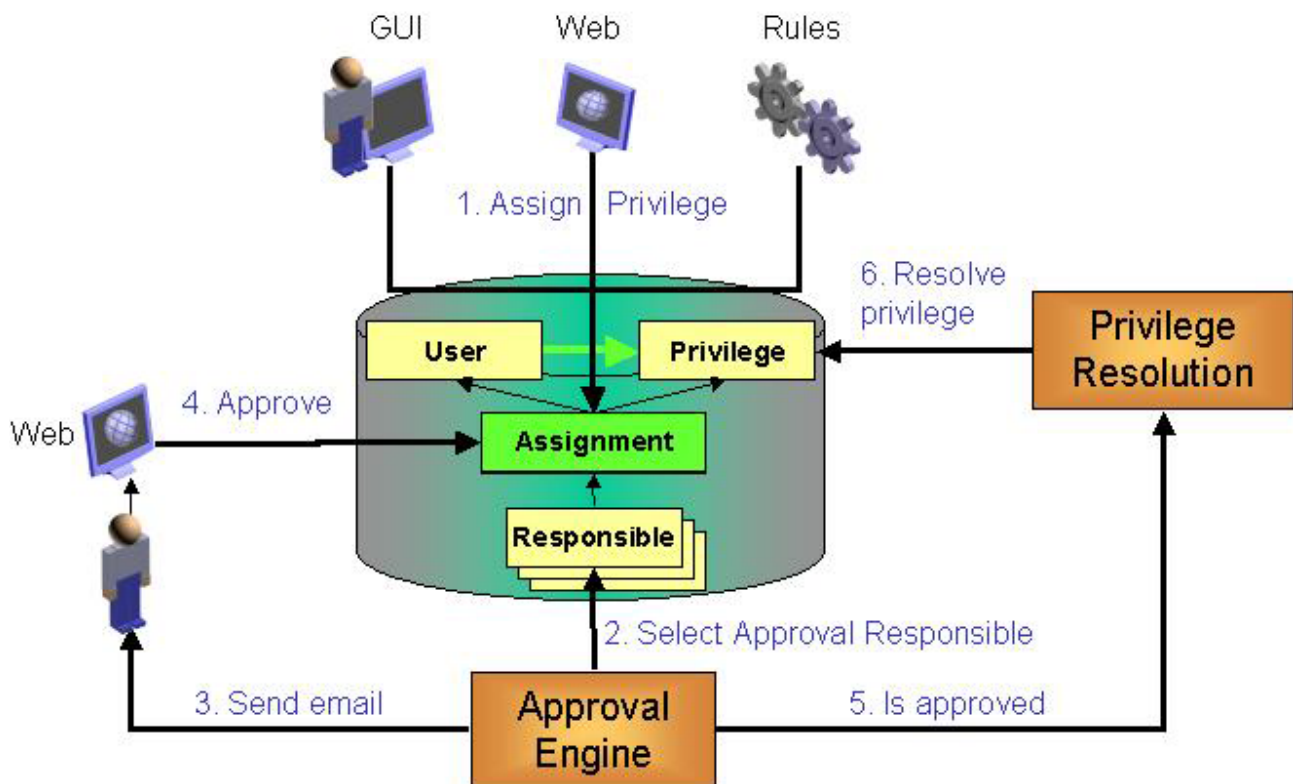
Figure 38. The DirX Identity Provisioning Approval Process
