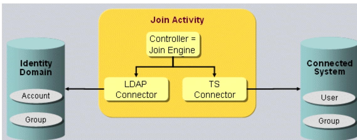
Figure 5. Provisioning Activity Structure
