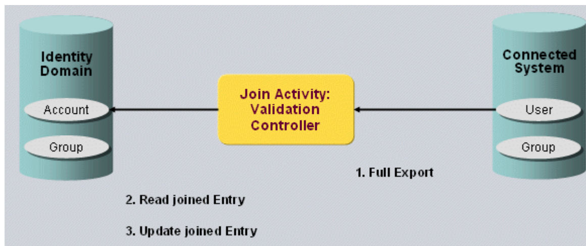
Figure 9. Validation Controller Processing
