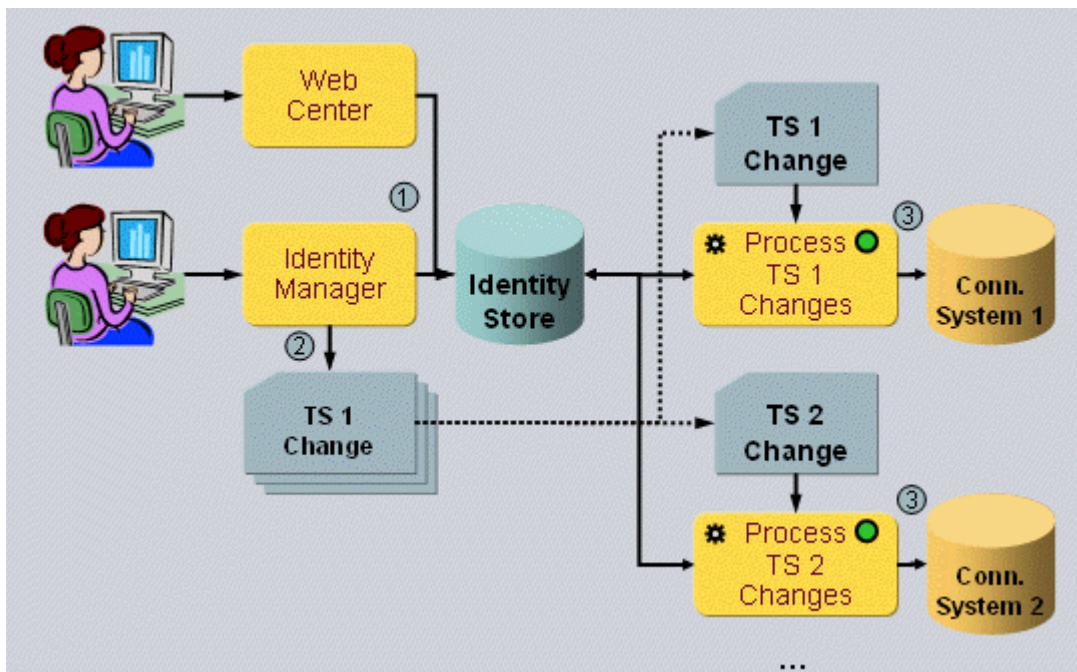
Figure 11. Event-Triggered Provisioning Workflow
