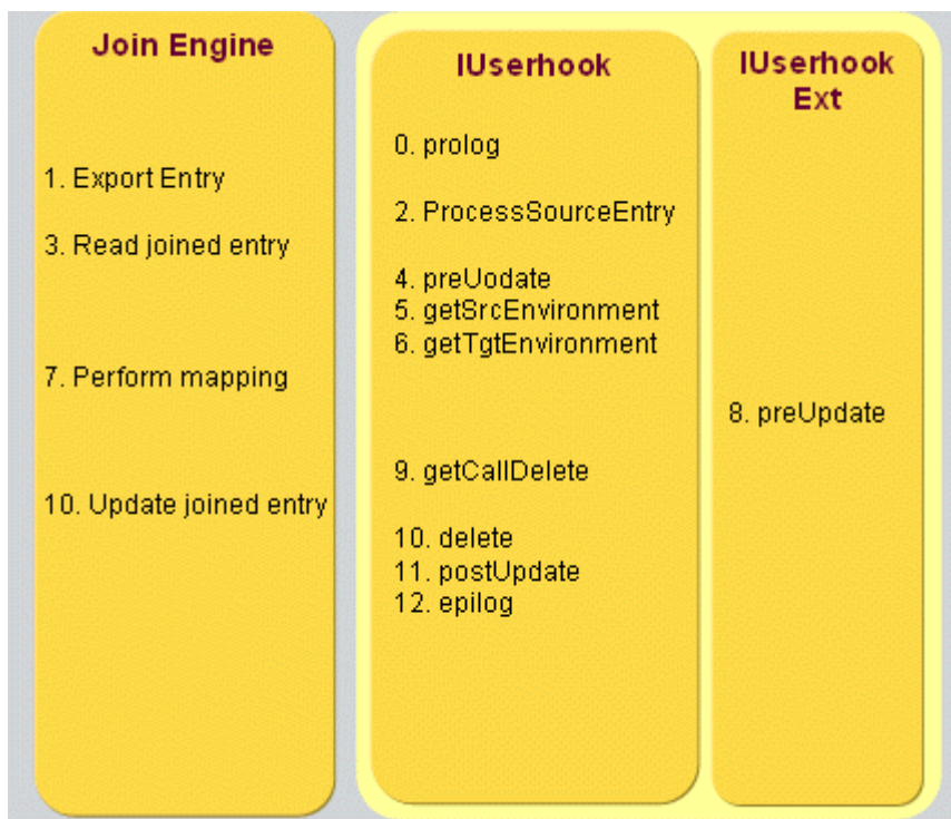
Figure 15. Join Engine-User Hook Operation Calling Sequence
