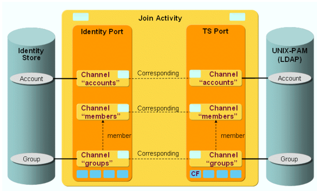
Figure 122. UNIX-PAM Provisioning Workflow Channels and Objects
