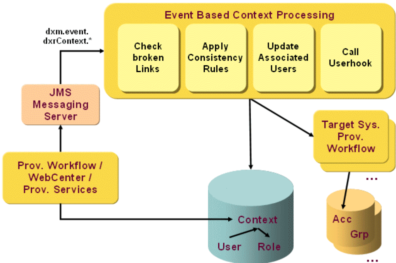
Figure 66. Event-based Maintenance Workflow Operation: Context Objects
