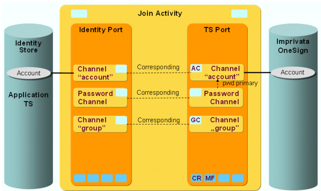
Figure 87. Imprivata Workflow Channels for Imprivata OneSign Account Objects
