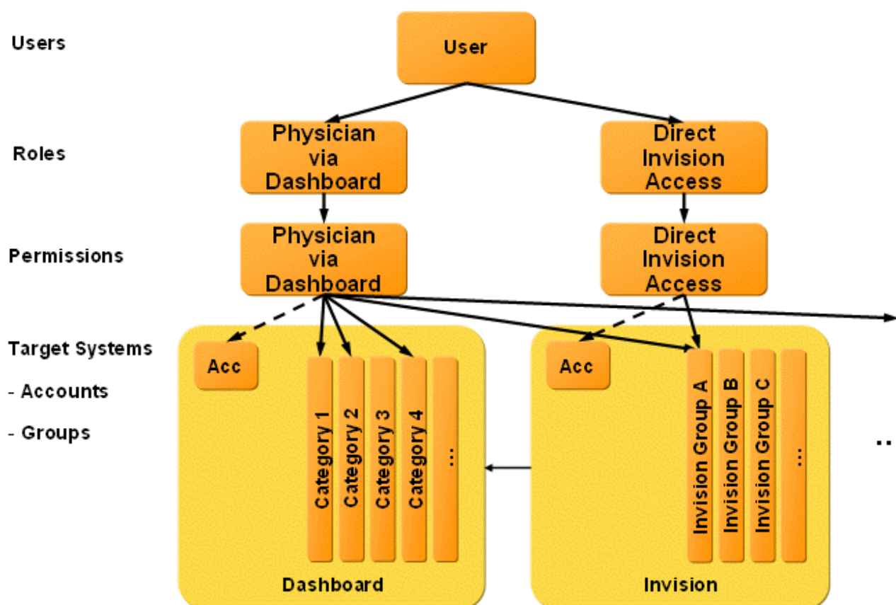
Figure 117. Dashboard Privilege Model
