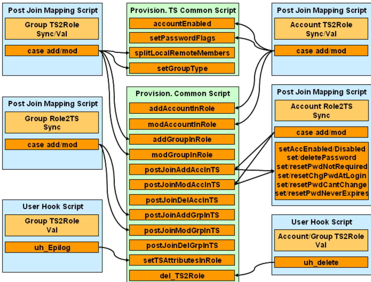
Figure 22. DirX Identity Connectivity and Provisioning Script Function Calls
