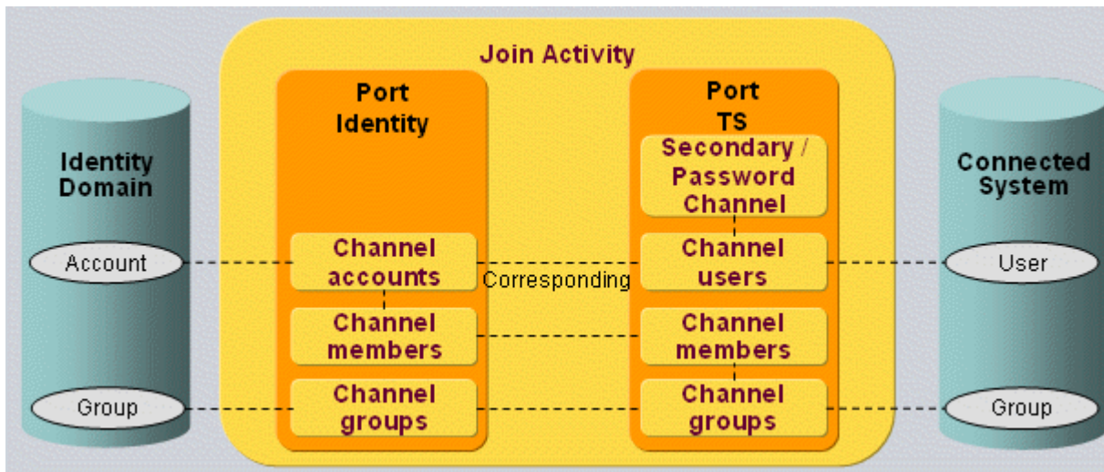
Figure 6. Provisioning Ports and Channels
