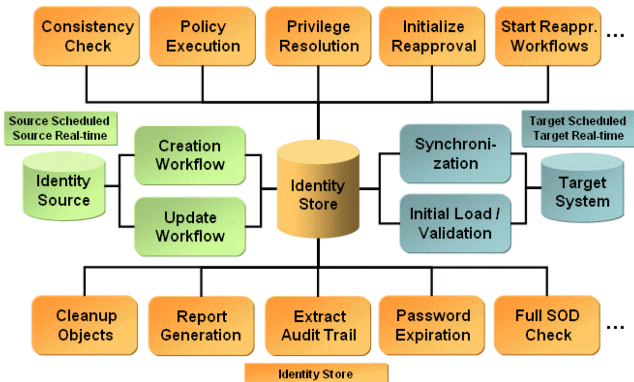
Figure 46. DirX Identity Default Connectivity Scenario
