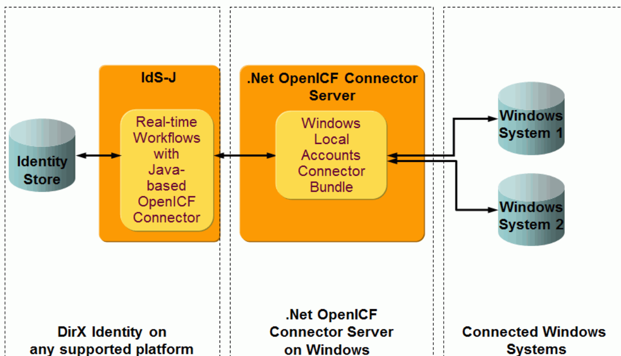
Figure 100. OpenICF Windows Local Accounts Deployment
