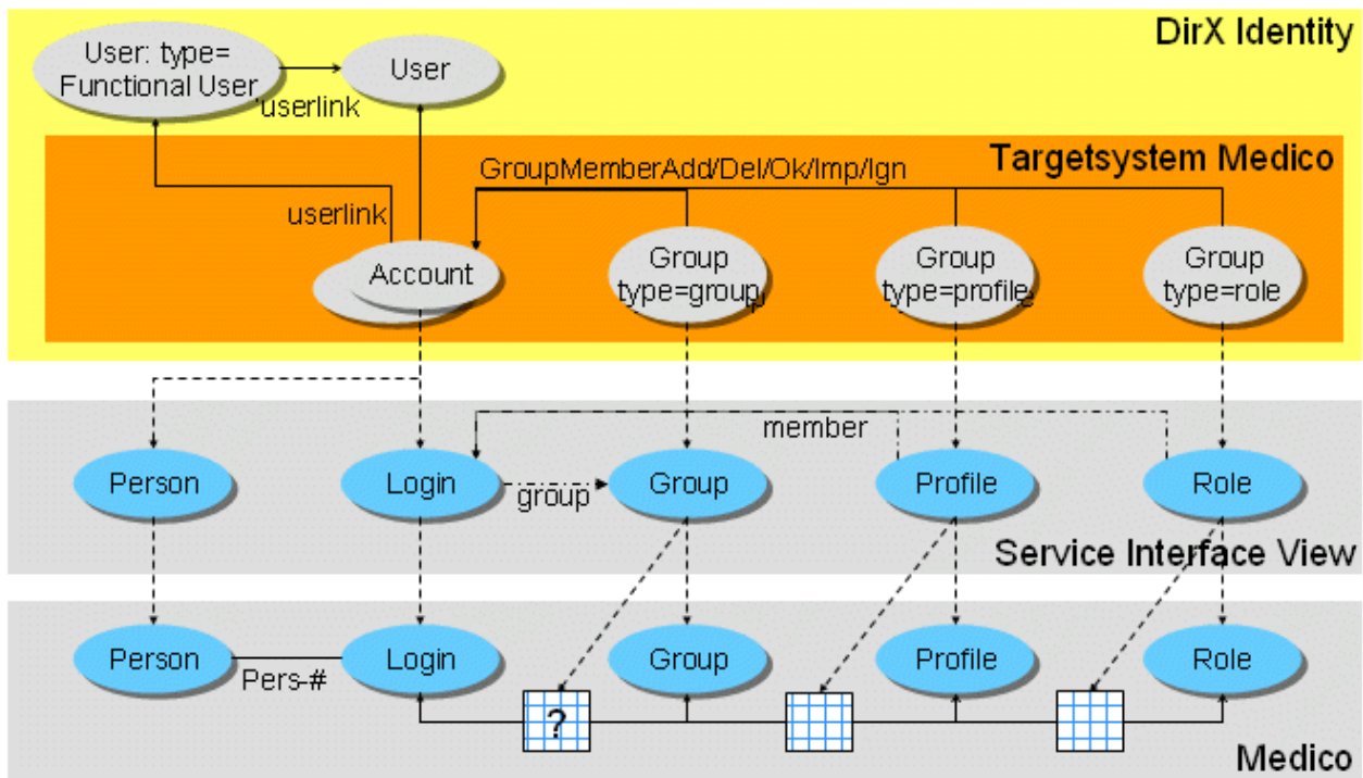
Figure 96. Relationships between Medico and DirX Identity Objects
