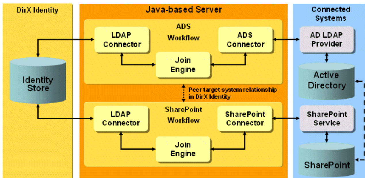
Figure 109. SharePoint Provisioning Workflow Architecture
