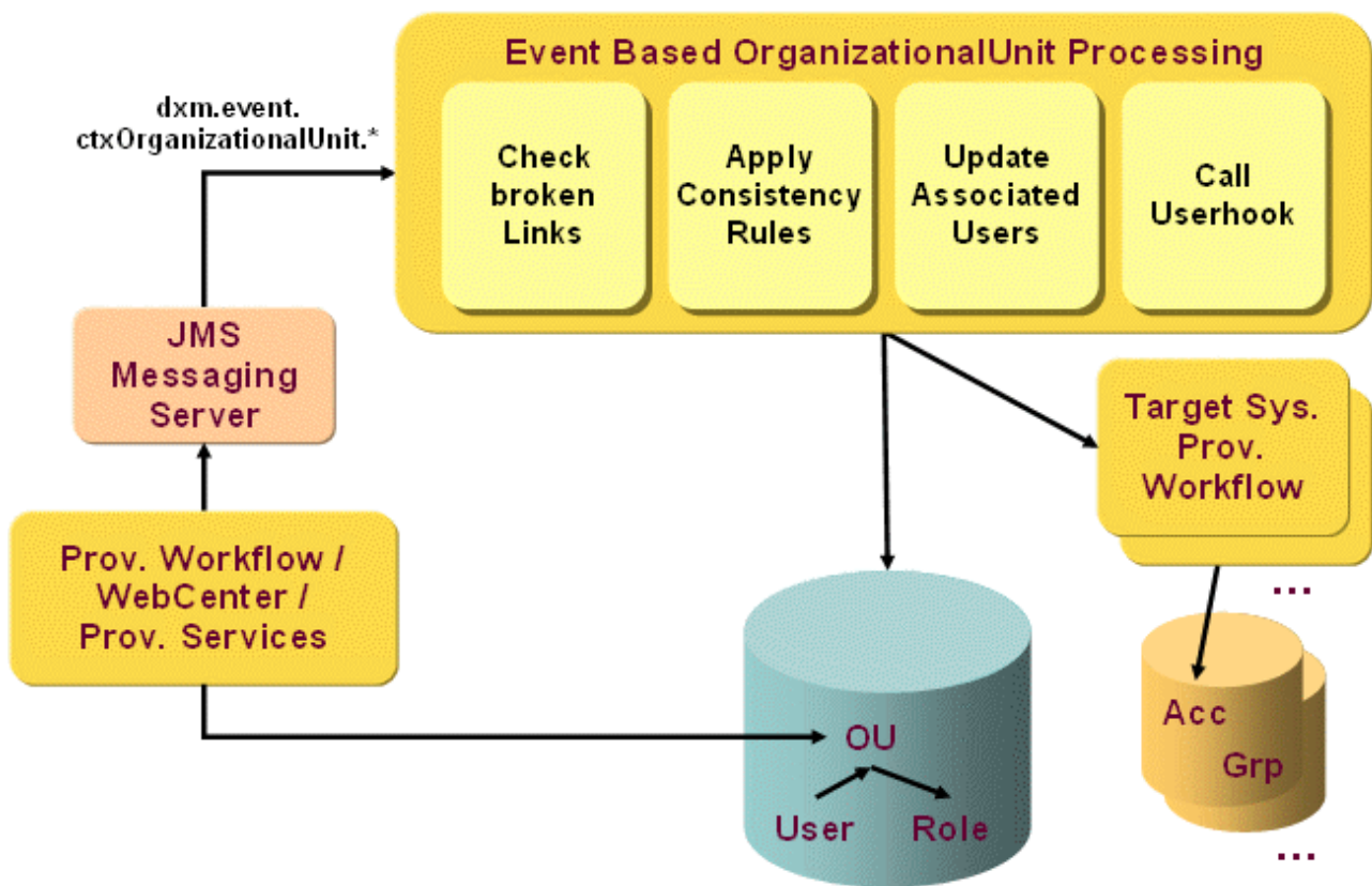
Figure 65. Event-based Maintenance Workflow Operation: Organizational Units
