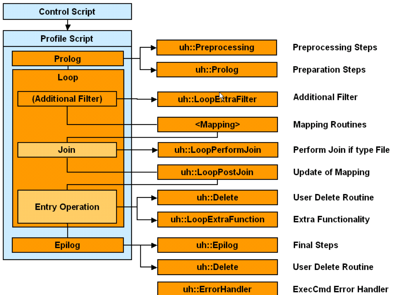
Figure 28. User Hook Routines
