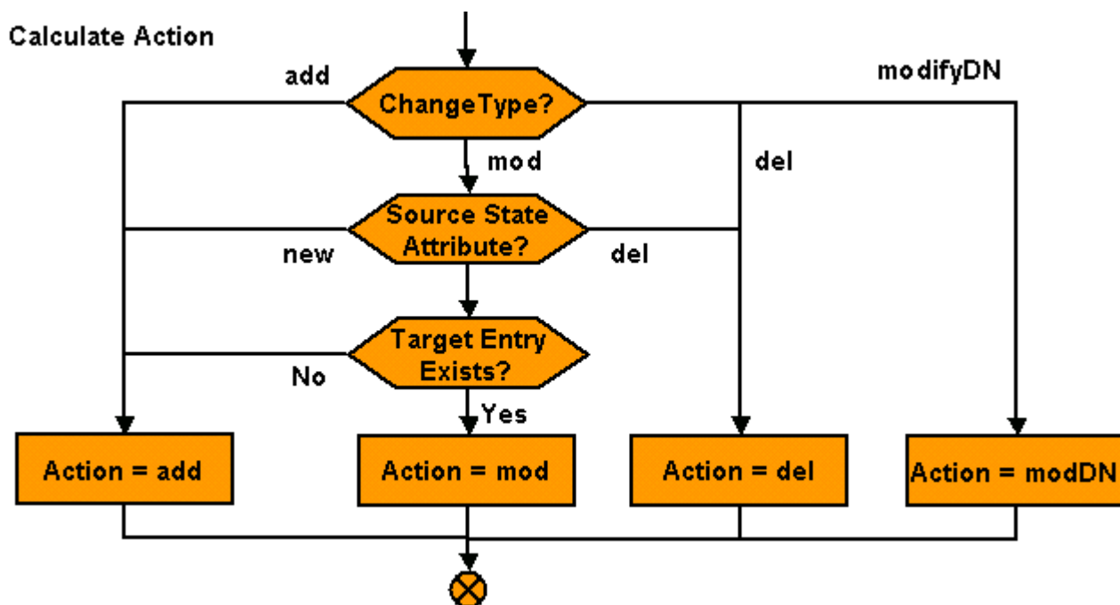
Figure 24. Profile Script - Calculate Action Logic
