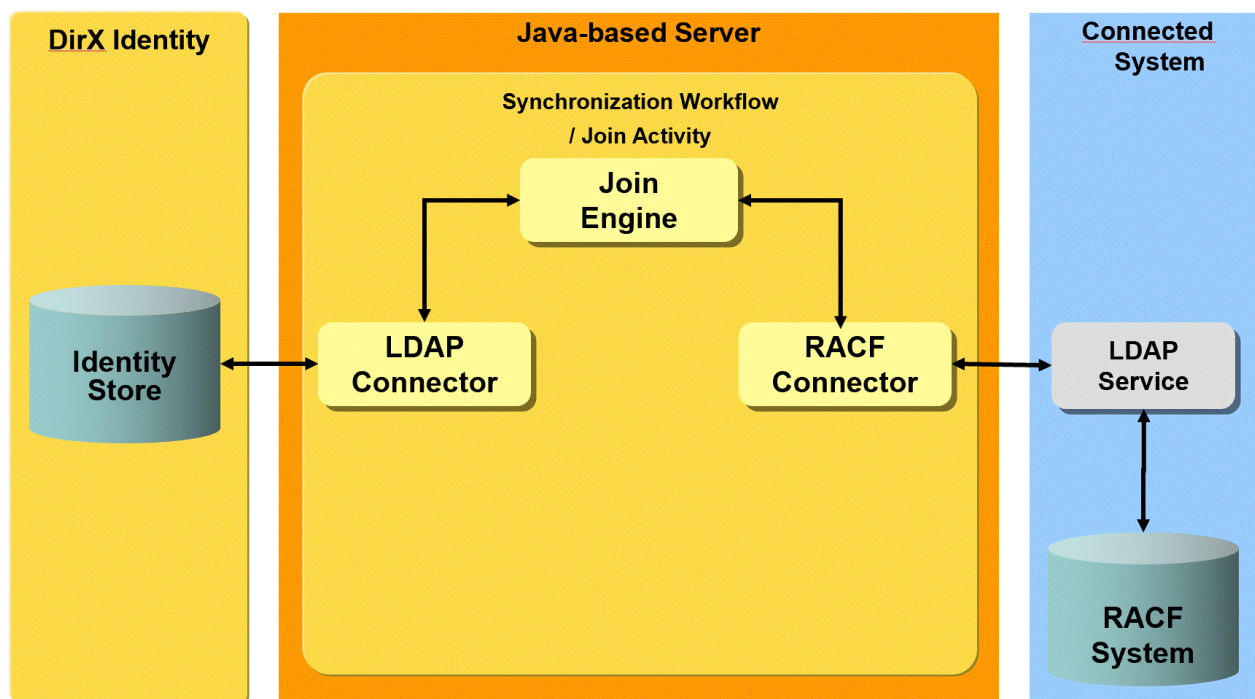
Figure 103. RACF Workflow Architecture
