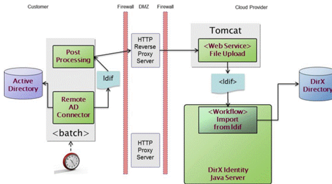
Figure 59. Remote AD Connector Operation
