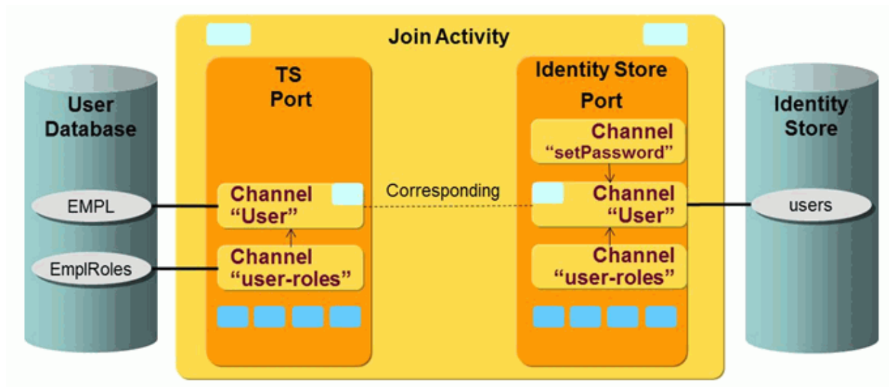
Figure 49. Relational Database User Import Workflow Ports and Channels
