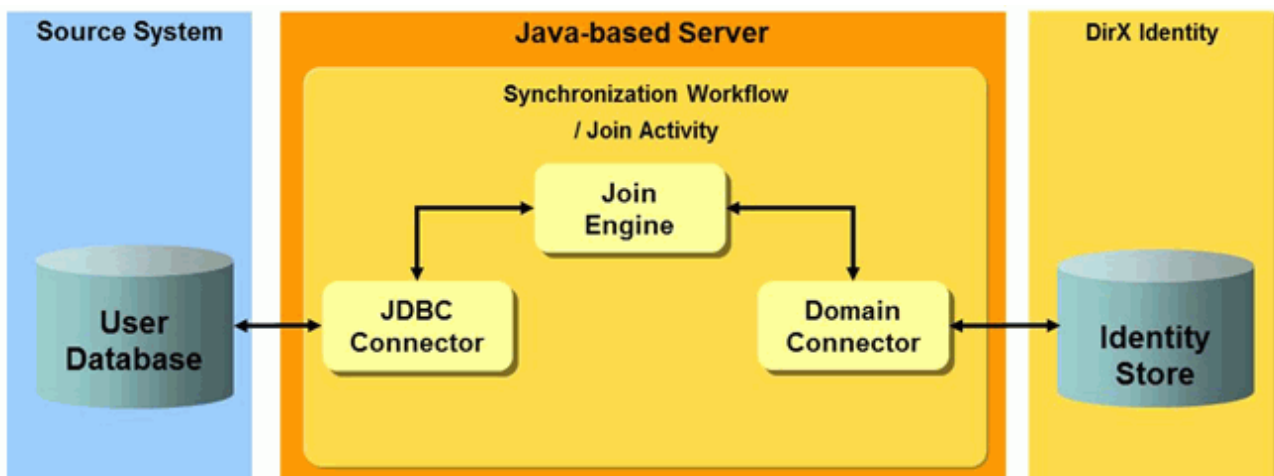
Figure 48. Relational Database User Import Workflow
