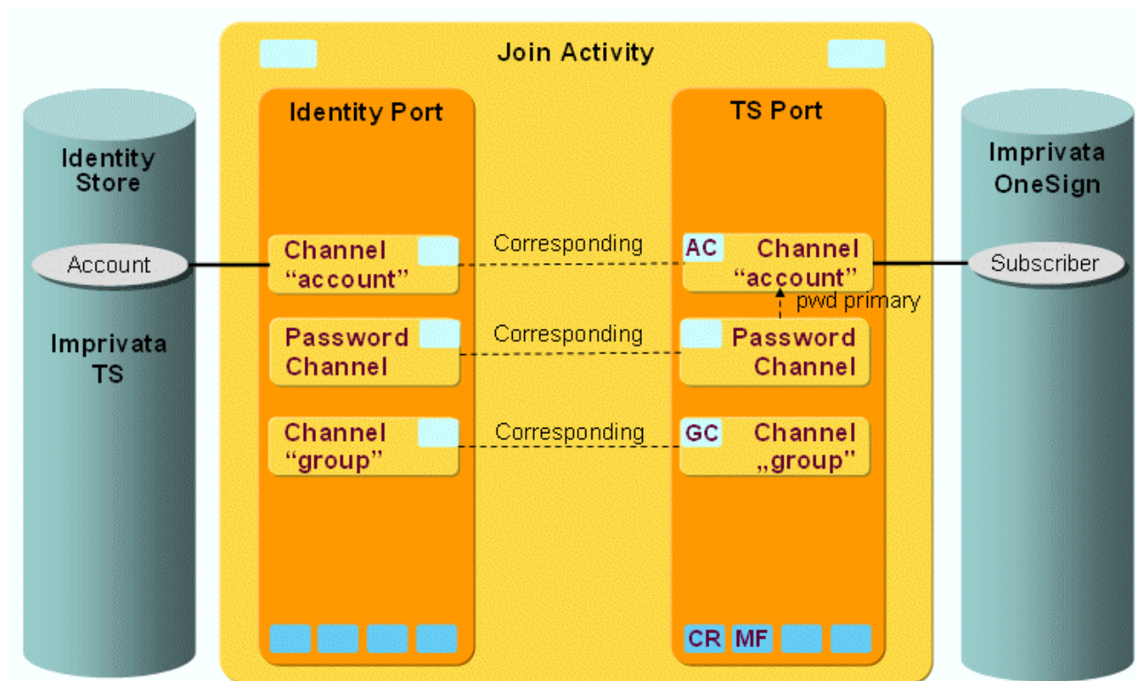
Figure 86. Imprivata Workflow Channels for Imprivata OneSign Subscriber Objects
