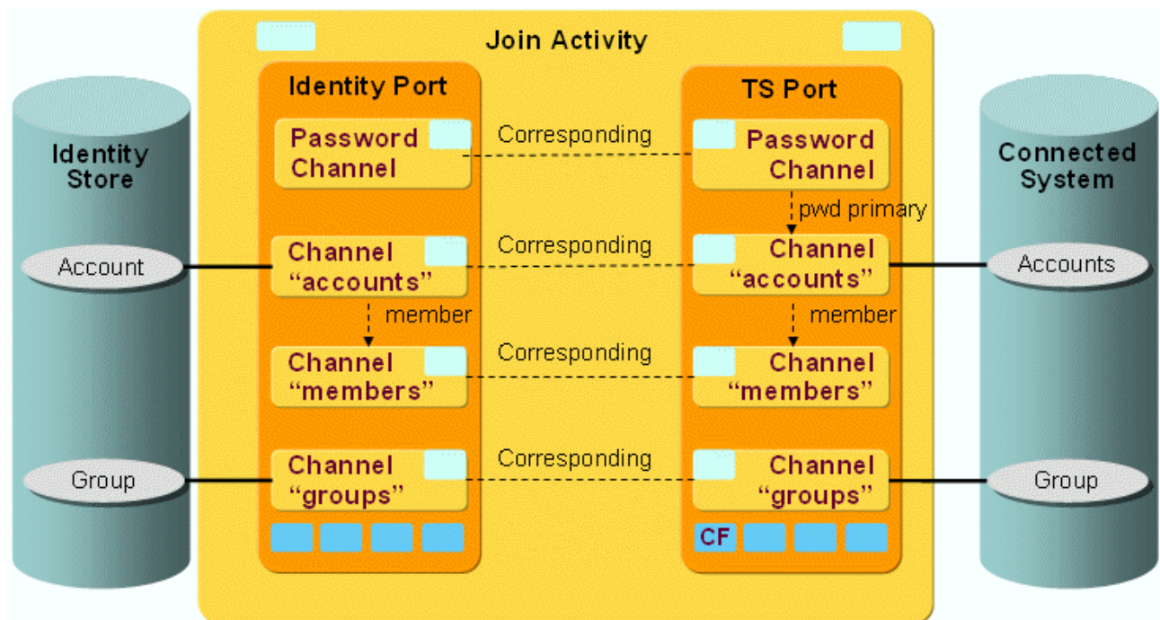
Figure 91. LDAP Workflow Channels
