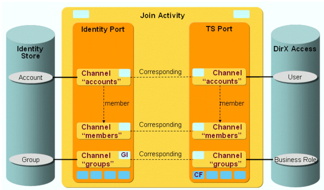
Figure 120. DirX Access Provisioning Workflow Channels and Objects
