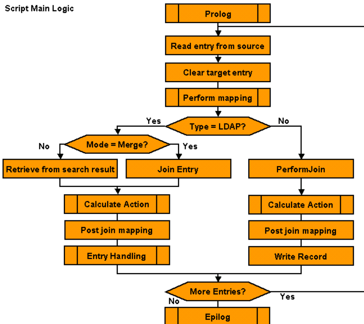
Figure 23. Profile Script Algorithm
