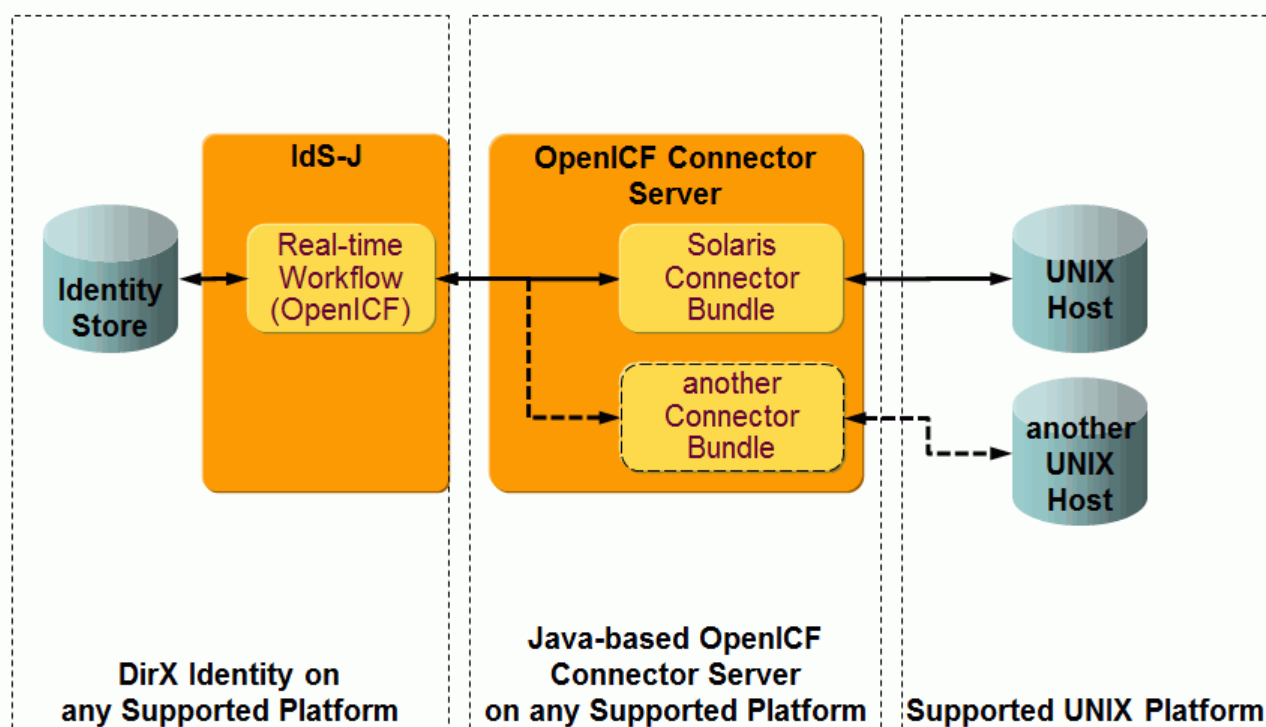
Figure 113. UNIX-OpenICF Connector Server Architecture
