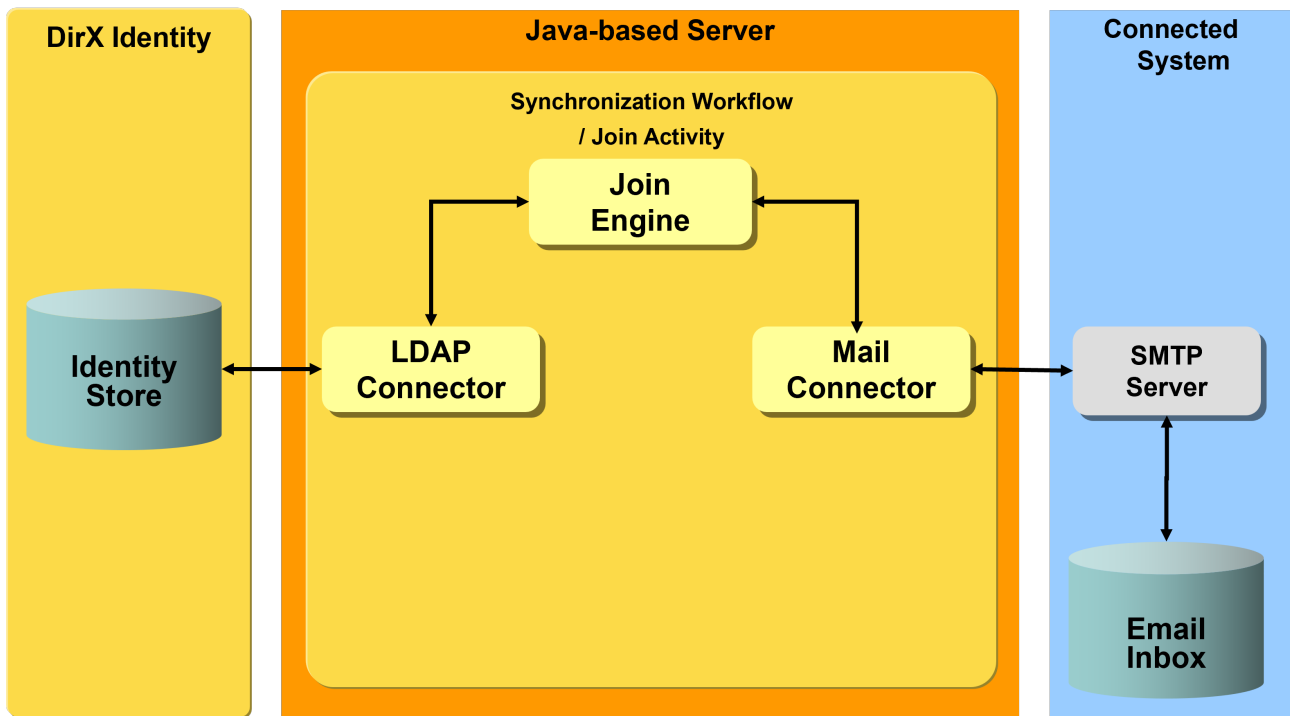
Figure 94. Mail Provisioning Workflow Architecture
