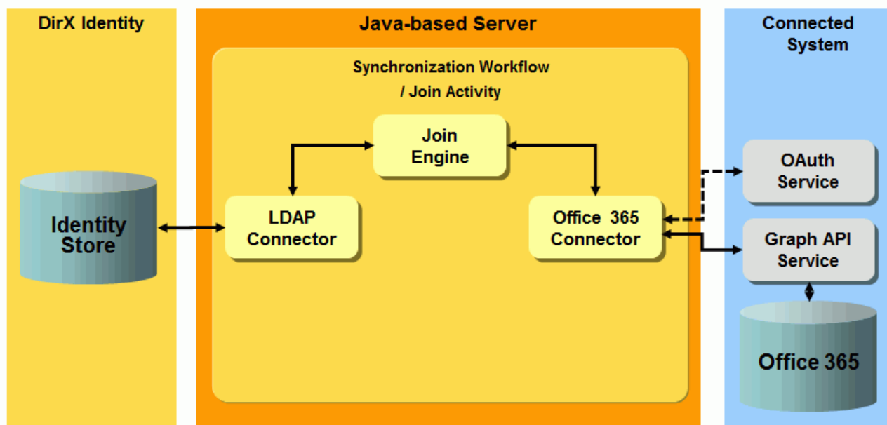
Figure 98. Microsoft 365 Provisioning Workflow Architecture
