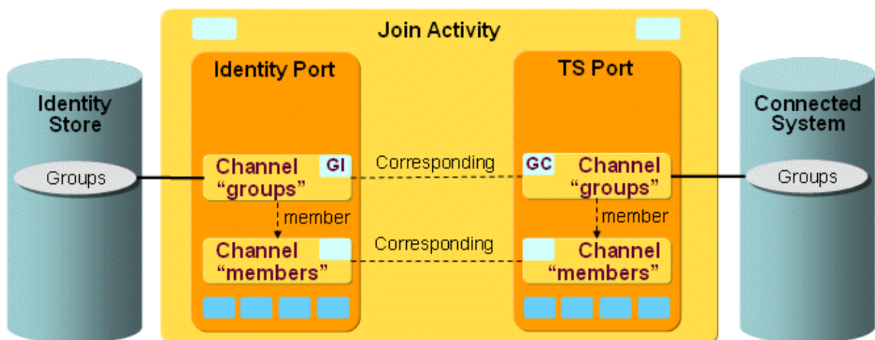
Figure 110. SharePoint Provisioning Workflow Channels and Objects
