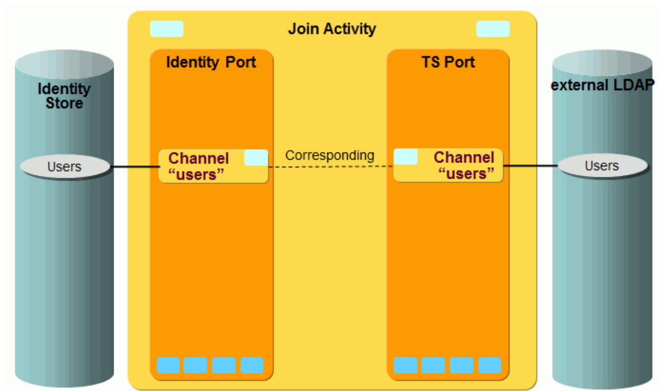
Figure 61. External LDAP User Import Workflow Ports and Channels
