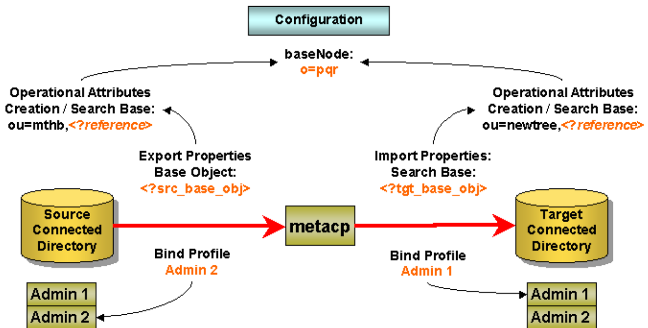
Figure 27. Base Object Reference Concept
