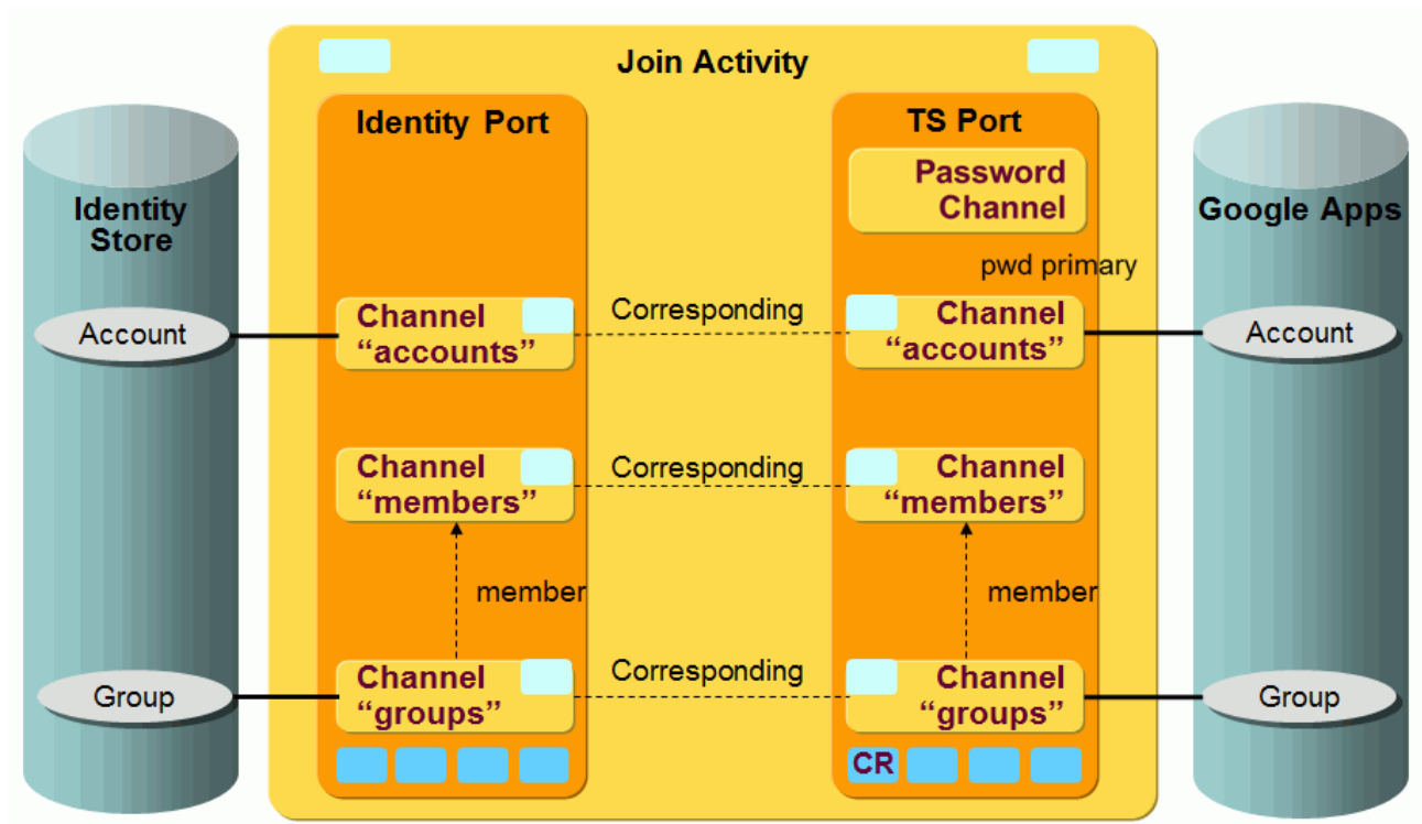
Figure 83. Google Apps Workflow Channels and Objects
