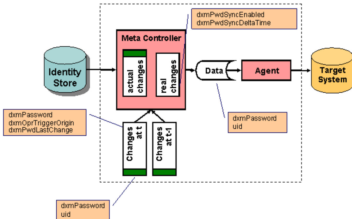
Figure 29. Workflow-Side Delta Handling
