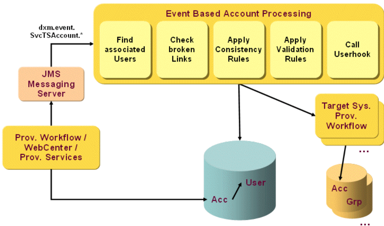
Figure 63. Event-based Maintenance Workflow Operation: Accounts
