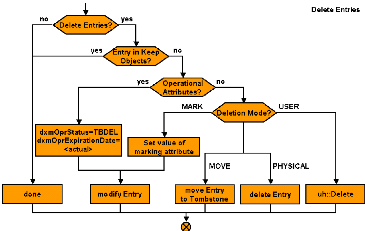
Figure 26. Profile Script - Entry Deletion Logic
