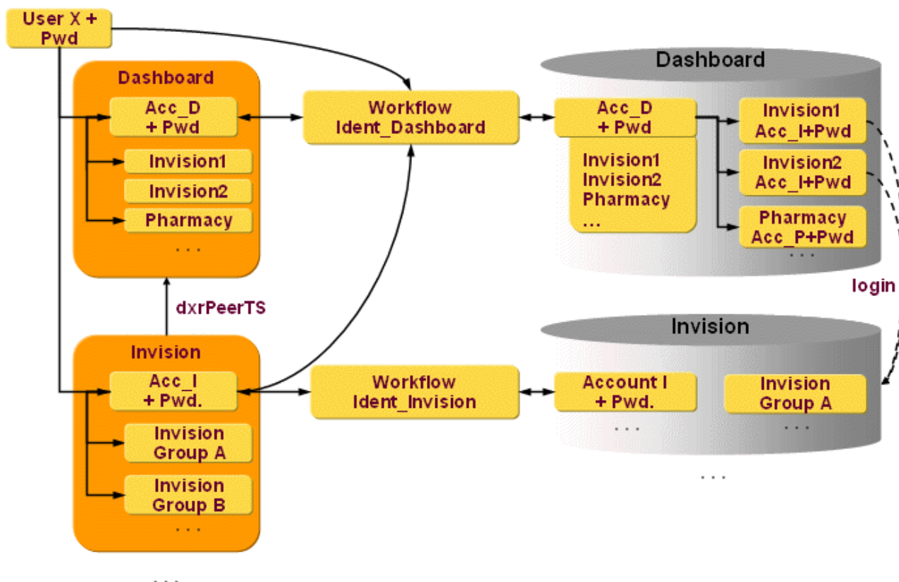
Figure 118. DirX Identity Dashboard Synchronization Model
