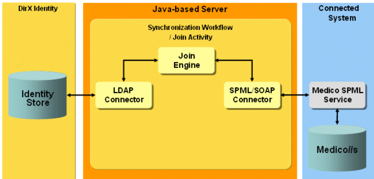
Figure 95. Medico Provisioning Workflow Architecture
