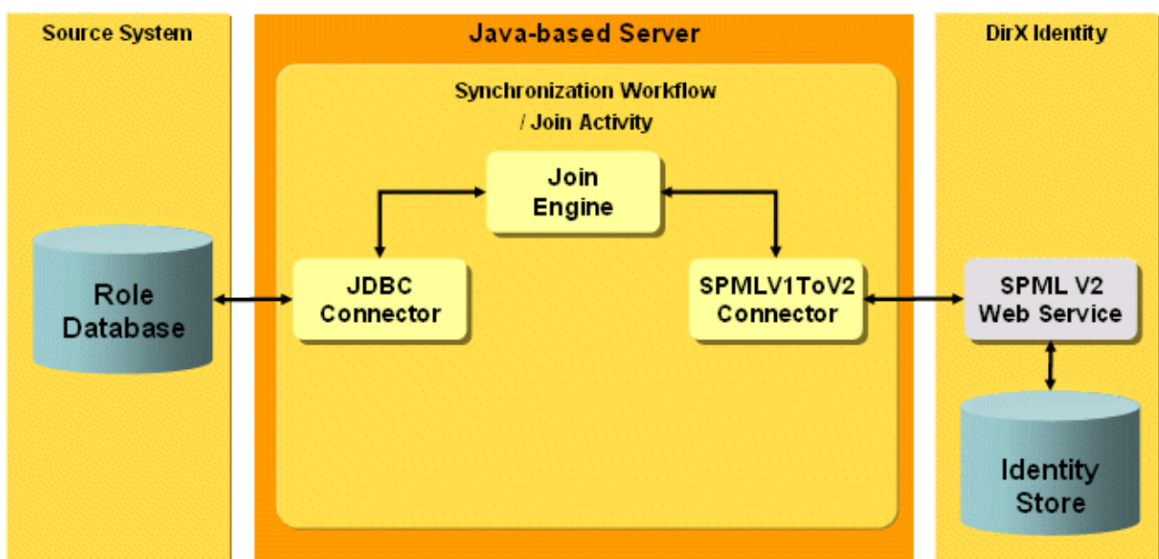
Figure 52. Role Import Workflow
