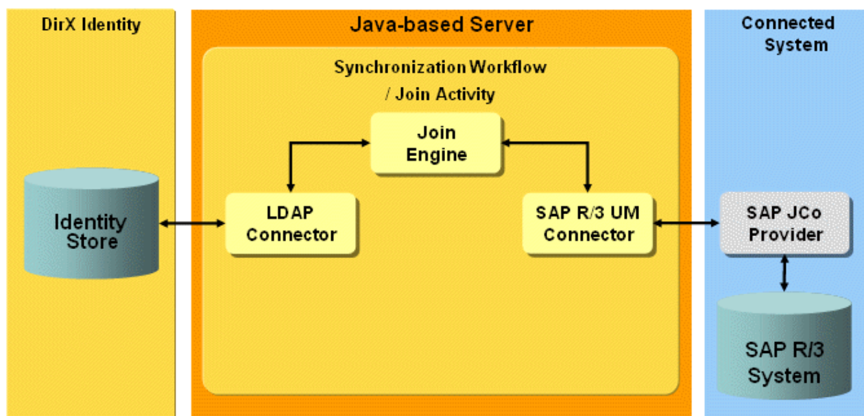
Figure 106. SAP R/3 UM Workflow Architecture
