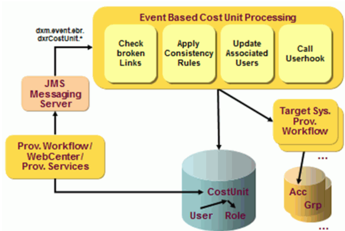
Figure 68. Event-based Maintenance Workflow Operation: Cost Units
