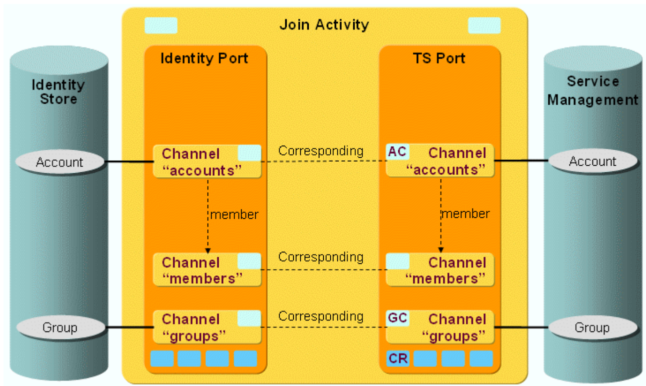
Figure 108. Service Management Channels and Object Types
