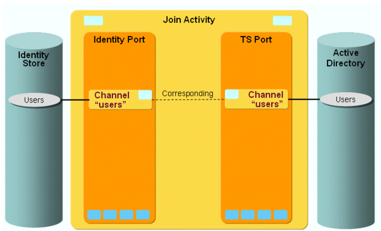
Figure 47. ADS User Import Workflow Ports and Channels
