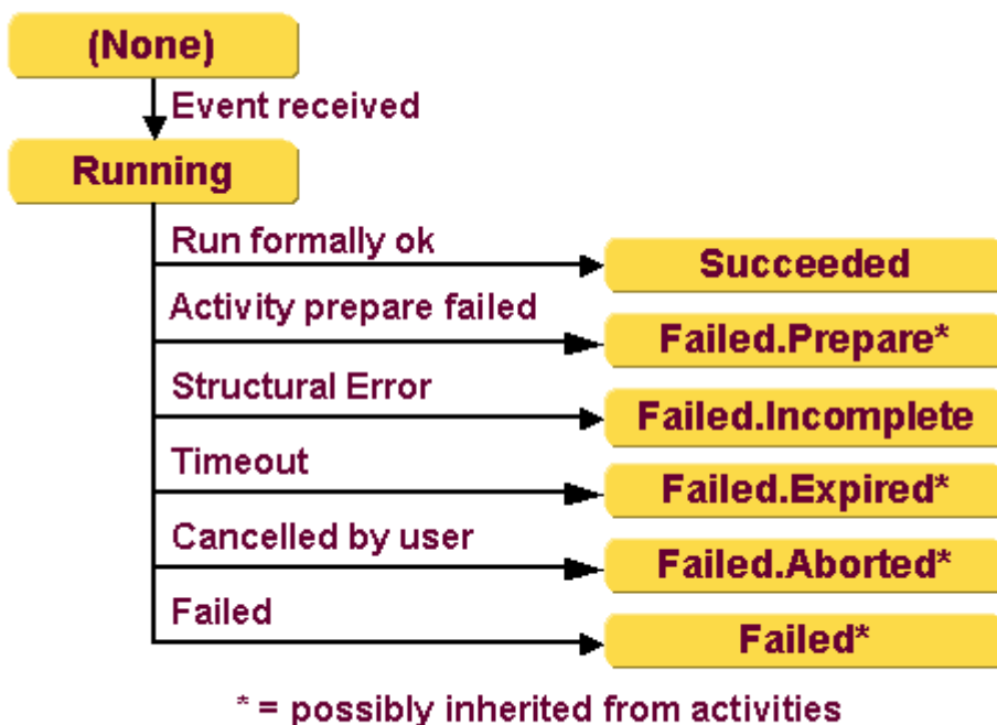
Figure 2. Request Workflow States
