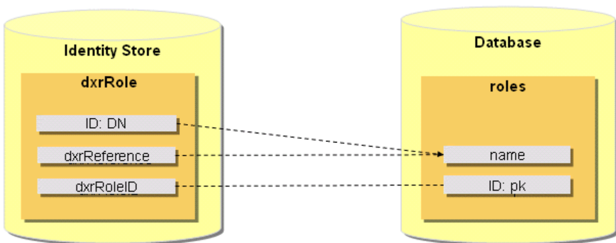
Figure 54. Role Import Workflow Channel Mapping
