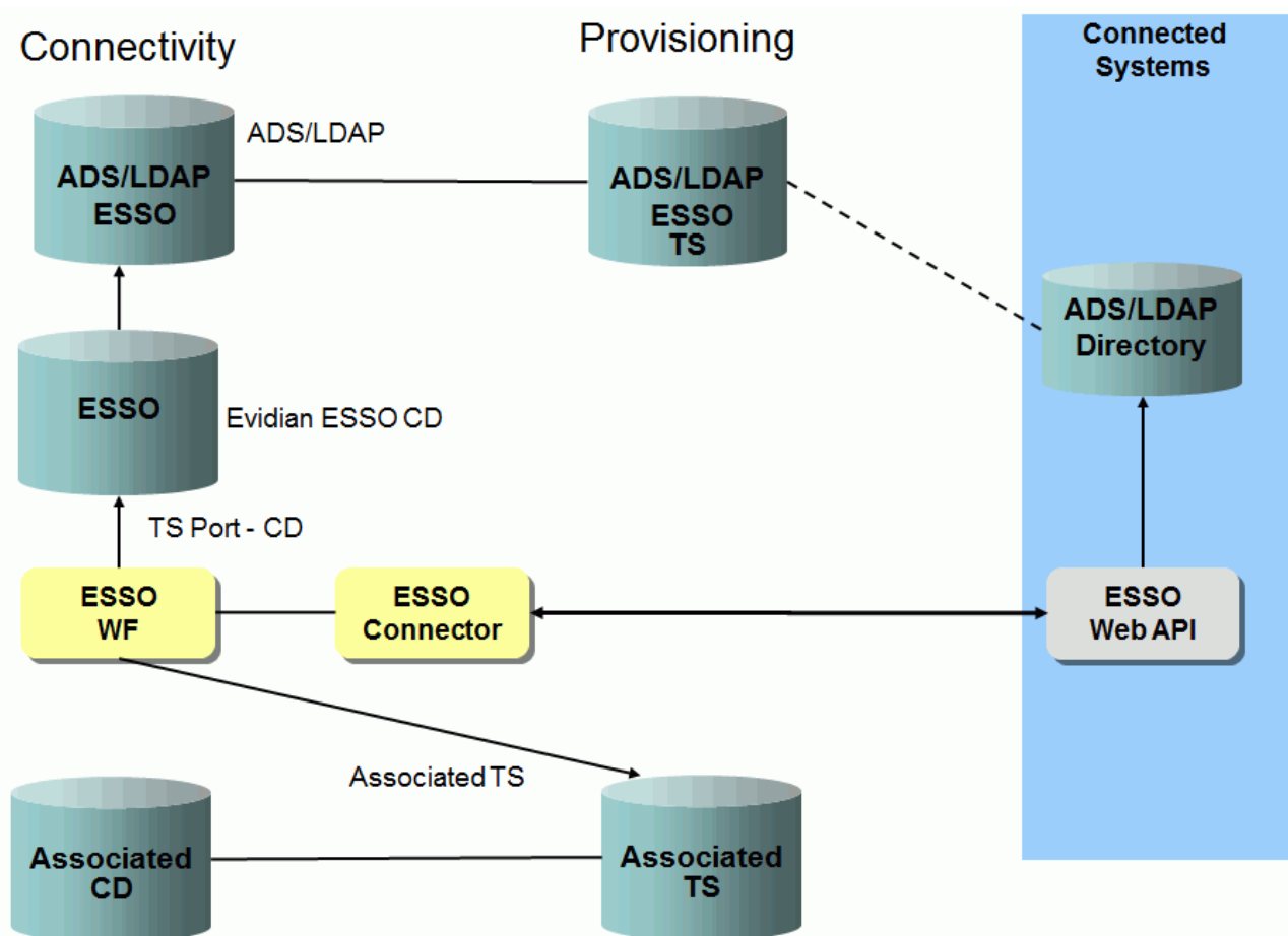
Figure 80. Evidian ESSO Provisioning Workflow Data Flow
