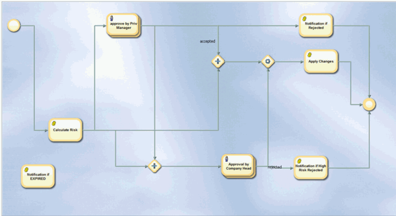
Figure 41. Risk Approval Workflow
