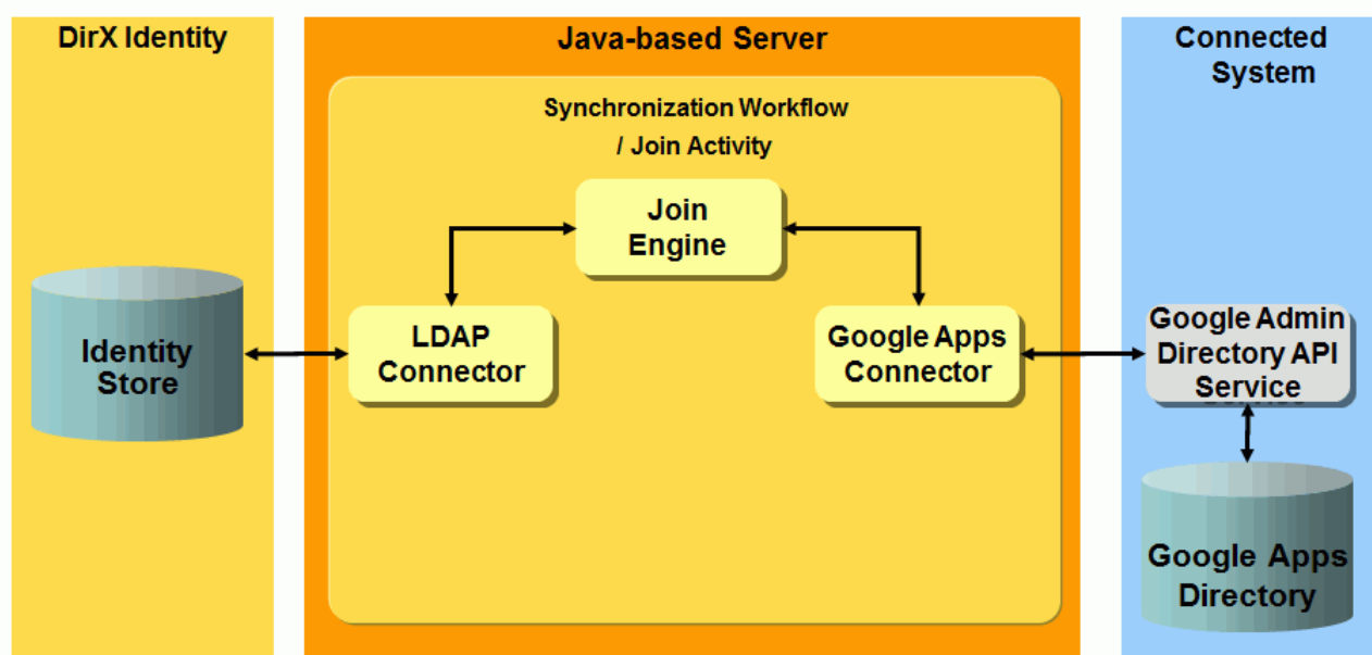
Figure 82. Google Apps Workflow Architecture
