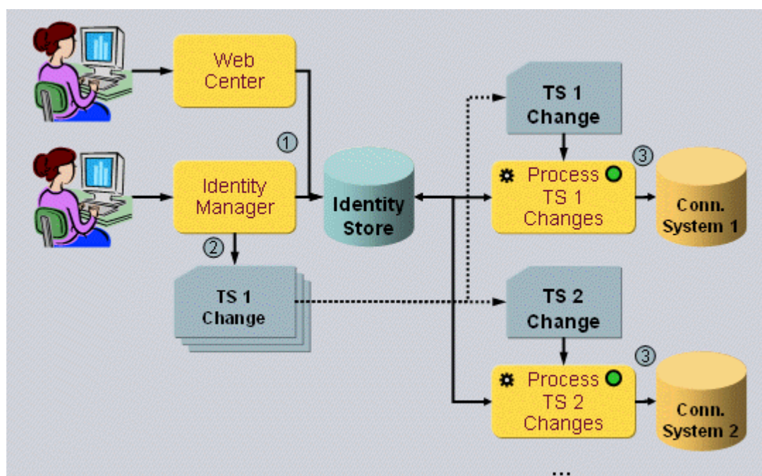
Figure 12. Password Change Workflow
