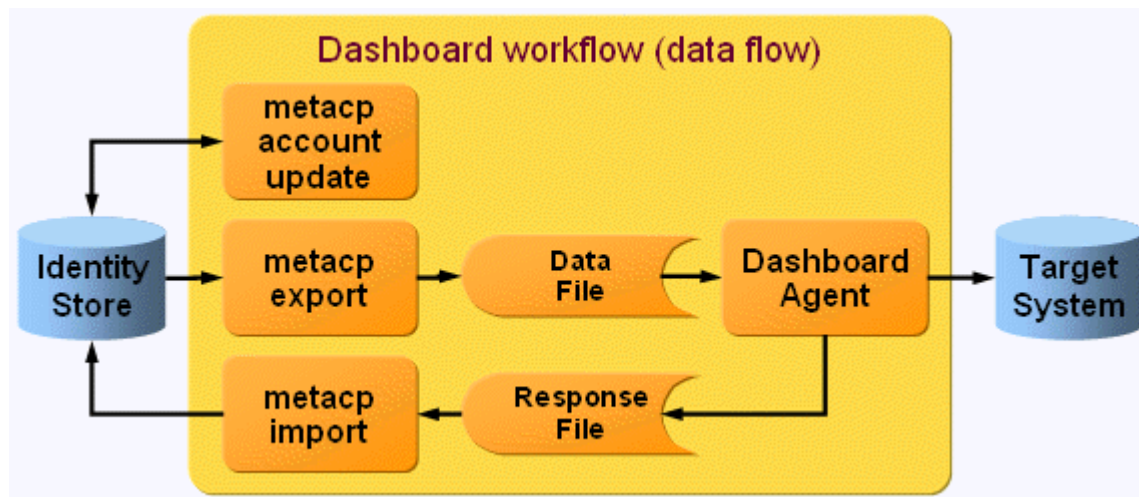
Figure 116. Dashboard Synchronization Workflow Operation
