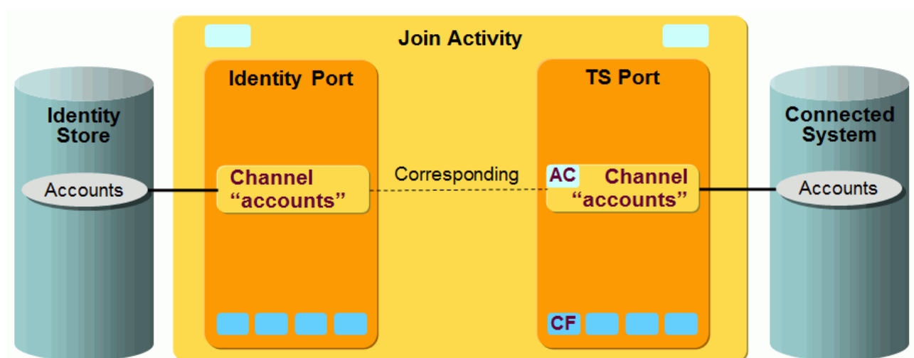
Figure 81. Evidian ESSO Provisioning Workflow Join Activity, Channels and Objects
