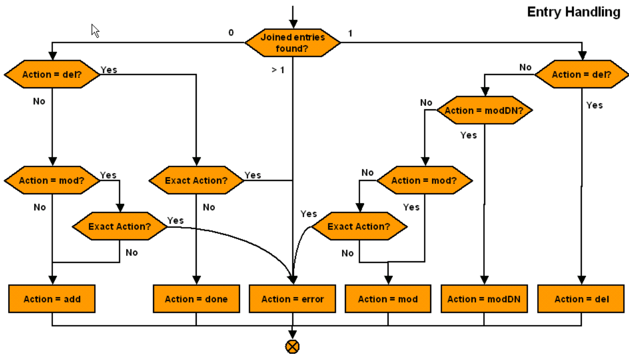
Figure 25. Profile Script - Entry Handling Logic
