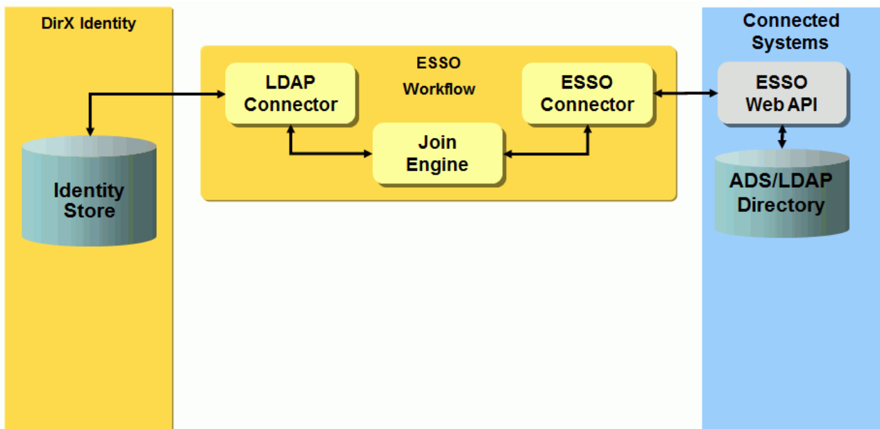
Figure 79. Evidian ESSO Provisioning Workflow Architecture
