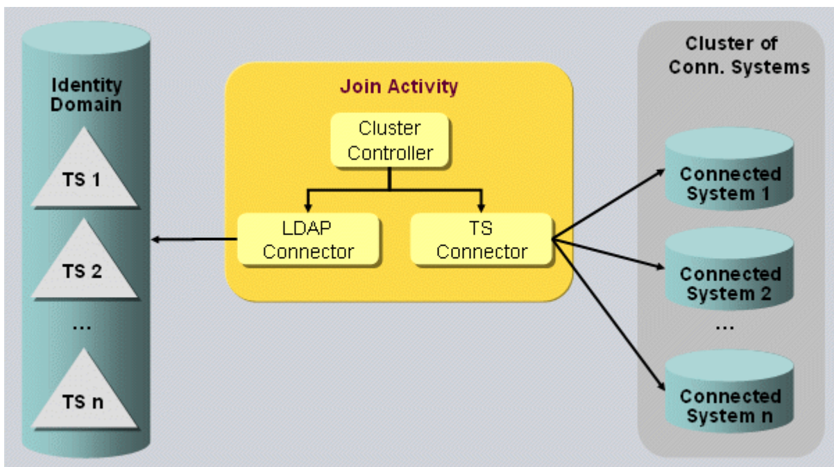
Figure 7. Cluster Workflow and Activity Structure
