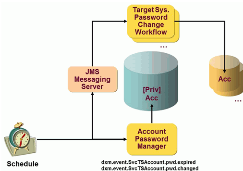
Figure 73. Account Password Management: Account Password Manager Workflow
