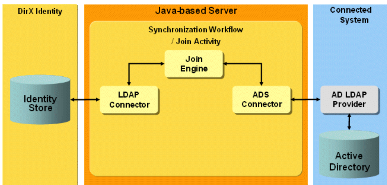
Figure 76. Active Directory Workflow Architecture
