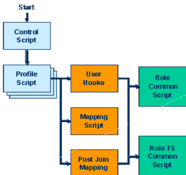
Figure 21. DirX Identity Provisioning and Connectivity Script Structure
