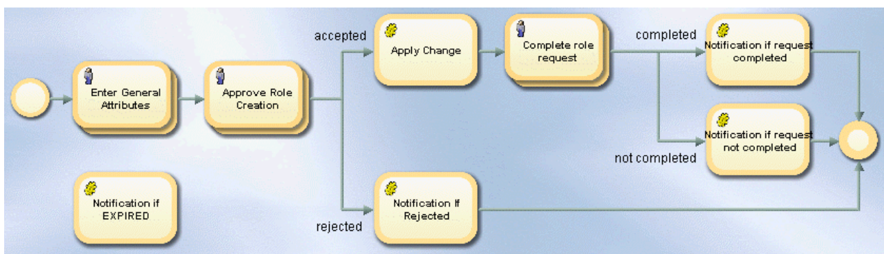
Figure 36. Example of a Create Role Workflow
