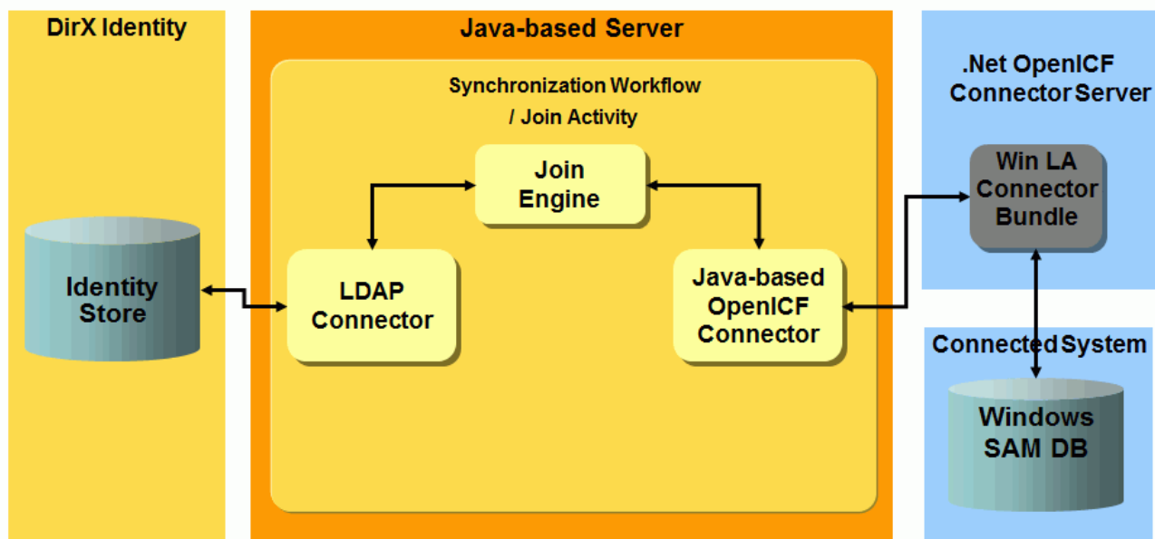
Figure 101. OpenICF Windows Local Accounts Provisioning Workflow Architecture
