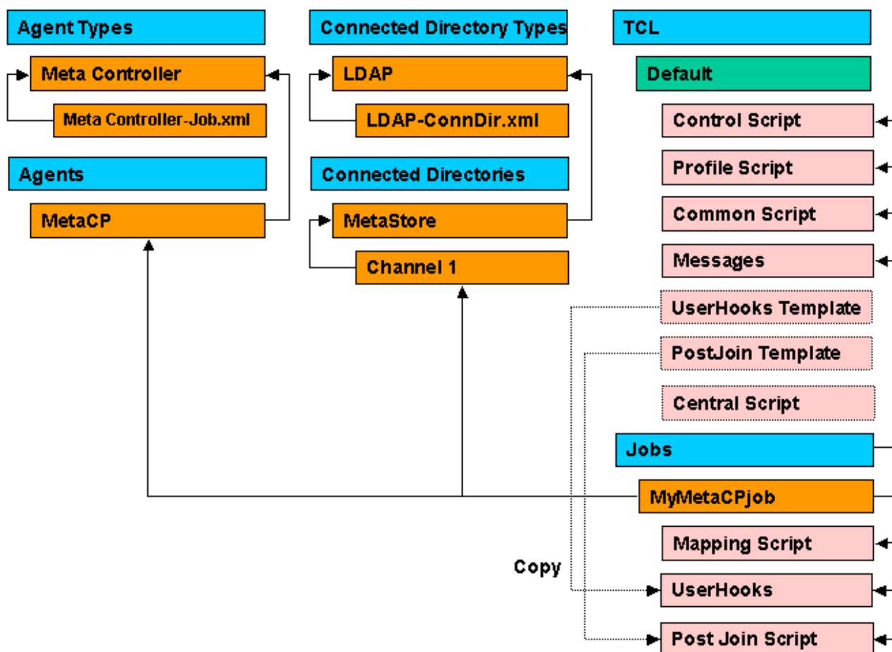
Figure 20. DirX Identity Connectivity Script Physical Structure
