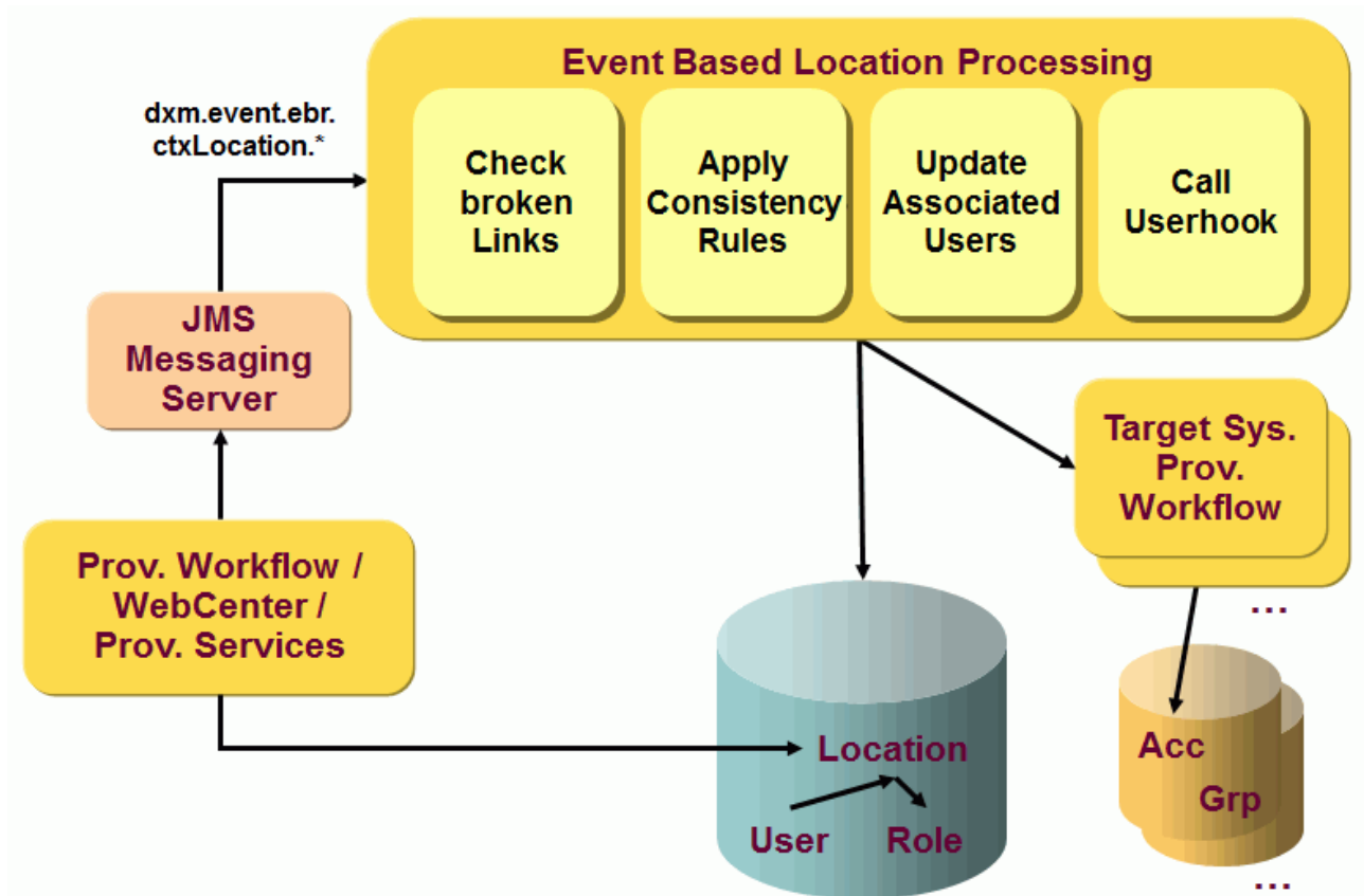
Figure 67. Event-based Maintenance Workflow Operation: Locations
