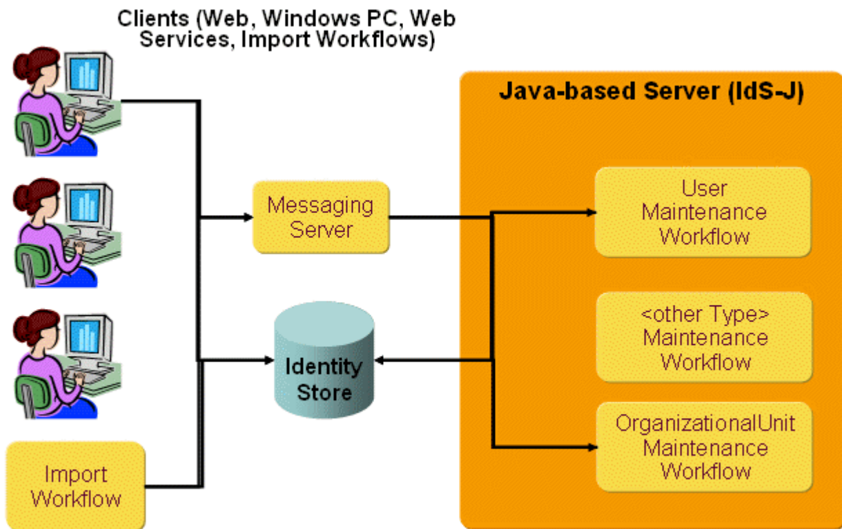
Figure 13. Event-based Maintenance Workflow
