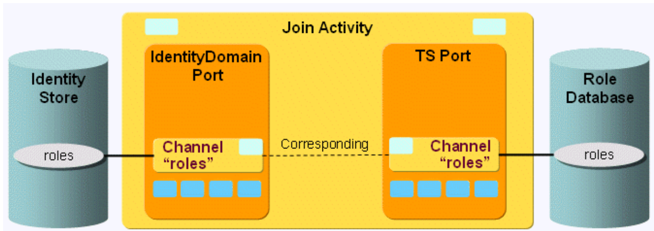
Figure 53. Role Import Workflow Ports and Channels
