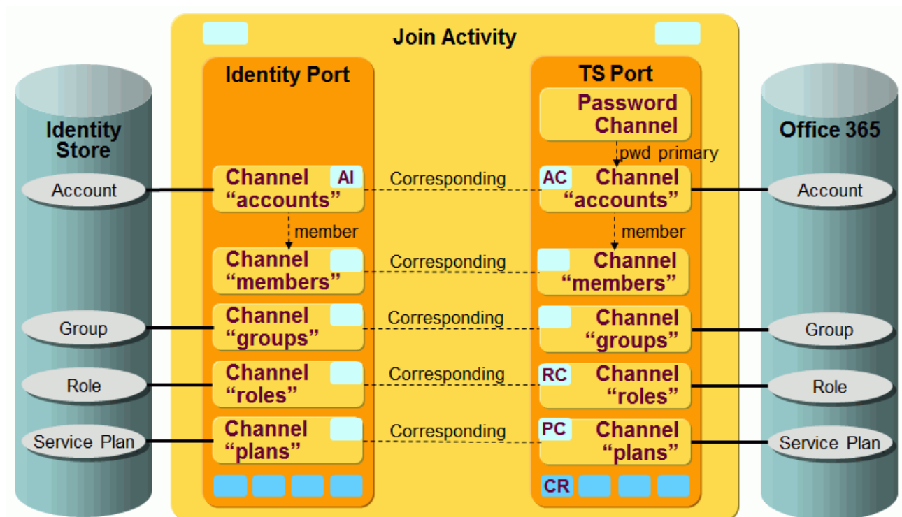
Figure 99. Microsoft 365 Provisioning Workflow Channels and Objects
