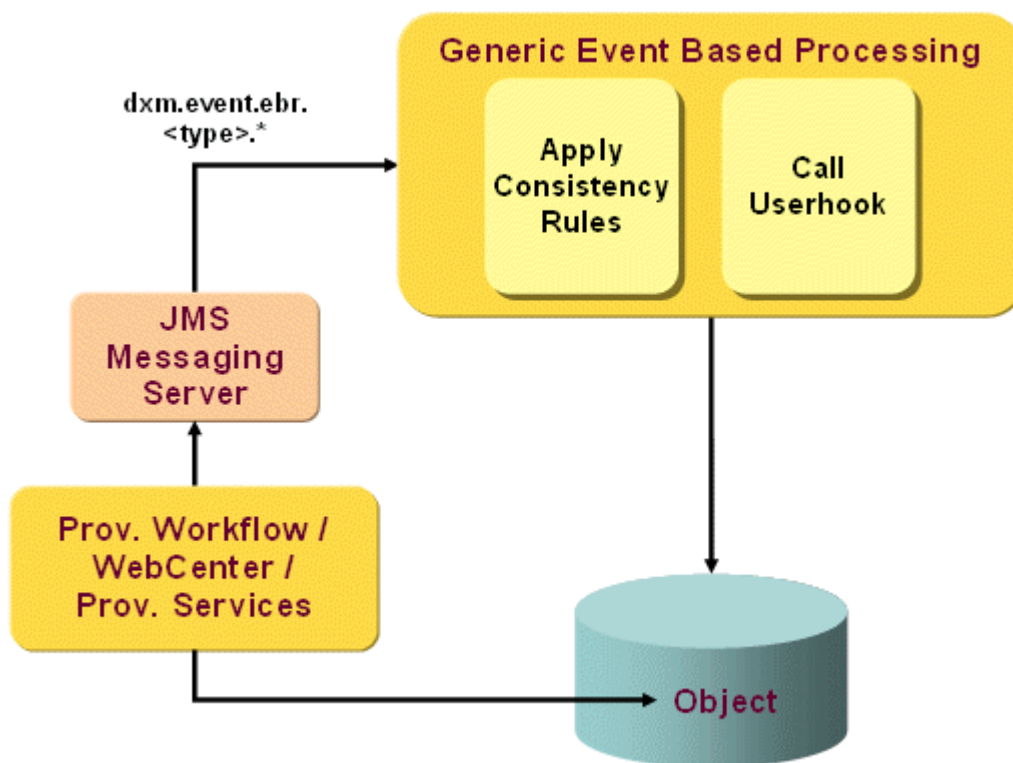
Figure 71. Generic Event-based Processing Workflow Operation
