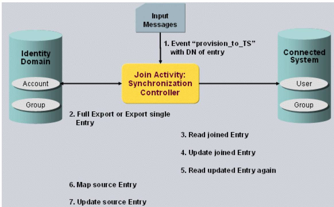
Figure 8. Sync2TS Controller Processing
