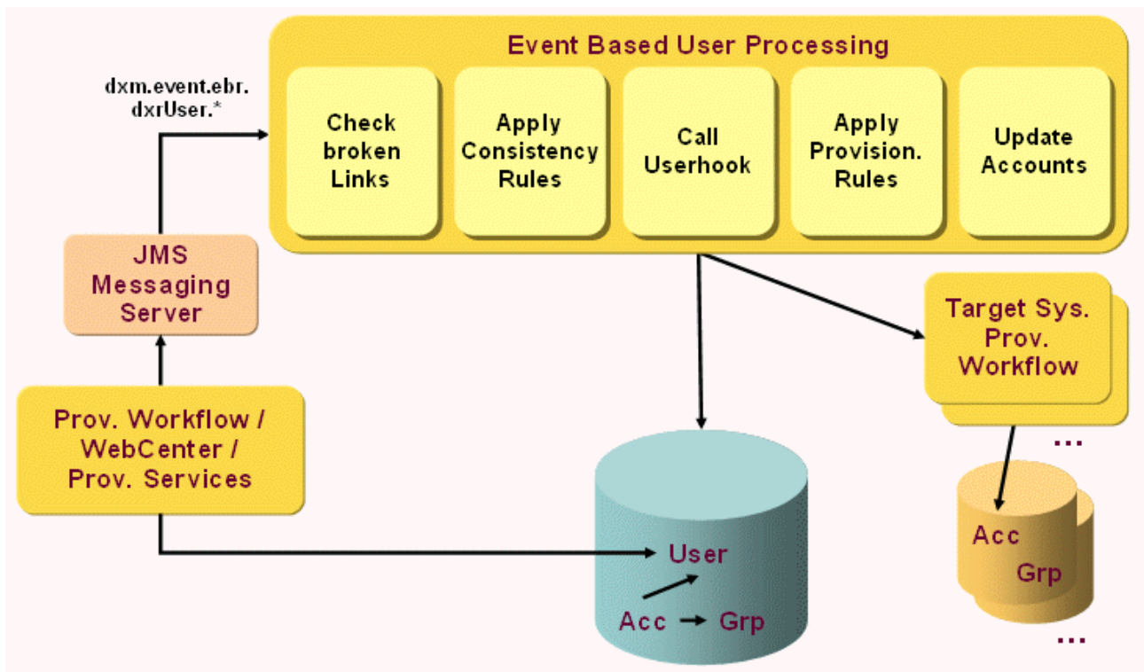
Figure 70. Event-based User Resolution Workflow Operation
