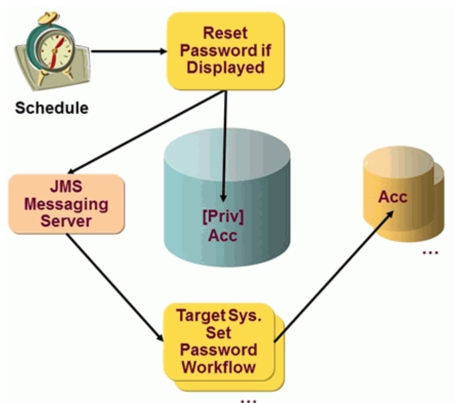
Figure 75. Account Password Management: Reset Password If Displayed Workflow
