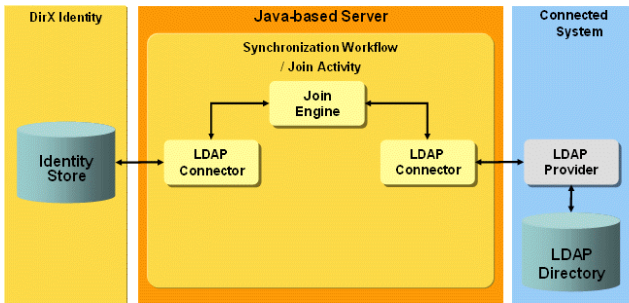
Figure 90. LDAP Workflow Architecture
