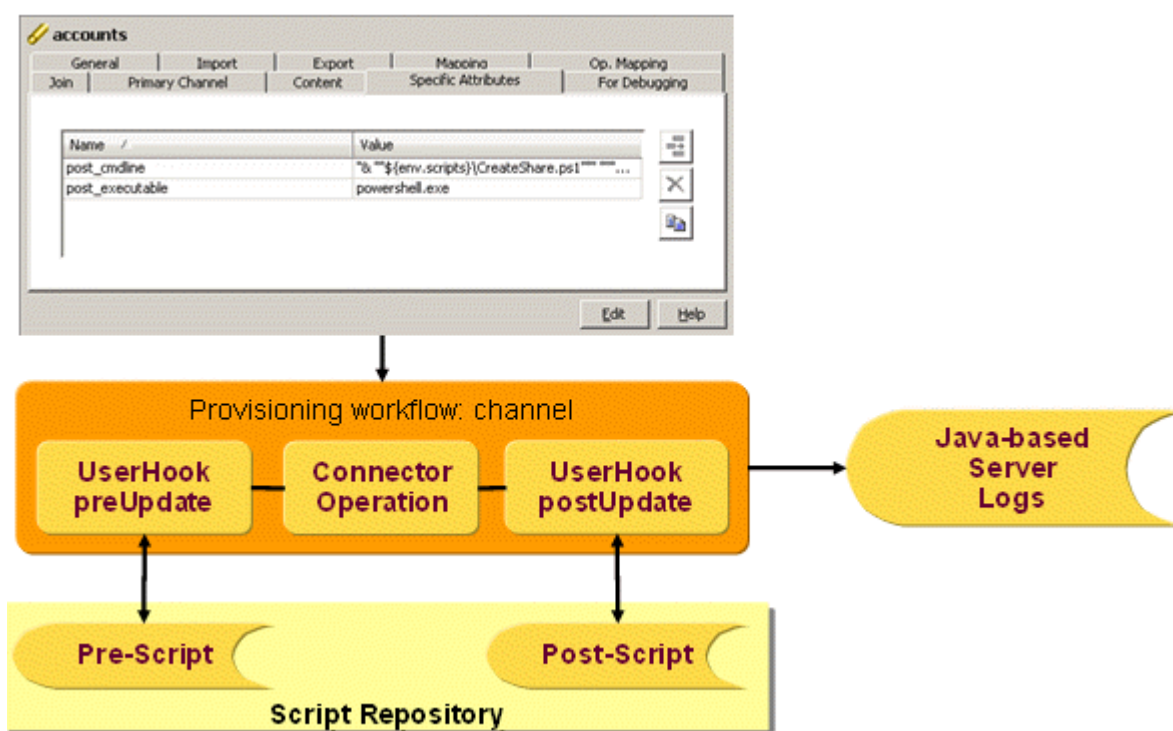
Figure 16. Running Executables from a User Hook
