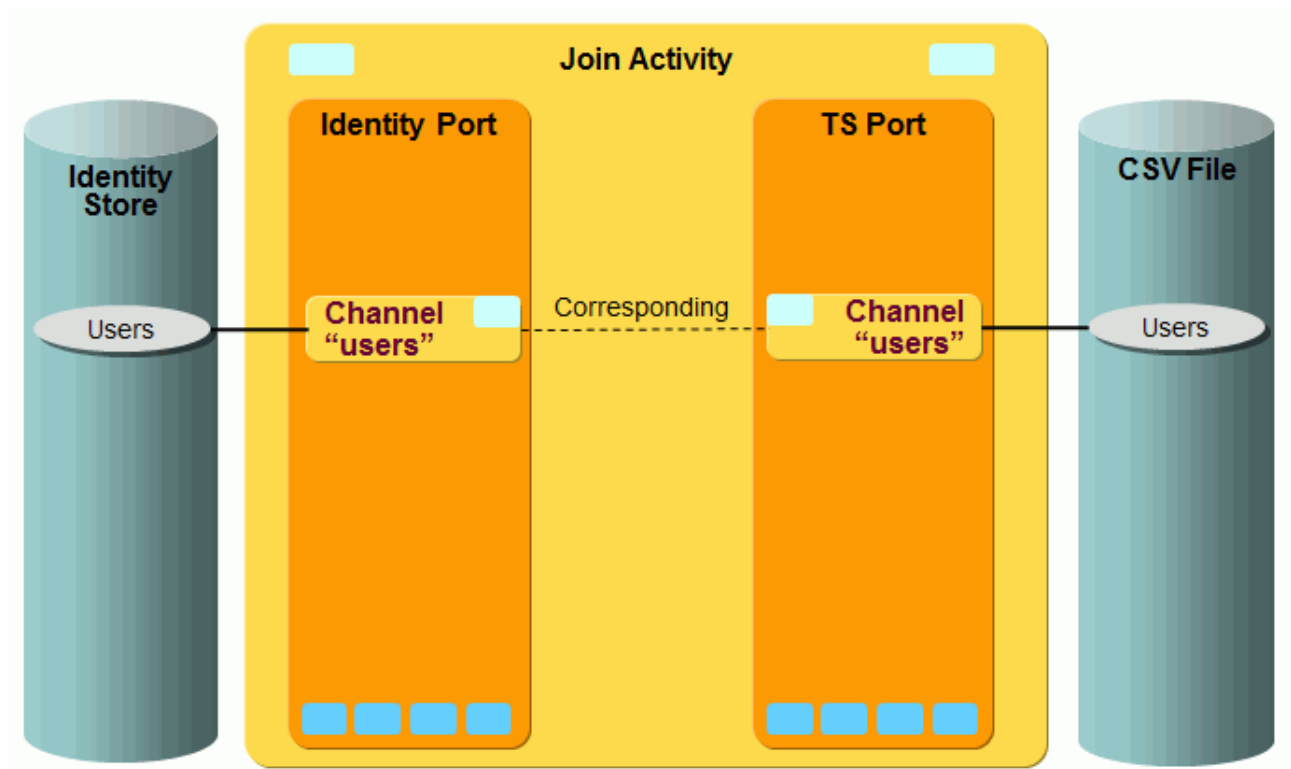
Figure 58. CSV User Export Workflows Ports and Channels
