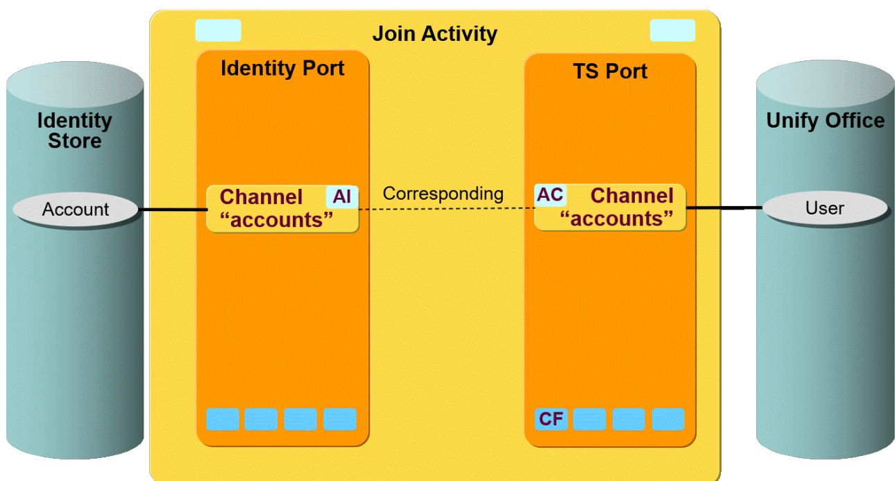
Figure 112. Unify Office Provisioning Workflow Channels and Objects
