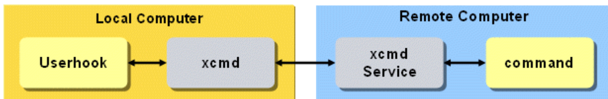
Figure 78. Remote Folder Management Architecture
