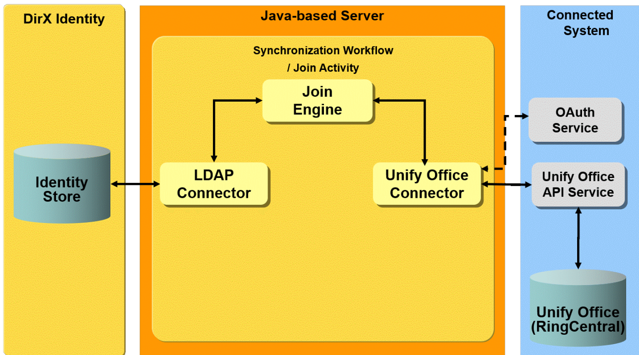
Figure 111. Unify Office Provisioning Workflow Architecture
