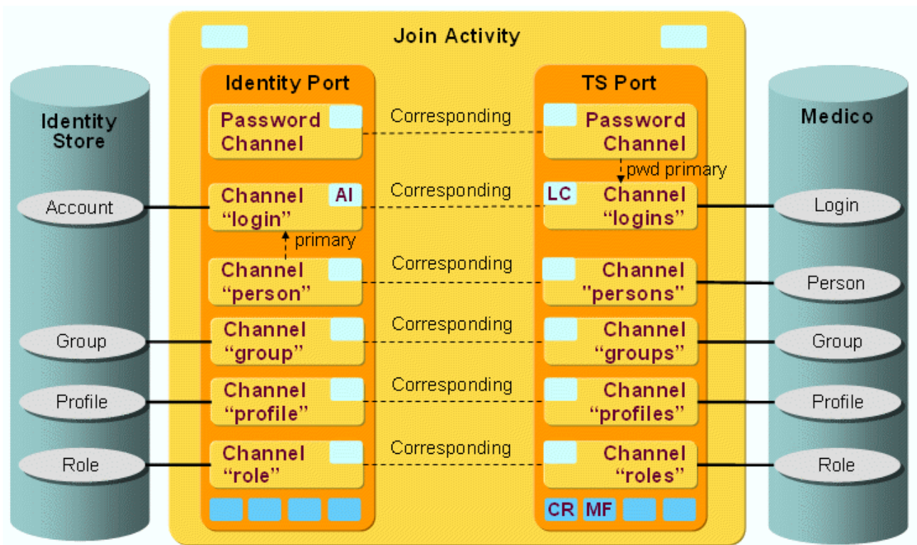
Figure 97. Medico Provisioning Workflow Channels and Objects
