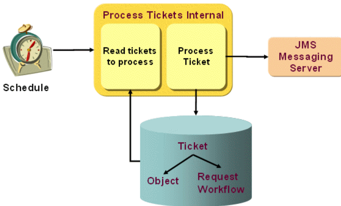
Figure 72. Process Tickets Internal Workflow
