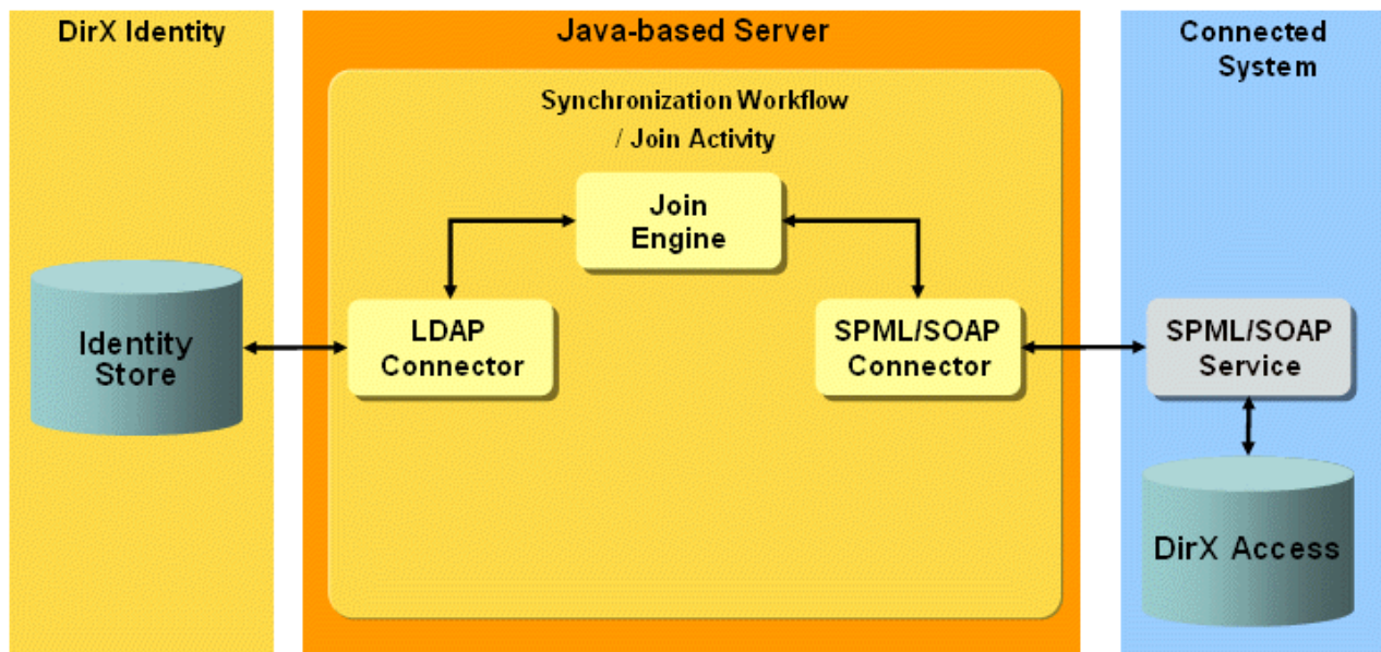
Figure 119. DirX Access Provisioning Workflow Architecture
