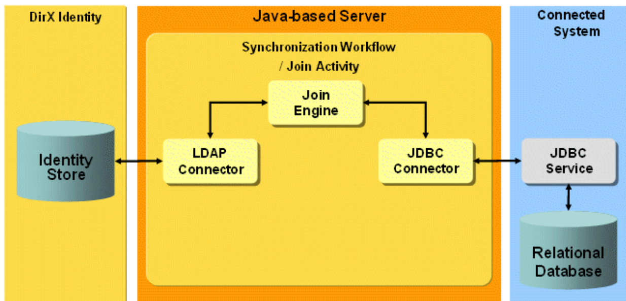
Figure 88. JDBC Provisioning Workflow Architecture
