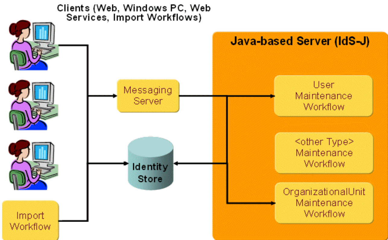
Figure 62. Invoking an Entry Maintenance Workflow
