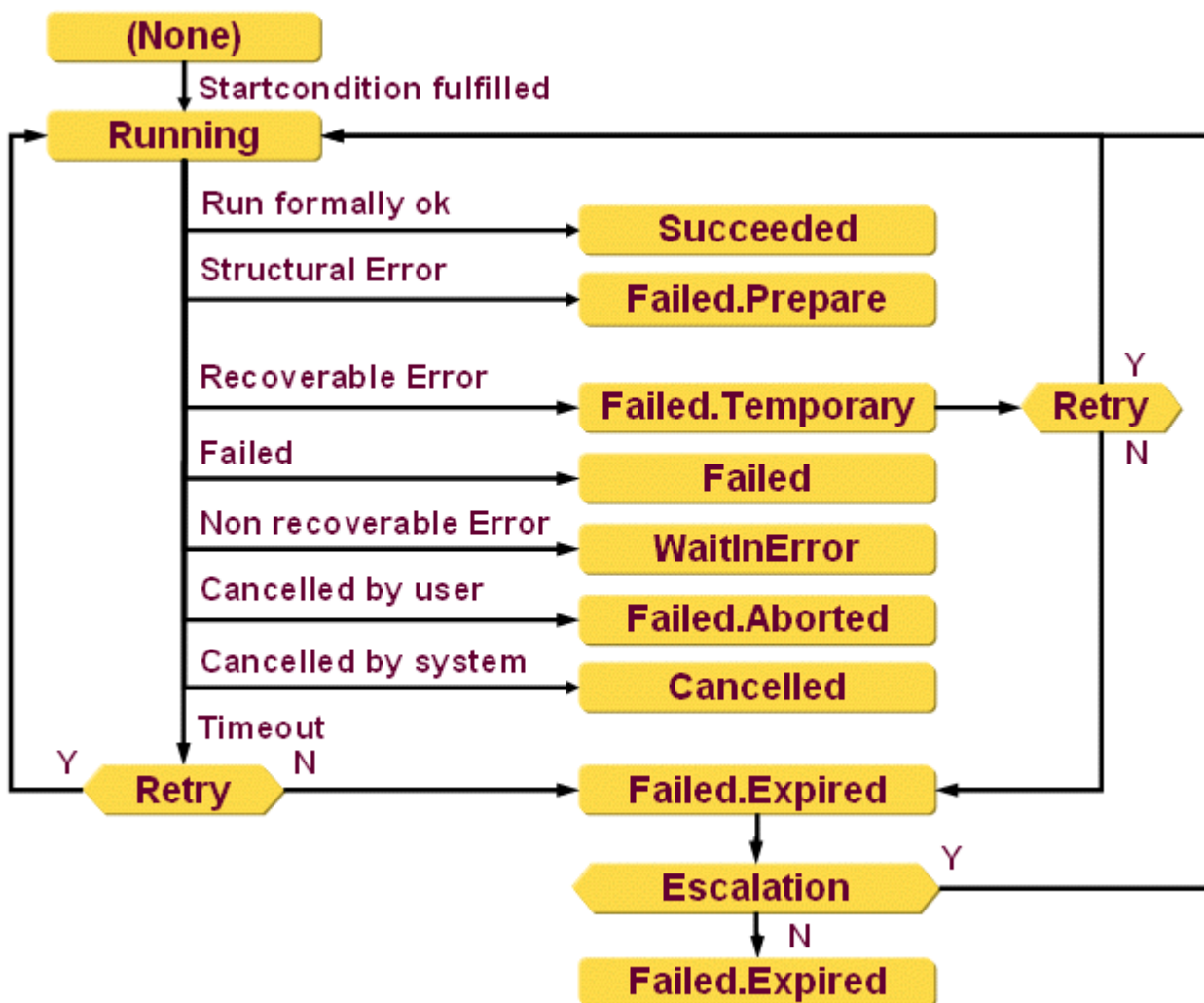
Figure 3. Request Workflow Activities
