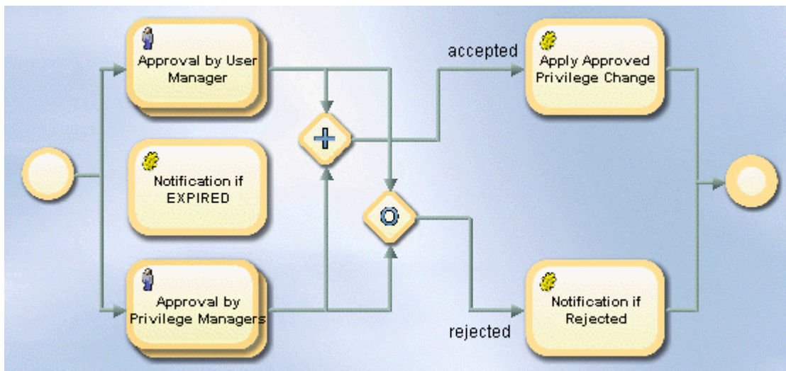
Figure 39. 4-Eye Approval Workflow
