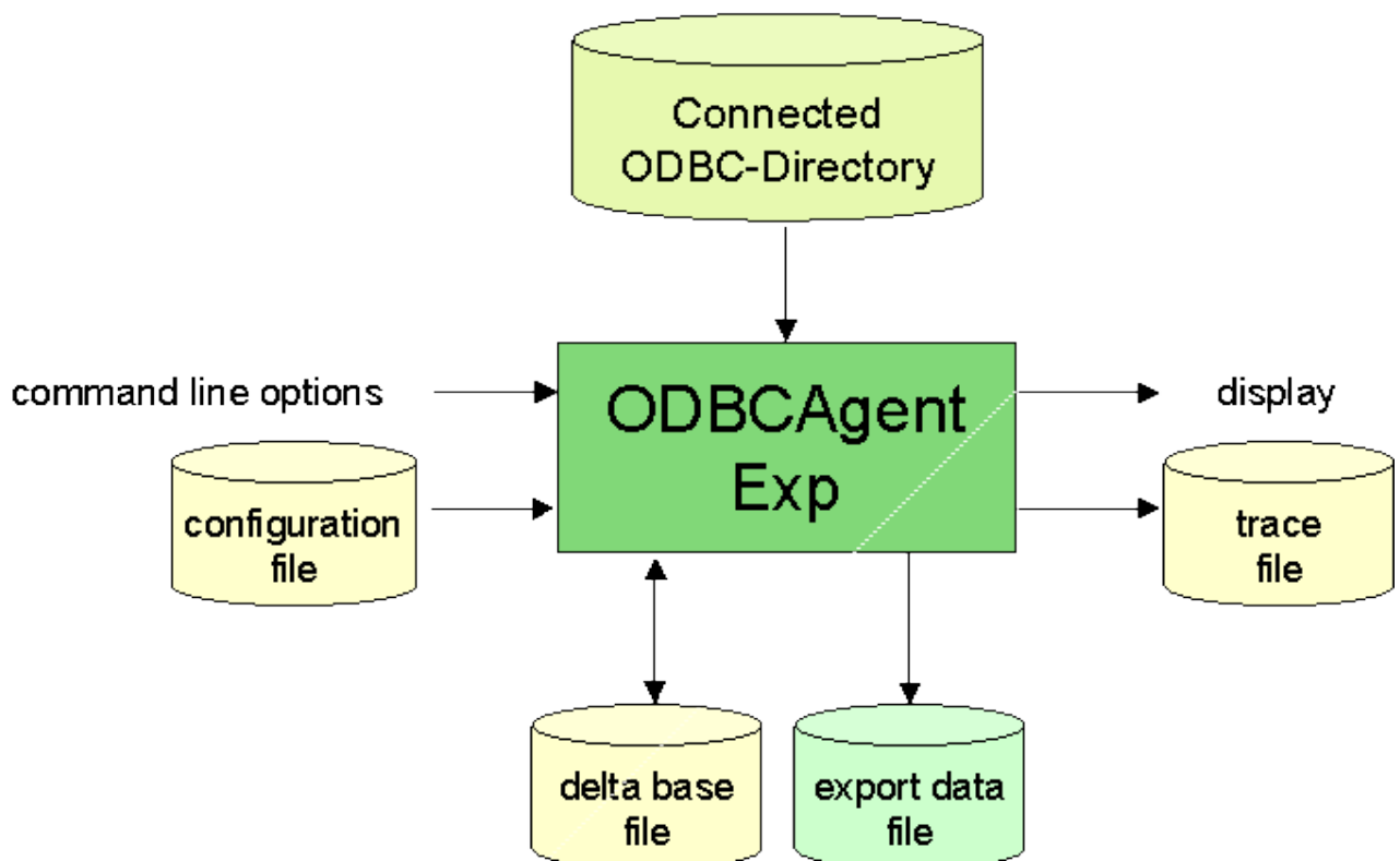
Figure 16. ODBCAgentExp Components
