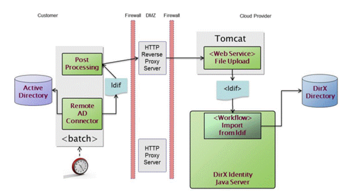
Figure 5. Remote AD Connector Architecture
