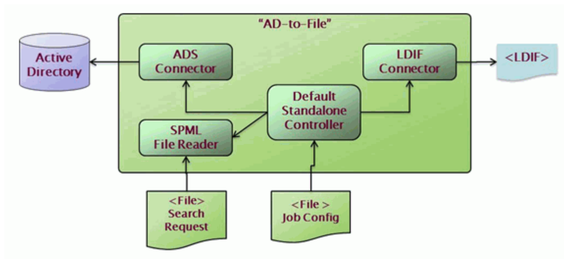
Figure 6. Export-AD-to-File Job
