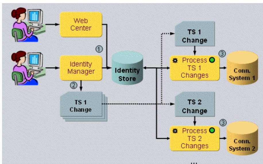
Figure 12. Password Change Workflow
