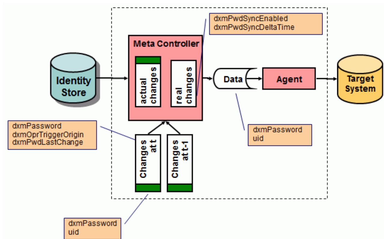
Figure 30. Workflow-Side Delta handling
