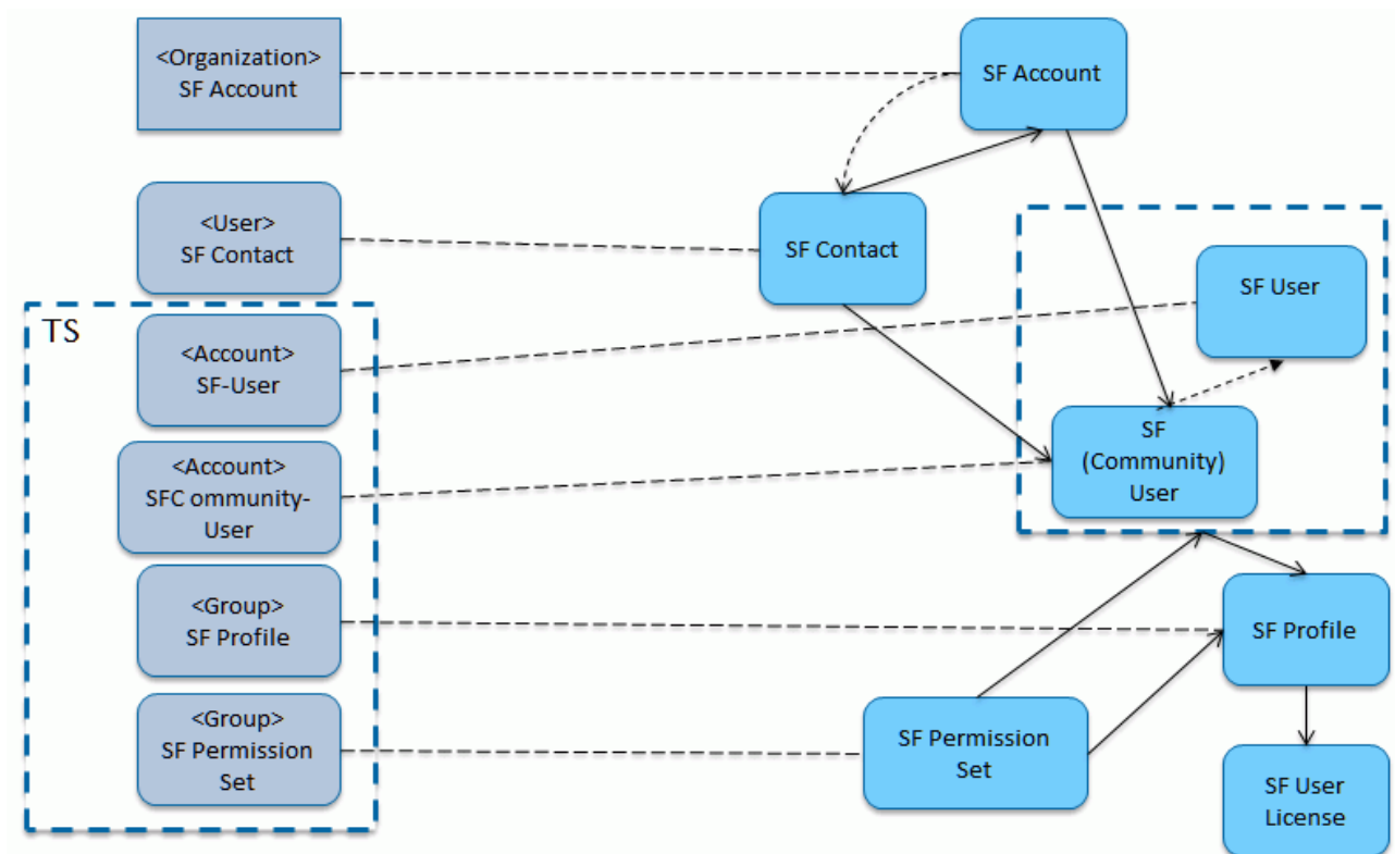
Figure 98. DirX Identity - Salesforce Object Model
