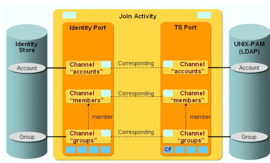
Figure 116. UNIX-PAM Provisioning Workflow Channels and Objects
