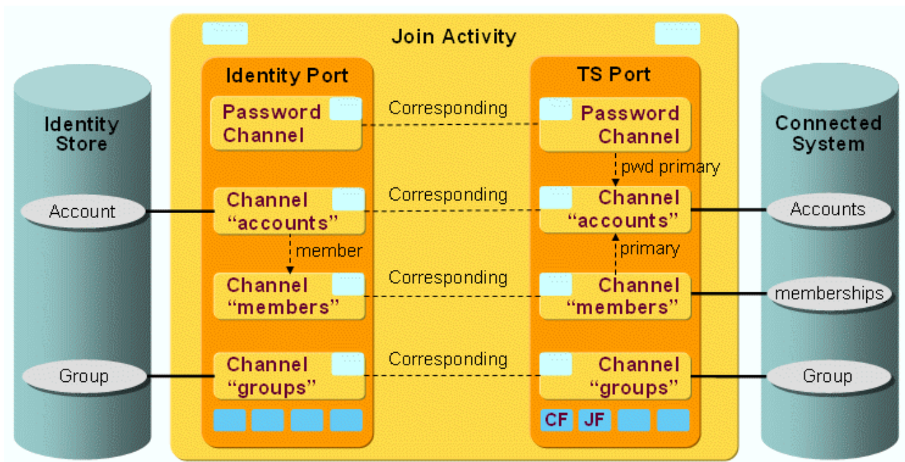
Figure 85. JDBC Provisioning Workflow Join Activity, Channels and Objects
