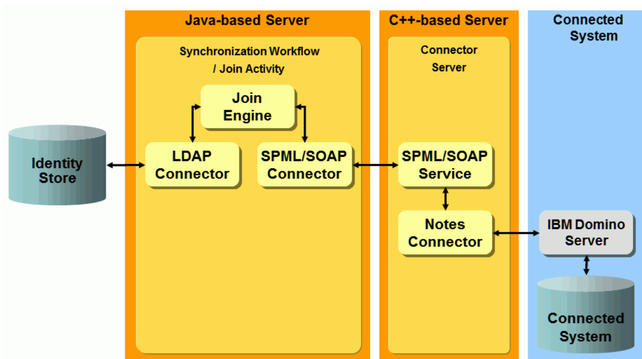
Figure 88. IBM Notes Workflows Architecture
