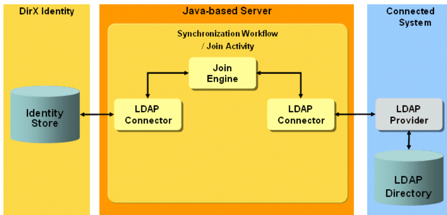
Figure 115. UNIX-PAM Workflow Architecture
