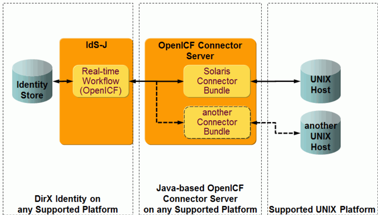
Figure 107. UNIX-OpenICF Connector Server Architecture
