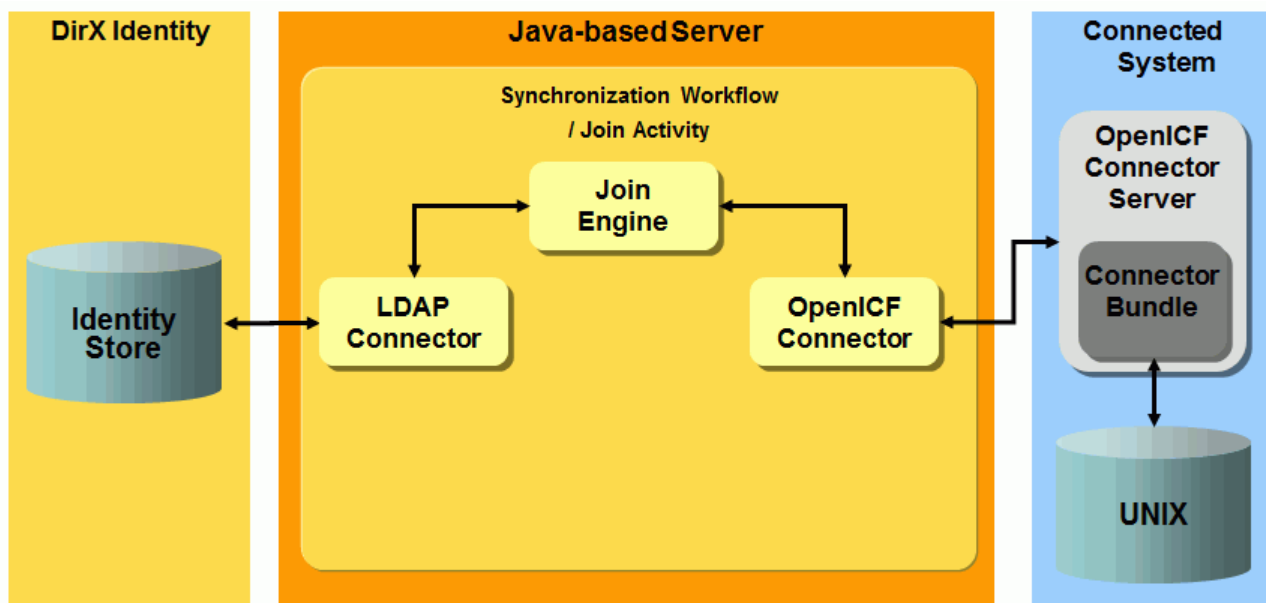
Figure 108. UNIX-OpenICF Provisioning Workflow Architecture
