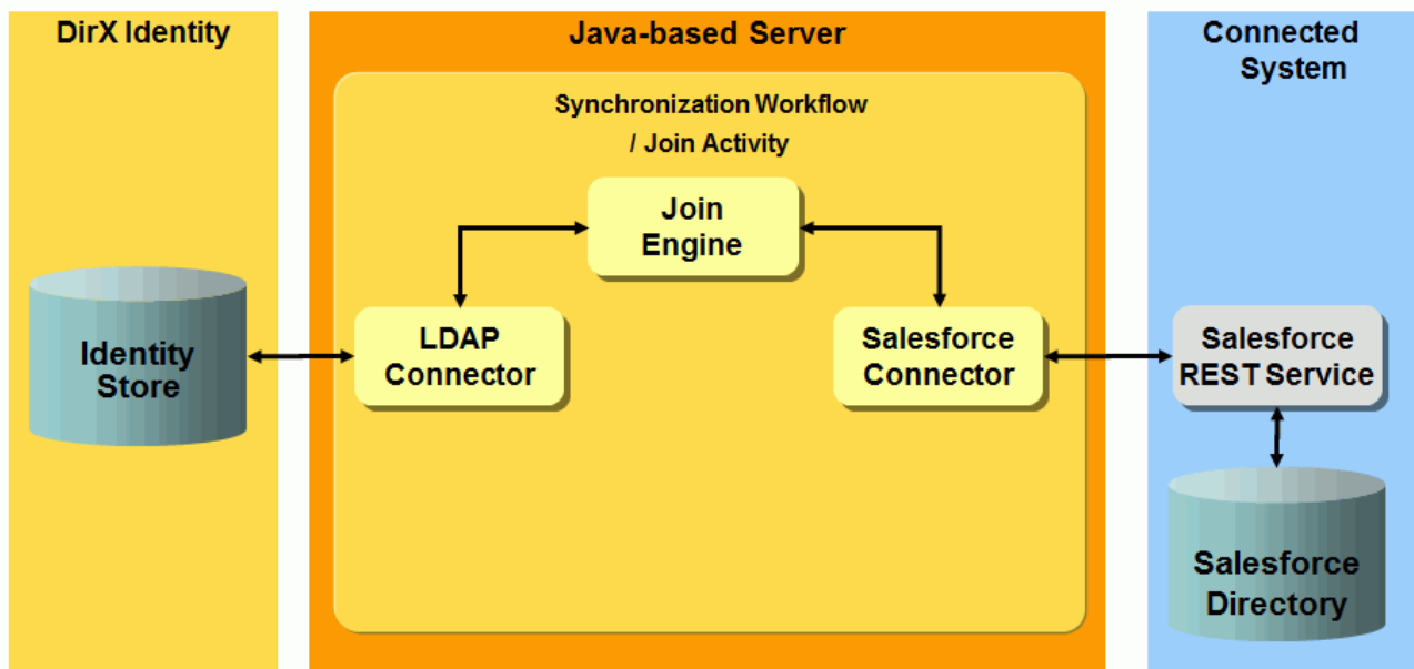
Figure 99. Salesforce Provisioning Workflow Architecture
