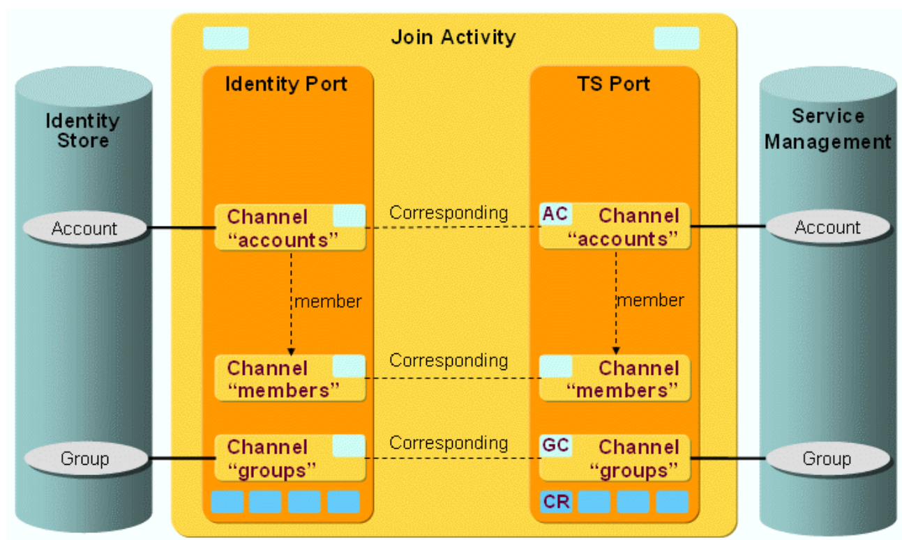
Figure 102. Service Management Channels and Object Types
