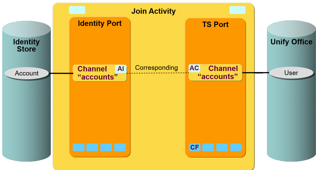
Figure 106. Unify Office Provisioning Workflow Channels and Objects
