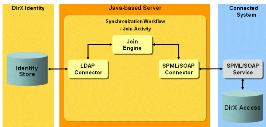
Figure 113. DirX Access Provisioning Workflow Architecture
