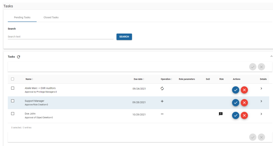
Figure 21. My Tasks
