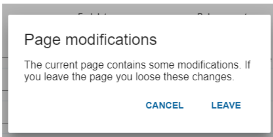
Figure 35. Warning Dialog
