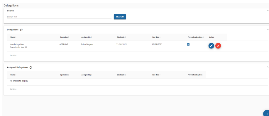
Figure 44. My Delegations
