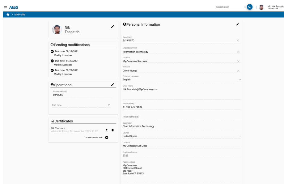
Figure 16. My Profile
