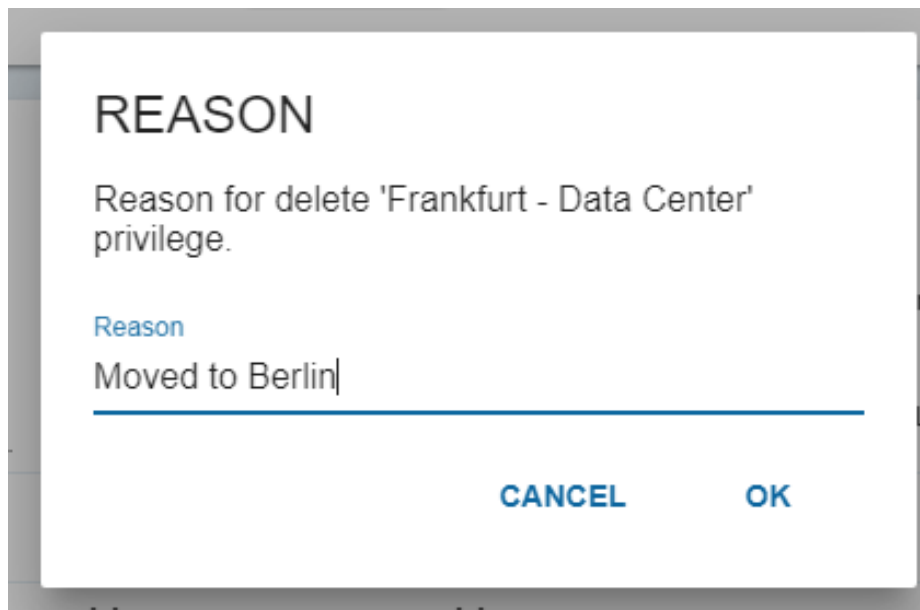
Figure 29. Reason Dialog
