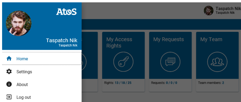
Figure 11. Navigation Menu
