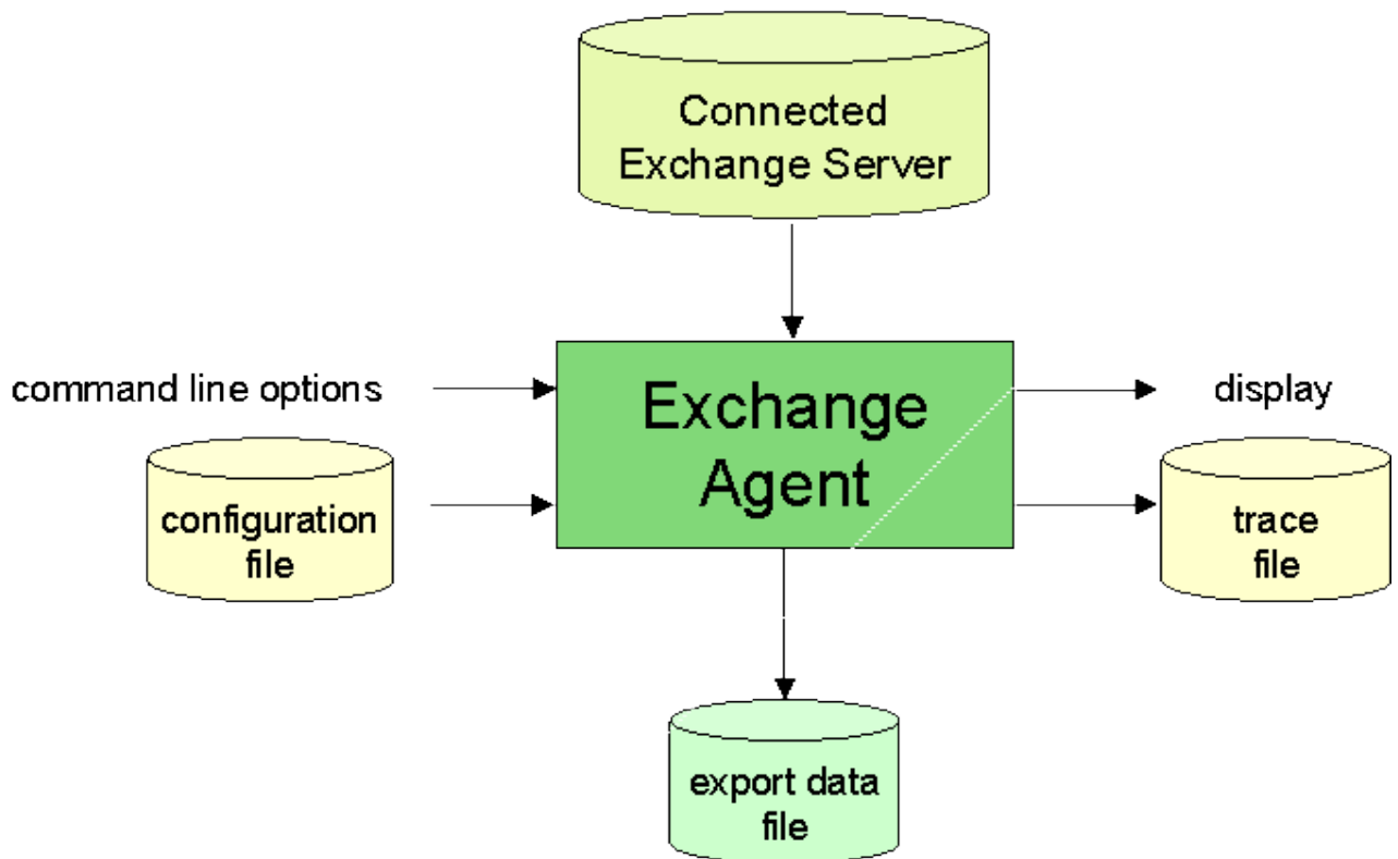
Figure 10. ExchangeAgent Export Components
