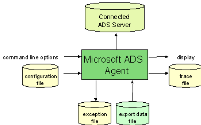
Figure 8. ADSAgent Export Components
