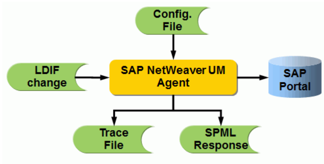
Figure 24. SAP NetWeaver UM Agent Export Components
