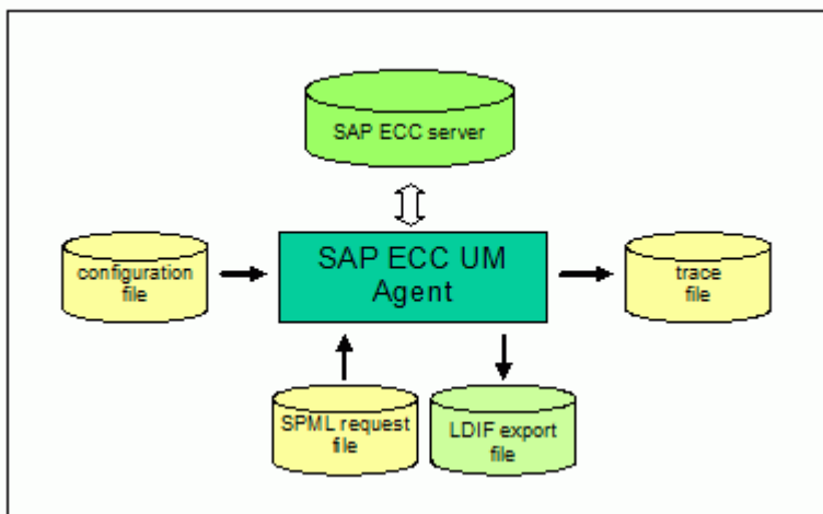
Figure 22. SAP-ECC-UM-Agent Export Components
