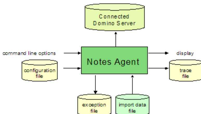
Figure 7. NotesAgent Import Components
