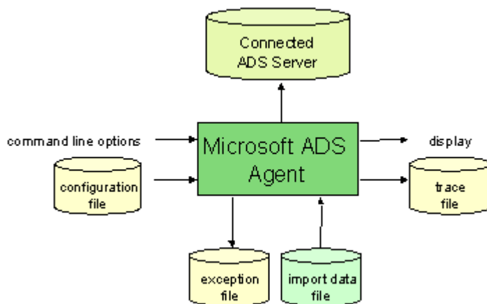
Figure 9. ADSAgent Import Components
