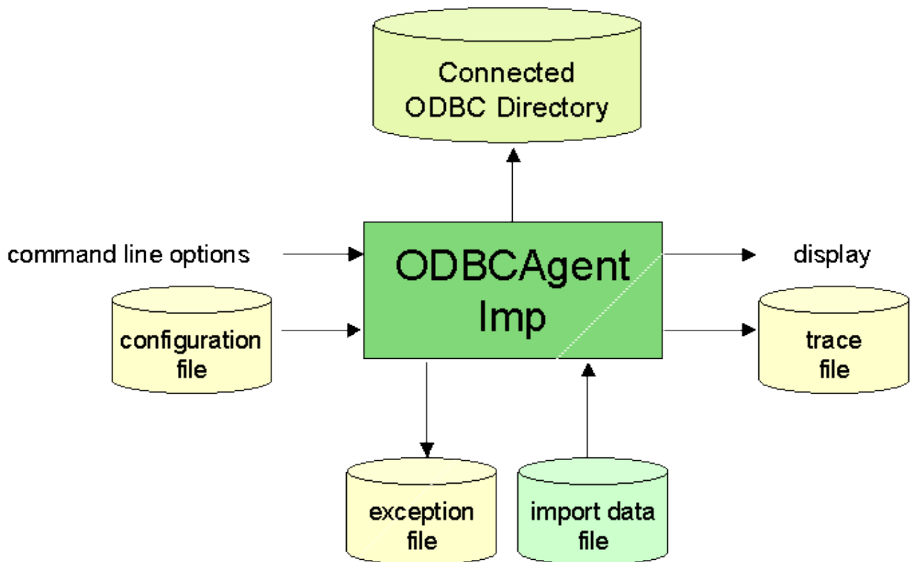
Figure 12. ODBCAgentImp Components
