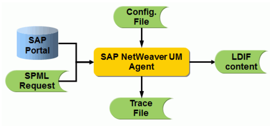
Figure 25. SAP NetWeaver UM Agent Import Components
