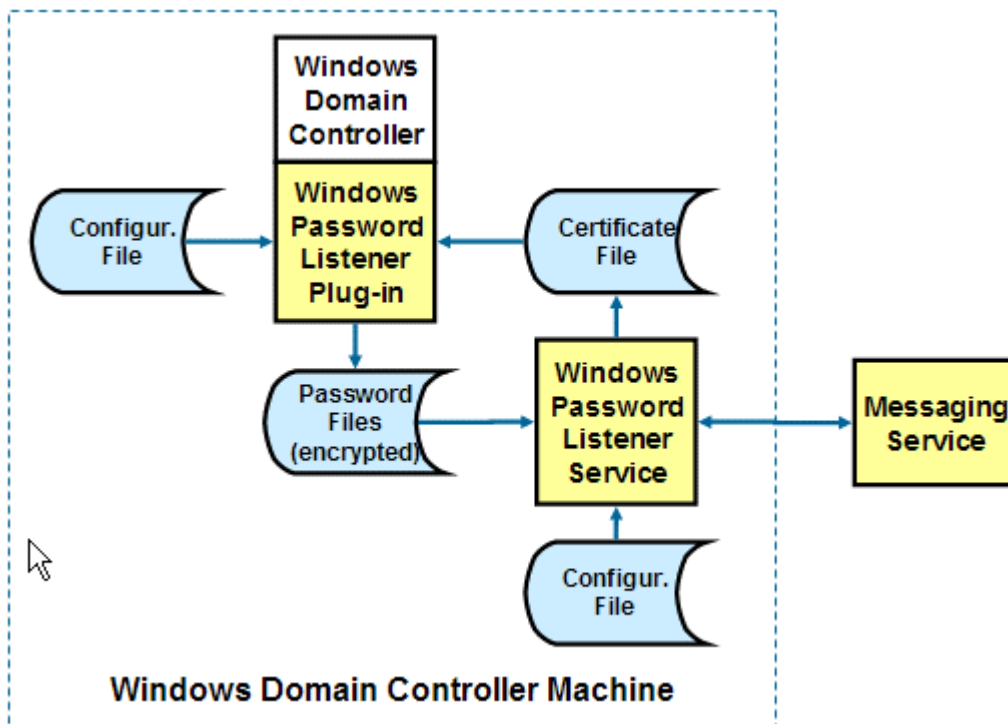
Figure 28. Windows Password Listener Architecture
