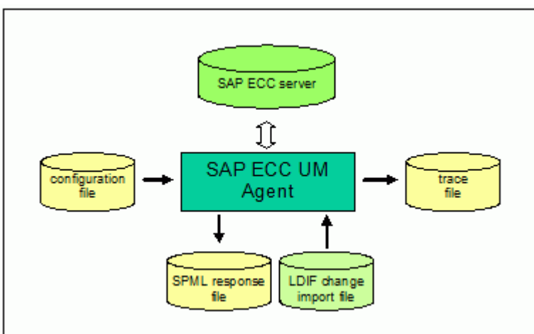
Figure 23. SAP-ECC-UM-Agent Import Components
