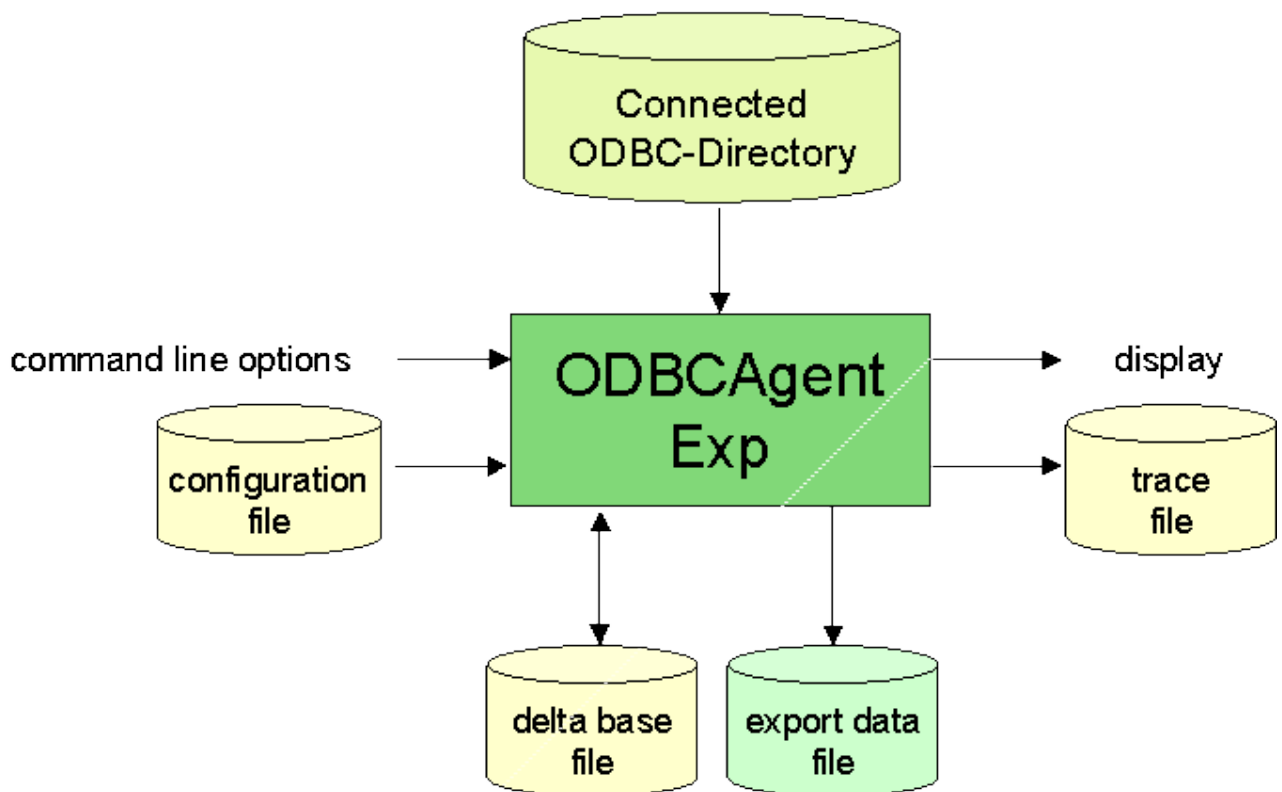
Figure 13. ODBCAgentExp Components
