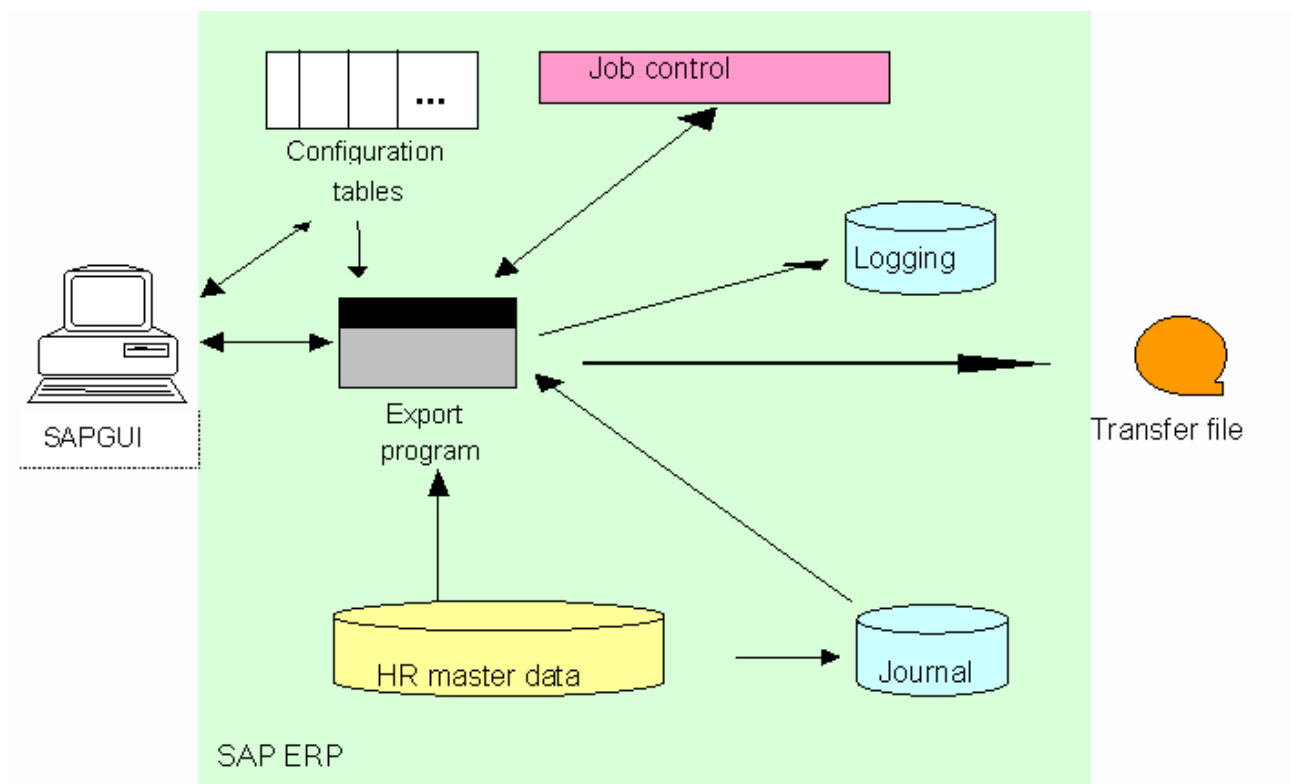
Figure 14. SAPAgent Components
