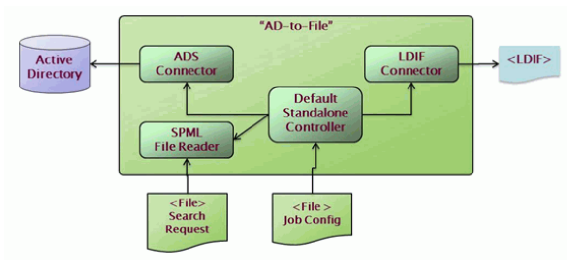
Figure 3. Export-AD-to-File Job
