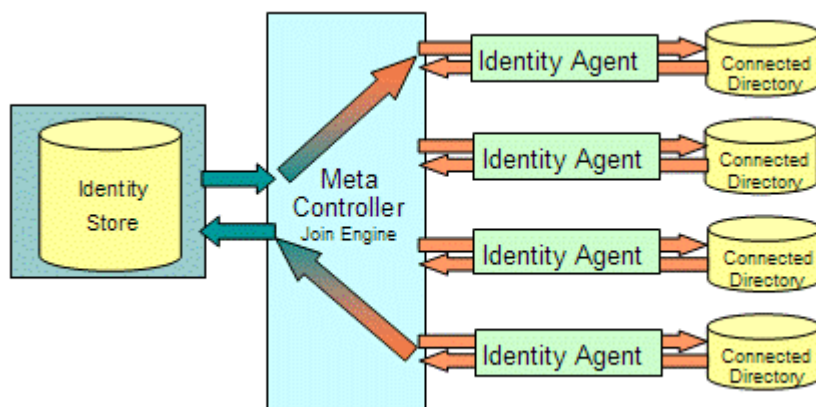
Figure 4. Meta Controller and Agent Control Flow
