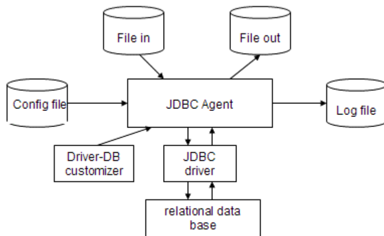
Figure 5. JDBC Agent Components
