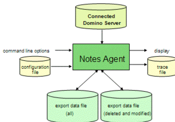
Figure 6. NotesAgent Export Components
