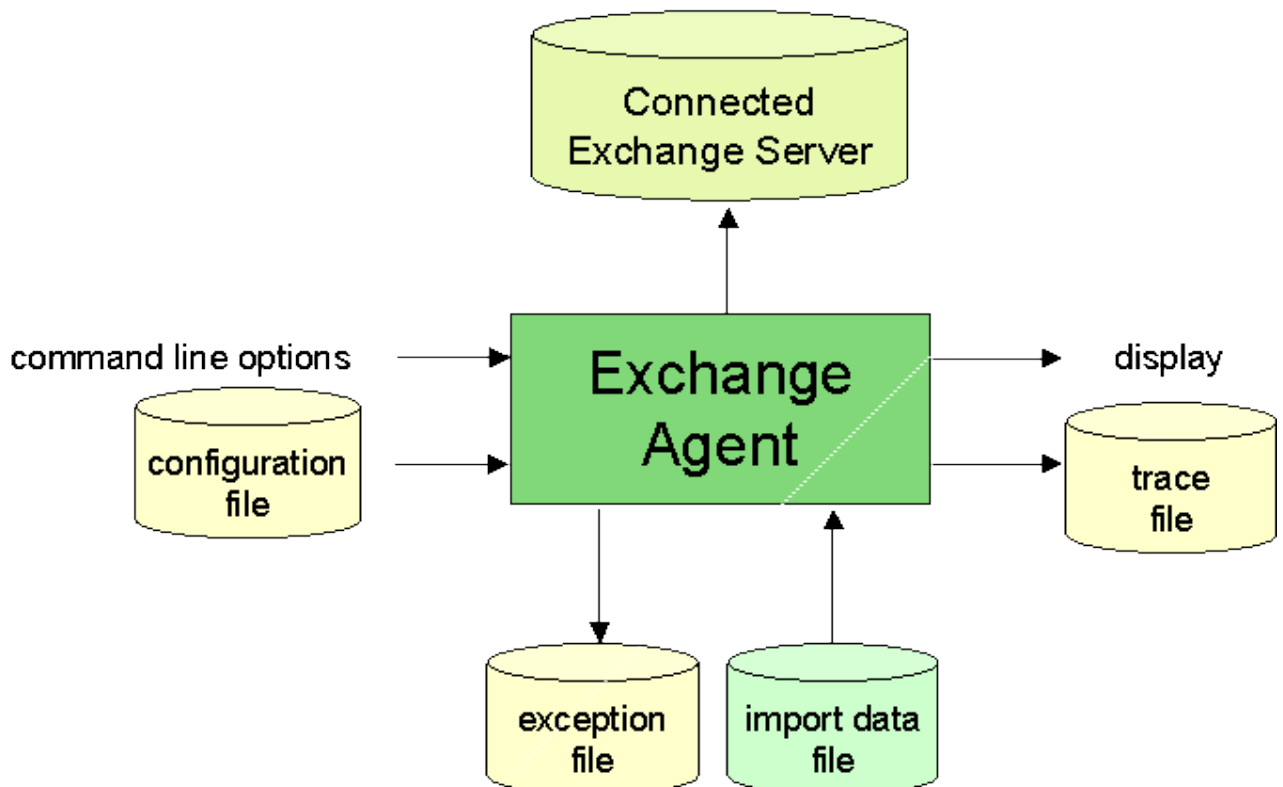
Figure 11. ExchangeAgent Import Components
