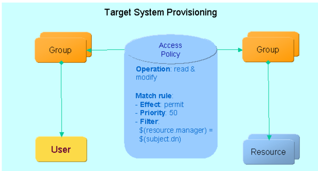
Figure 44. Access Policy with Match Rules
