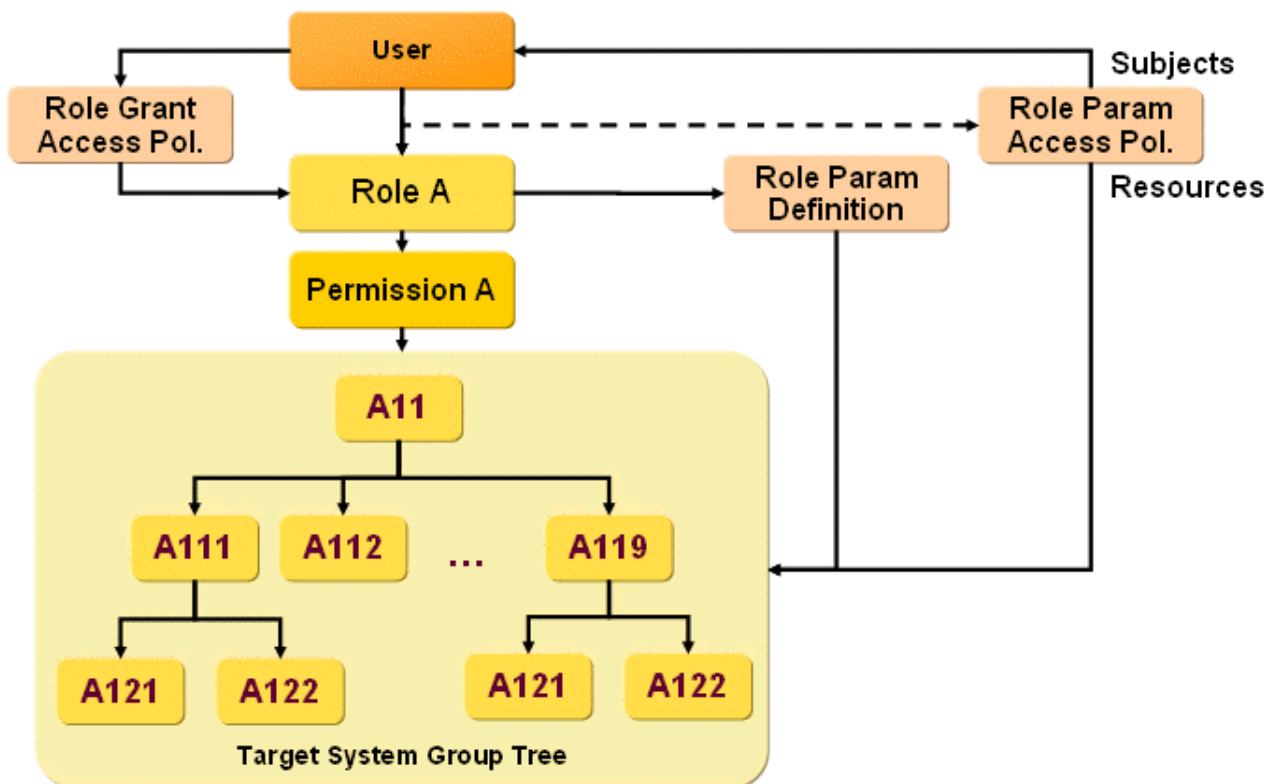
Figure 40. Hierarchical Parameter Object Relationships Example
