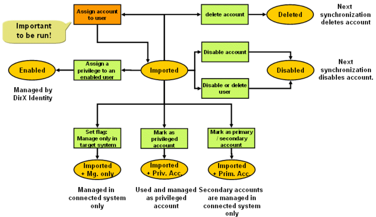
Figure 50. Alternatives for Handling Imported Accounts
