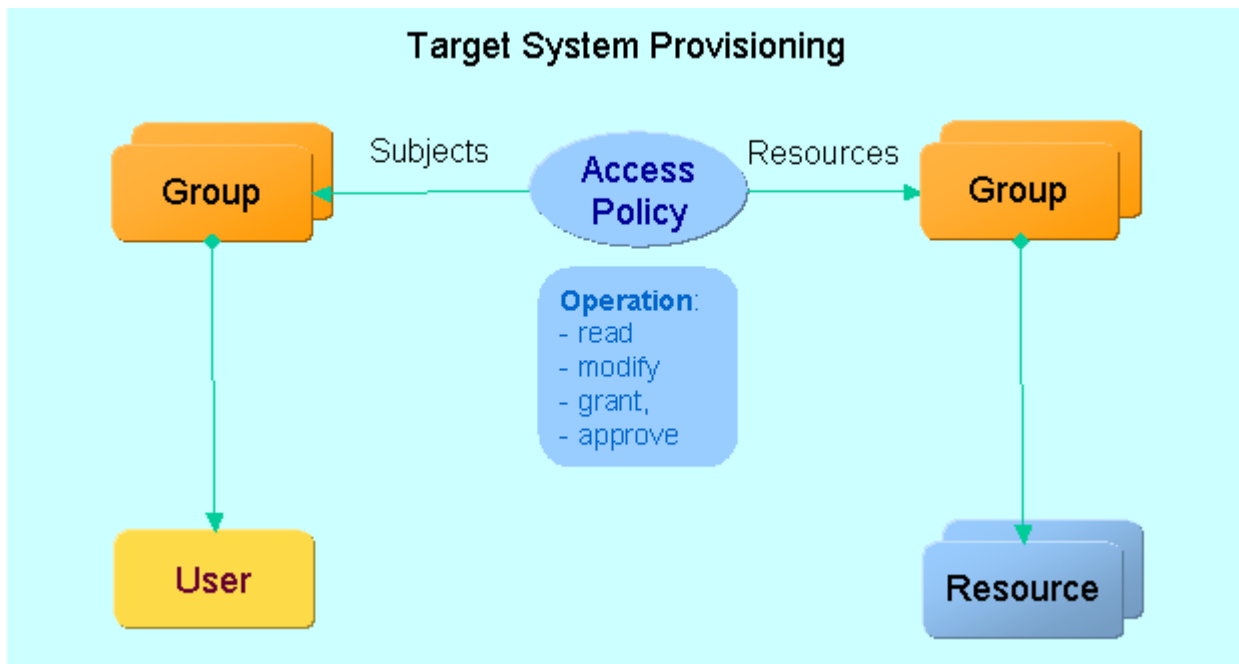
Figure 43. DirX Identity Provisioning Access Policy Structure
