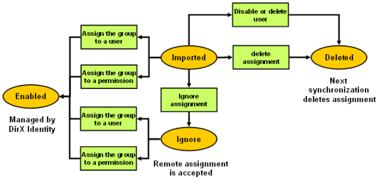
Figure 56. Alternatives for Handling Imported Group Memberships
