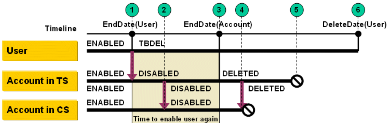
Figure 14. Relationship between User and Account Lifecycles
