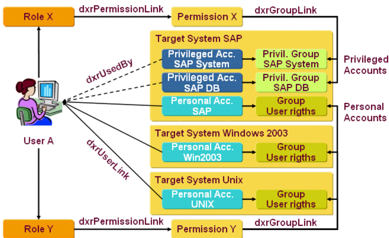
Figure 54. Personal and Privileged Accounts
