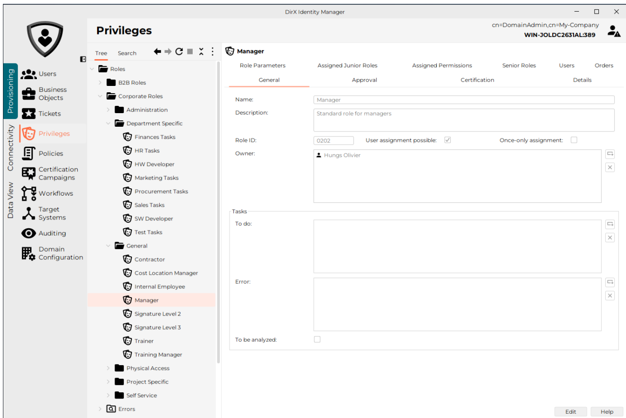
Figure 26. Viewing the Privilege Structure with DirX Identity Manager
