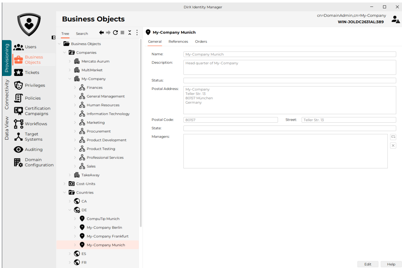
Figure 20. Viewing the Business Object Structure with DirX Identity Manager
