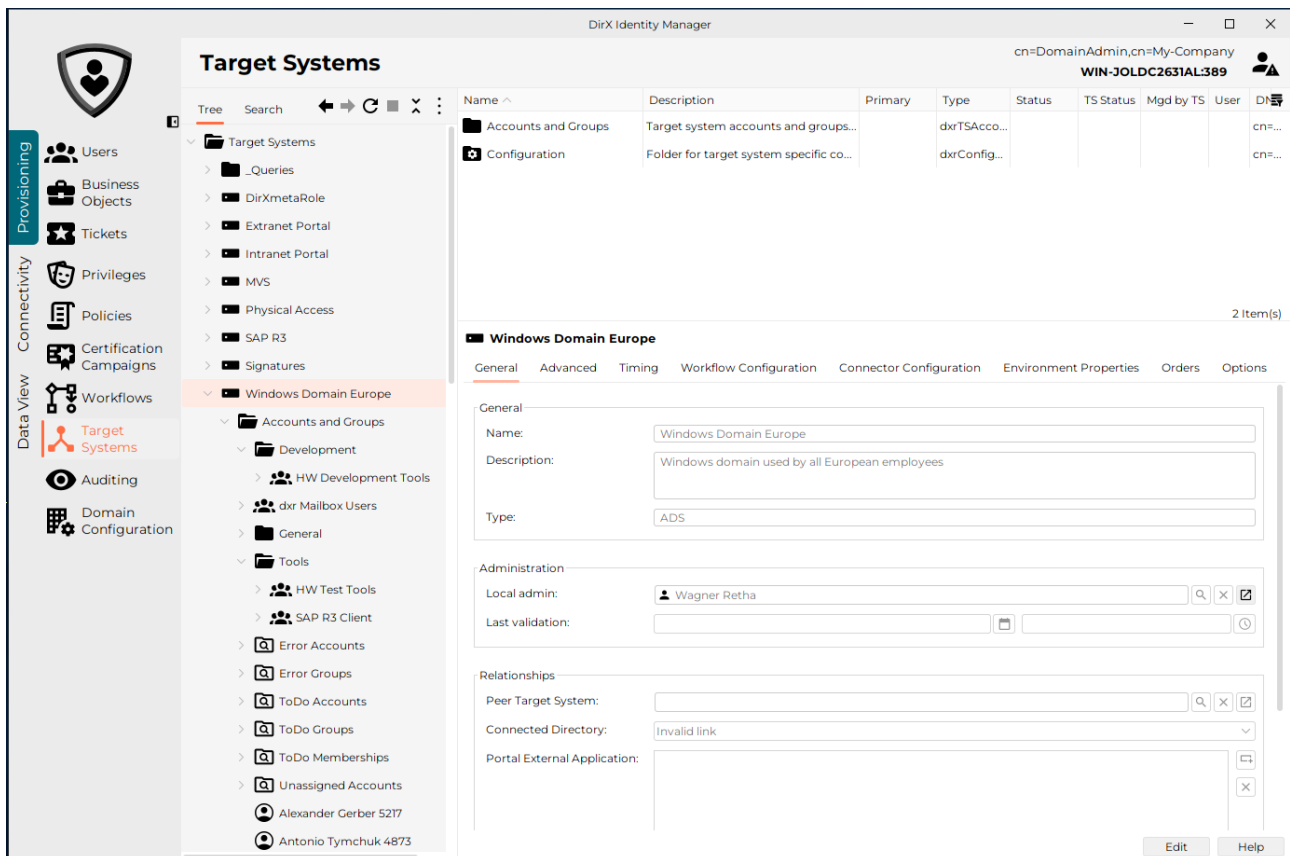
Figure 49. Managing Target Systems with DirX Identity Manager (Provisioning)
