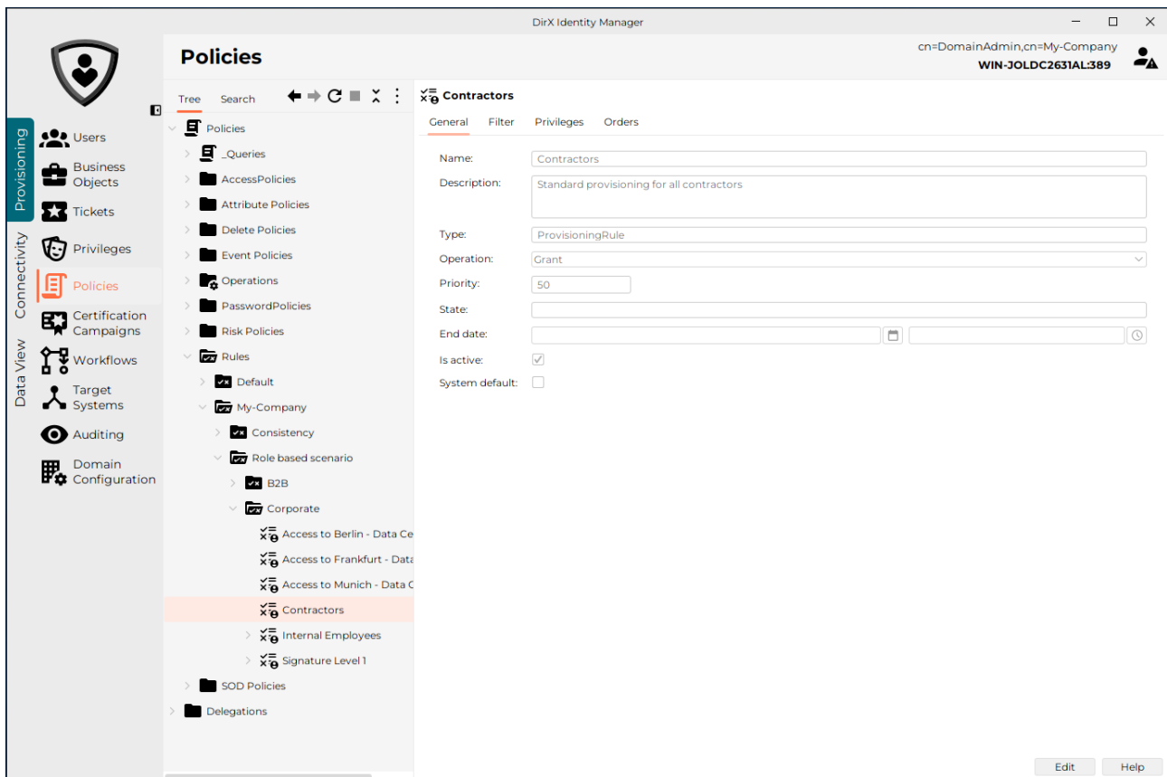
Figure 45. Viewing the Rules Subtree with DirX Identity Manager (Provisioning)
