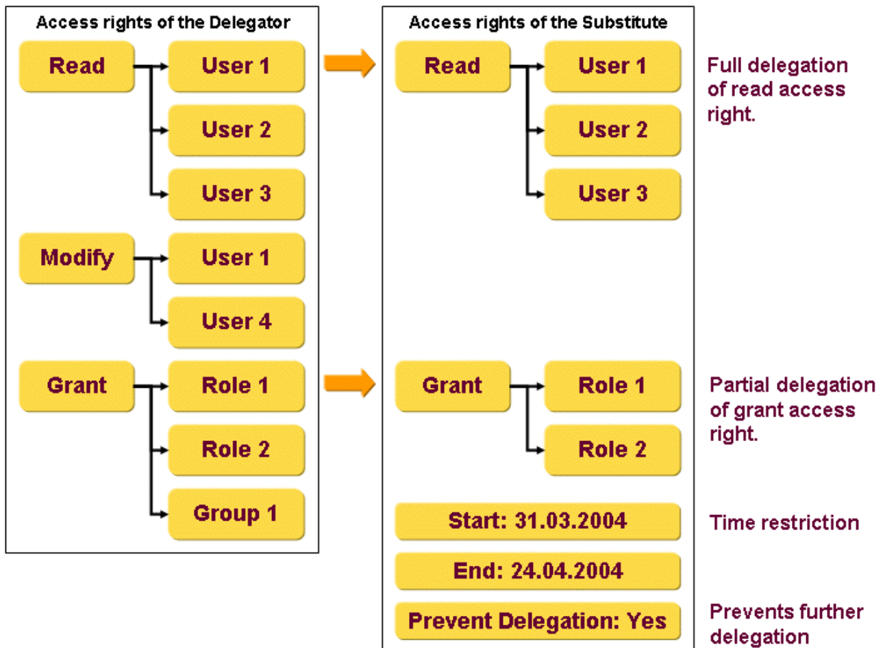
Figure 41. DirX Identity Provisioning Delegation Example
