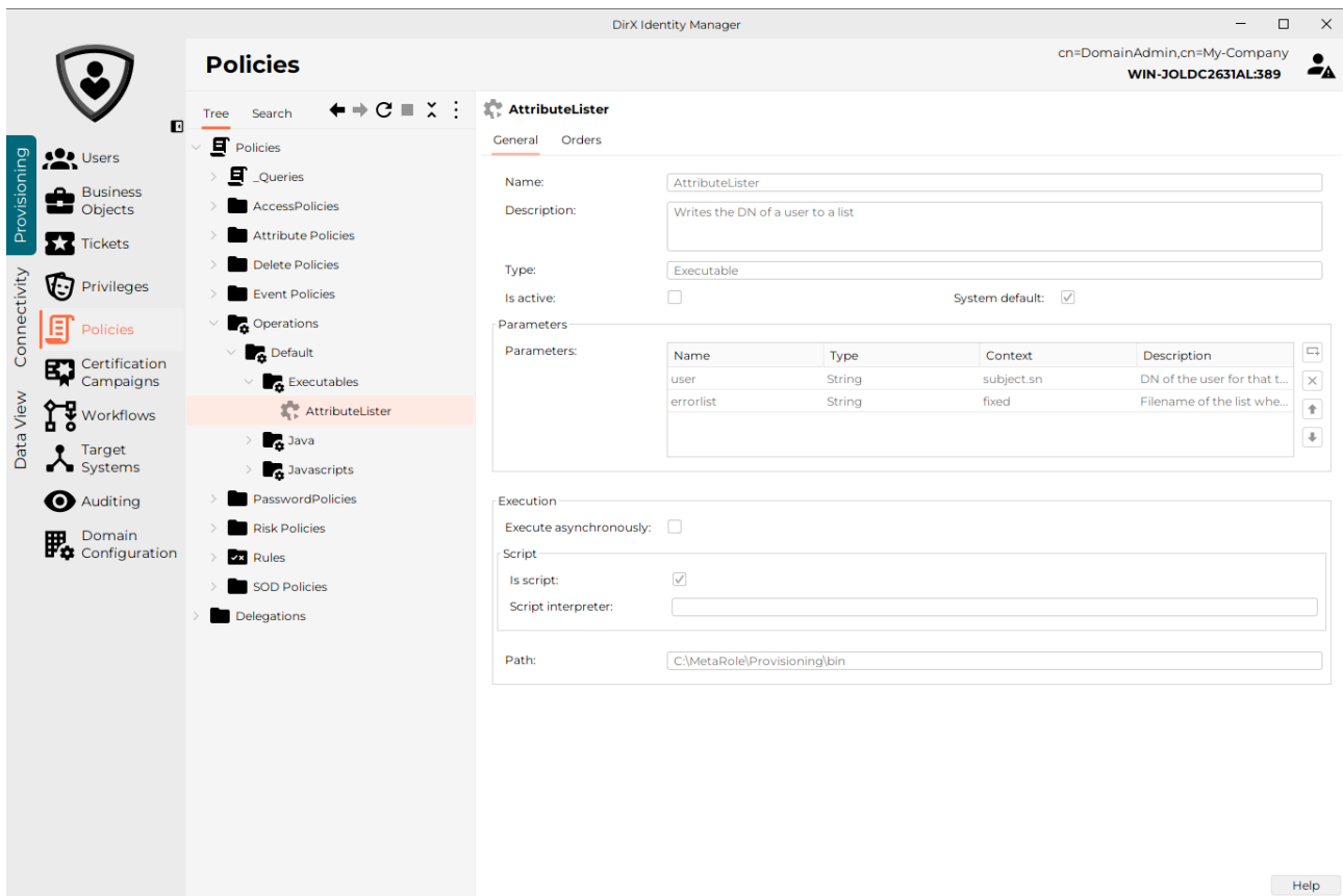
Figure 46. Viewing the Operations Structure with DirX Identity Manager (Provisioning)
