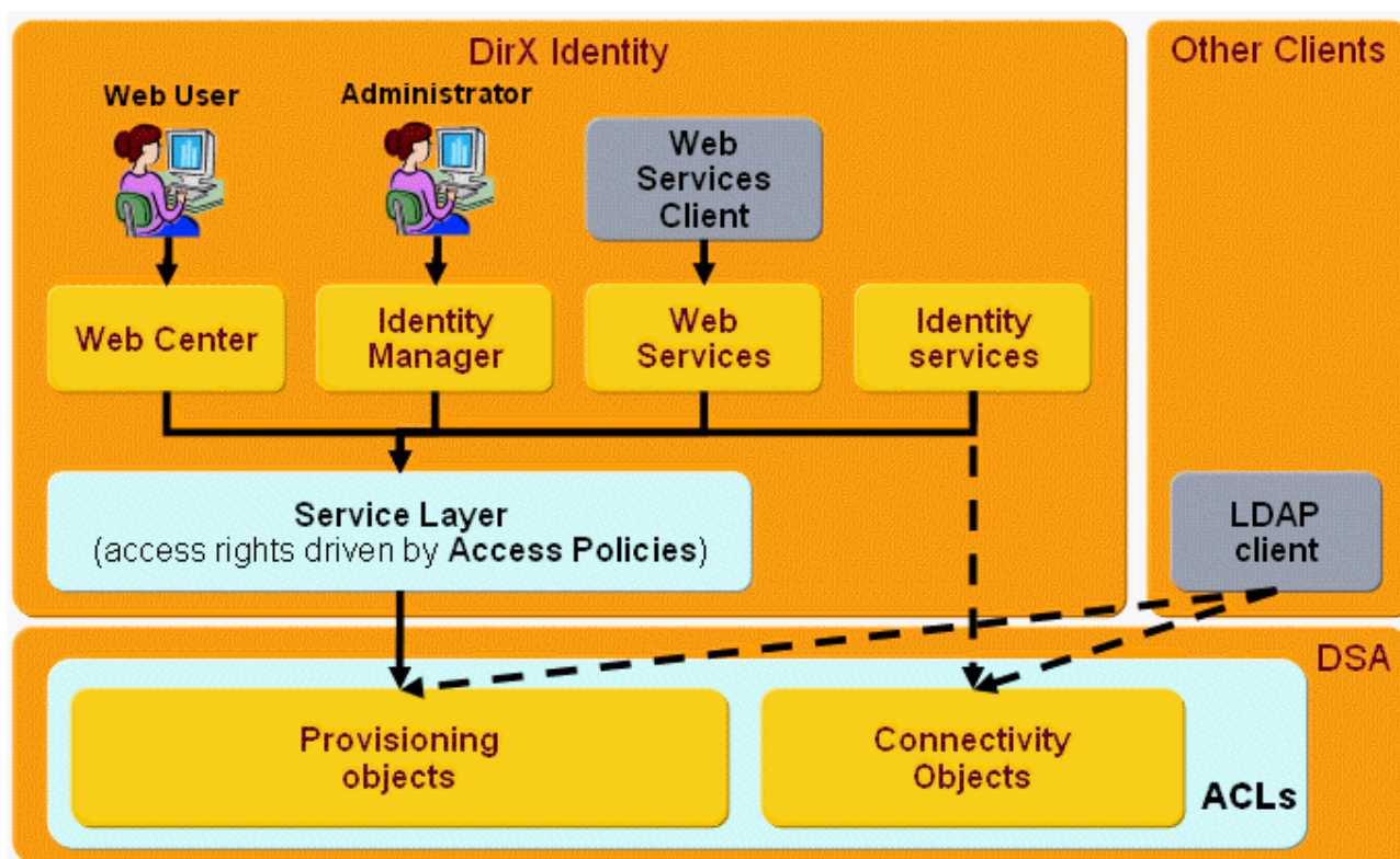
Figure 29. Access Policy Architecture
