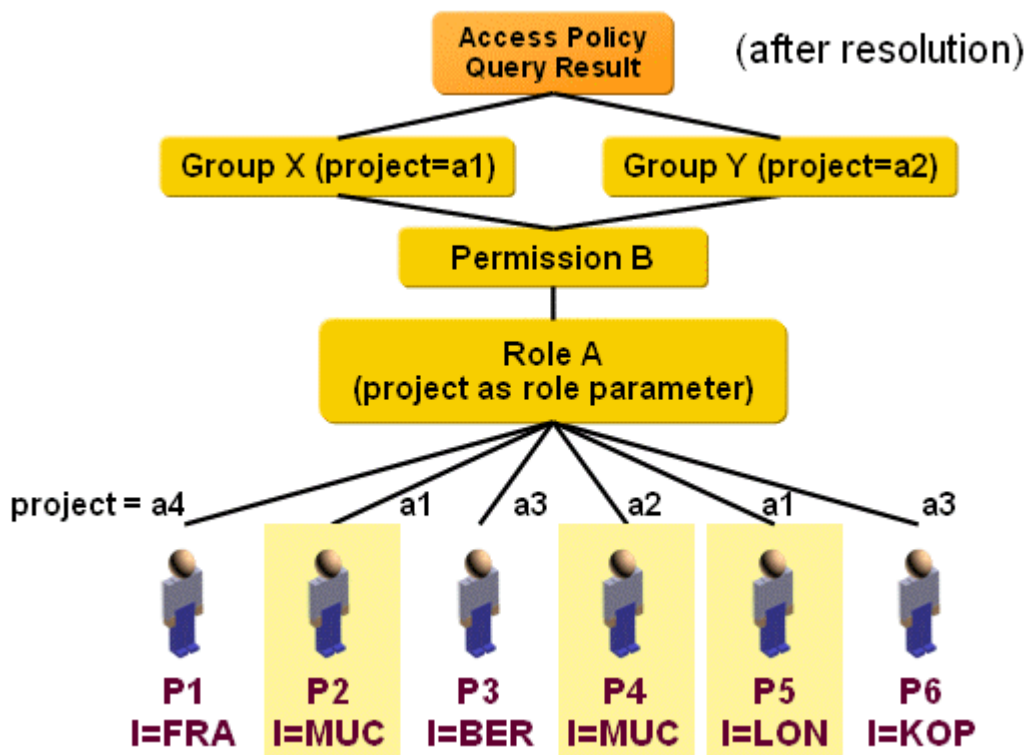
Figure 36. Selecting Subjects with Role Assignments and Role Parameters
