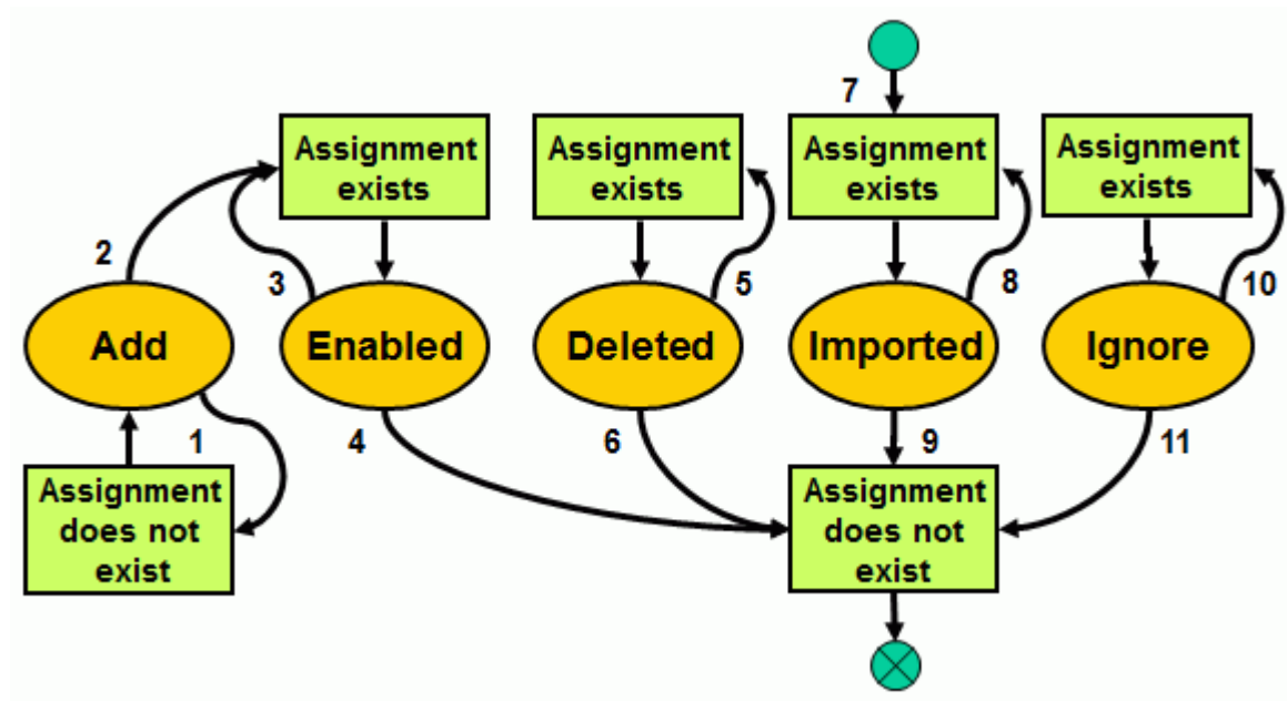
Figure 12. Assignment Import State Transitions (Account is Enabled)
