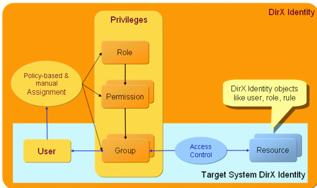
Figure 30. Access Control Model
