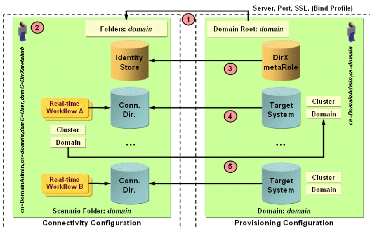
Figure 60. Relationship between Connectivity and Provisioning Domains
