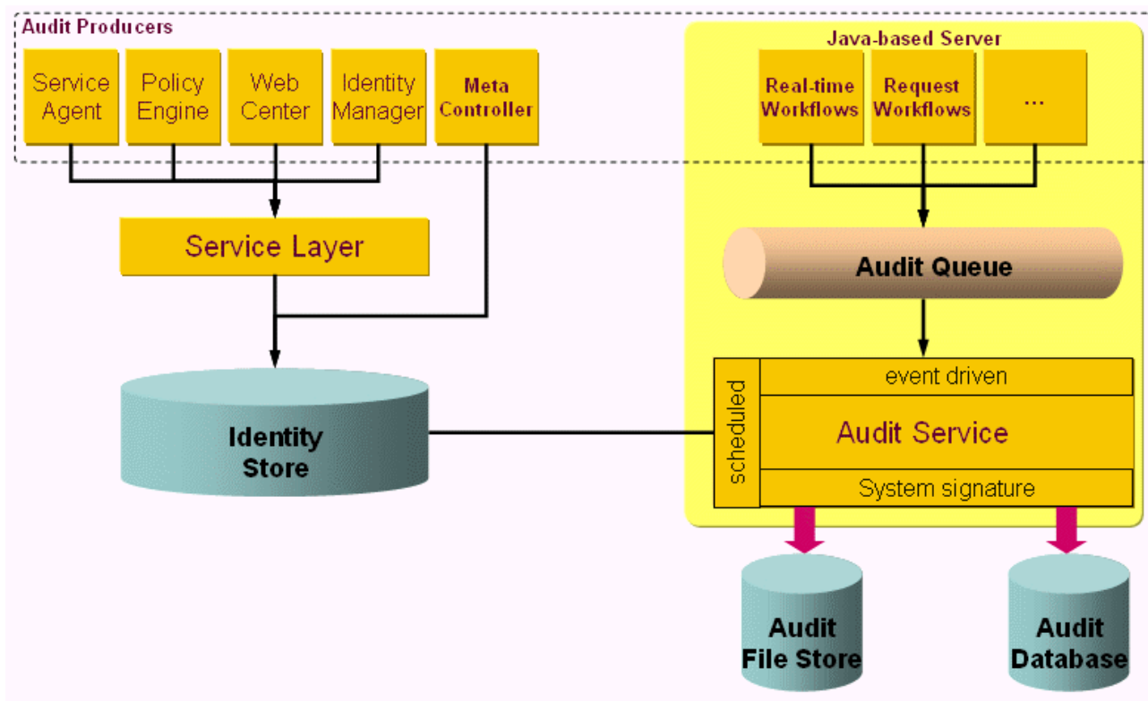
Figure 57. DirX Identity Audit Service
