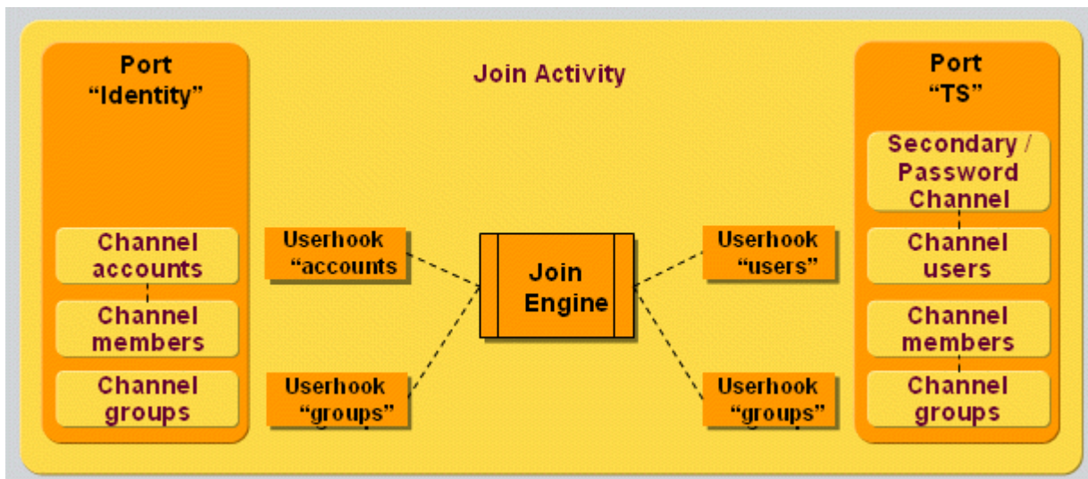
Figure 14. User Hooks
